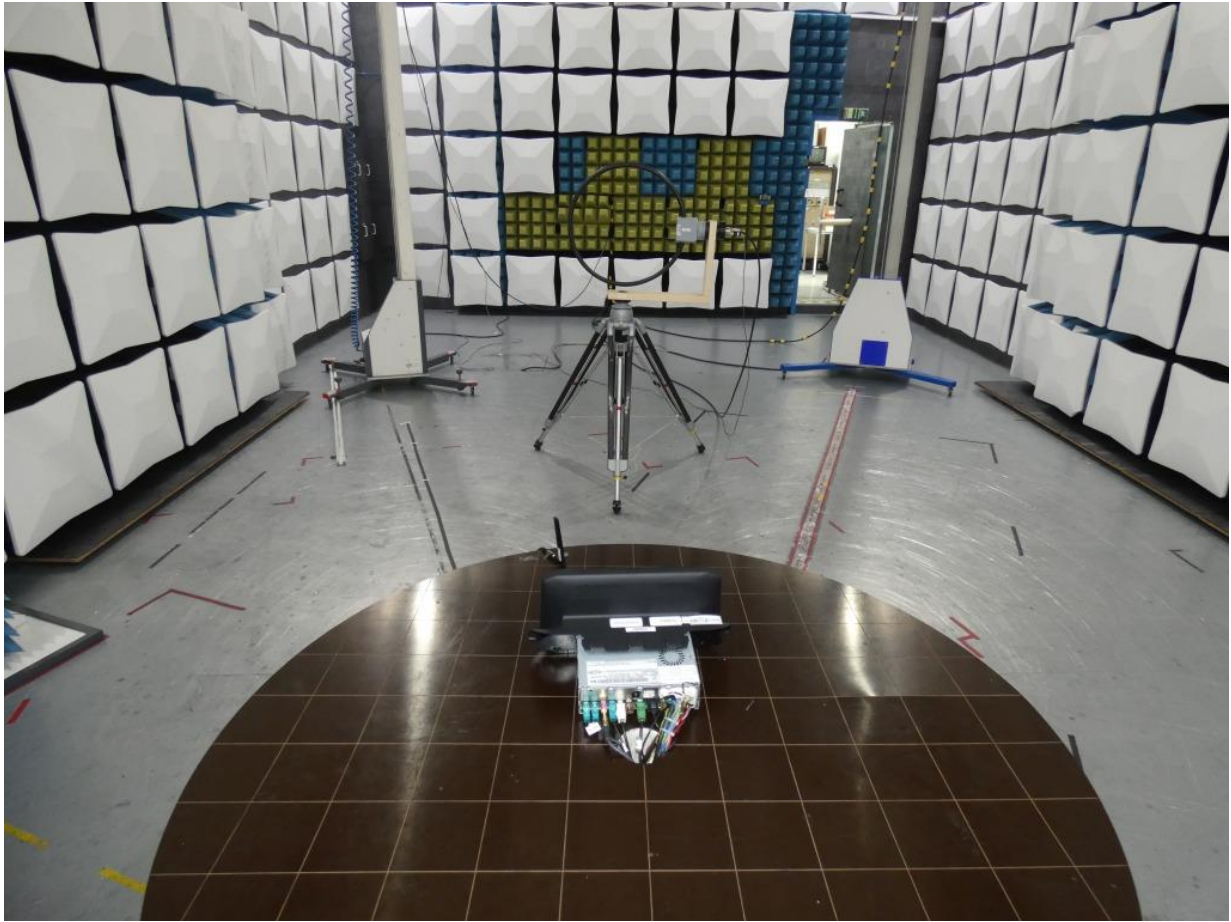
Photo 3: Test setup for radiated measurements ( 9 kHz - 30 MHz; FCC 15c247)
