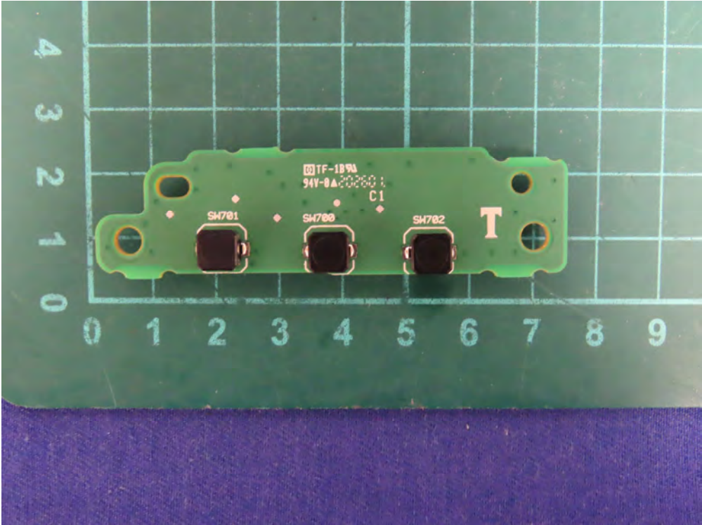
(98) EUT Photo (Monitor with WLAN Antenna 1)
