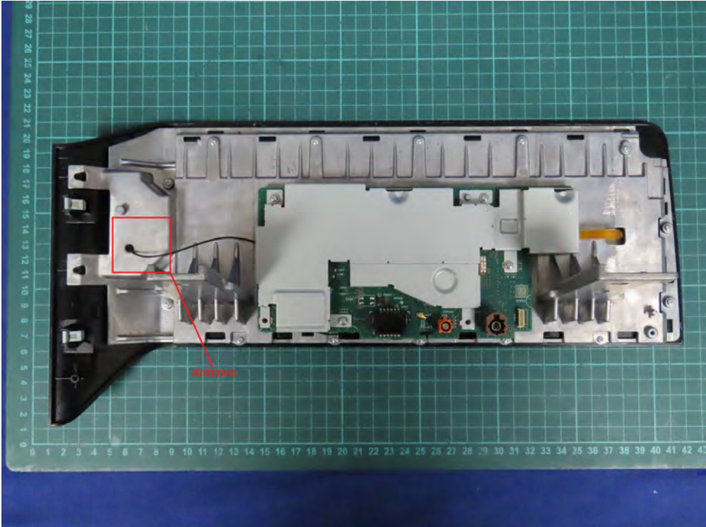
(111)EUT Photo (Monitor with WLAN Antenna 3)
