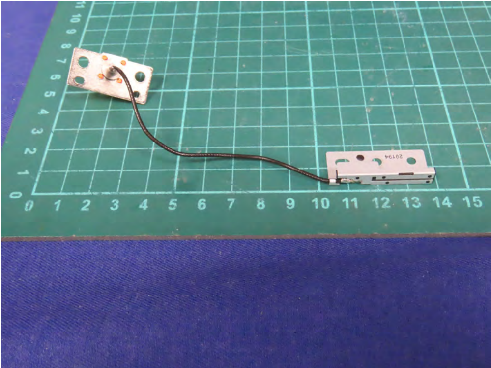
(86) EUT Photo (Monitor with WLAN Antenna 1)
