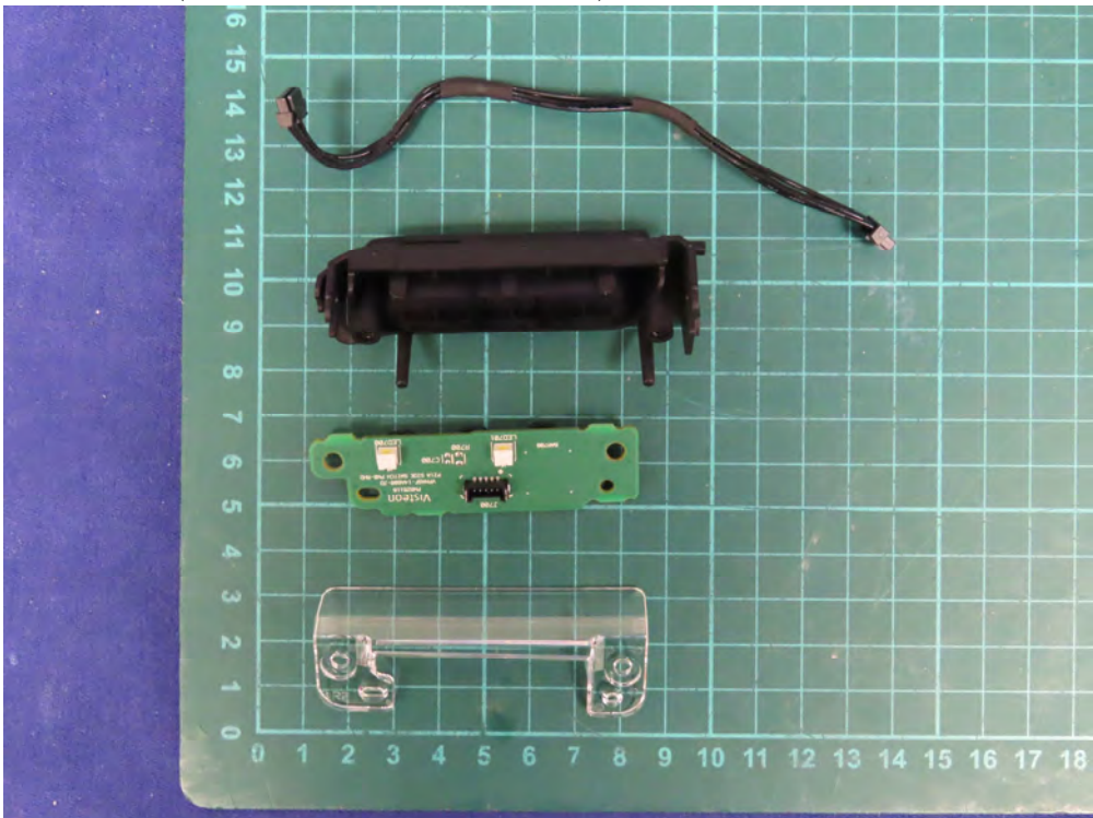
(96) EUT Photo (Monitor with WLAN Antenna 1)
