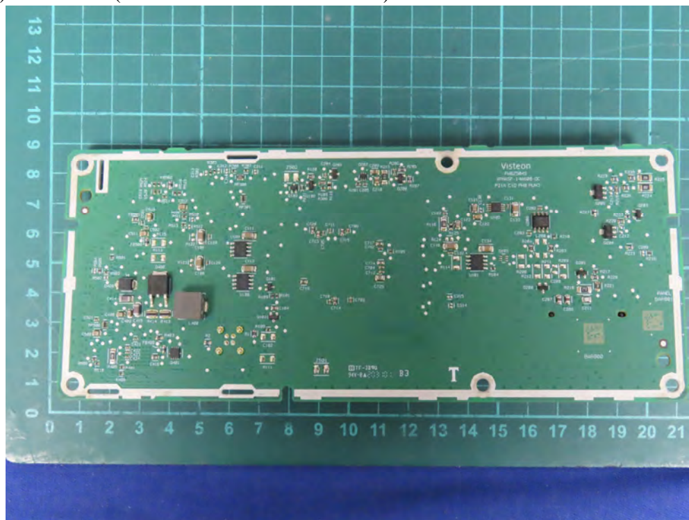
(81) EUT Photo (Monitor with WLAN Antenna 1)
