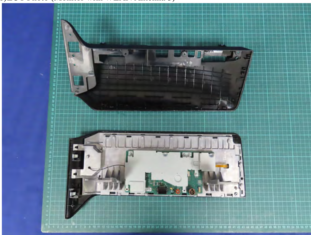
(110)EUT Photo (Monitor with WLAN Antenna 3)
