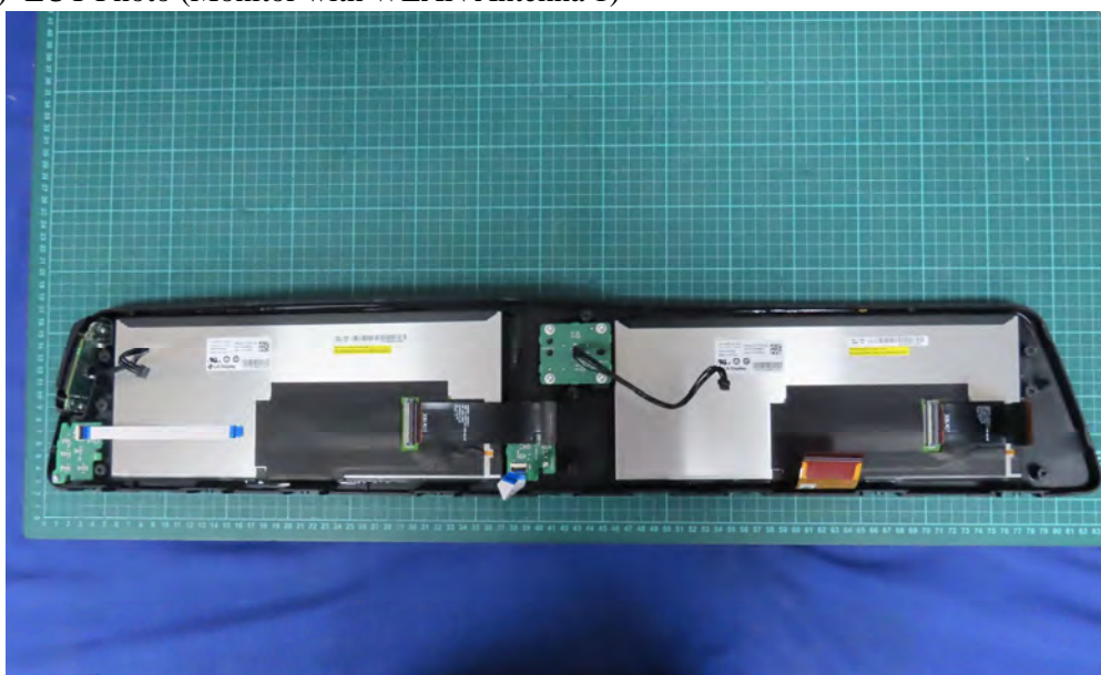
(88) EUT Photo (Monitor with WLAN Antenna 1)
