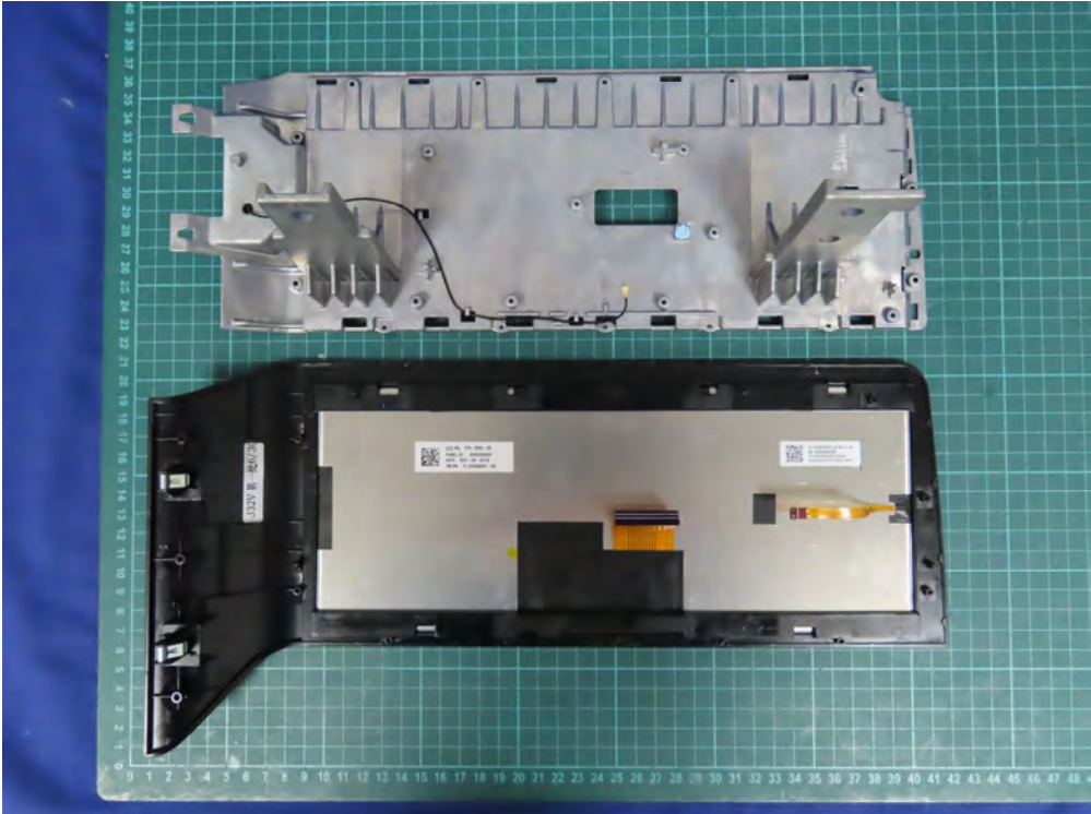
(115)EUT Photo (Monitor with WLAN Antenna 3)
