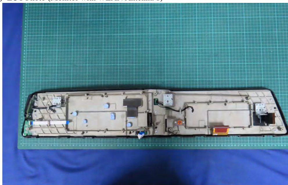
(82) EUT Photo (Monitor with WLAN Antenna 1)
