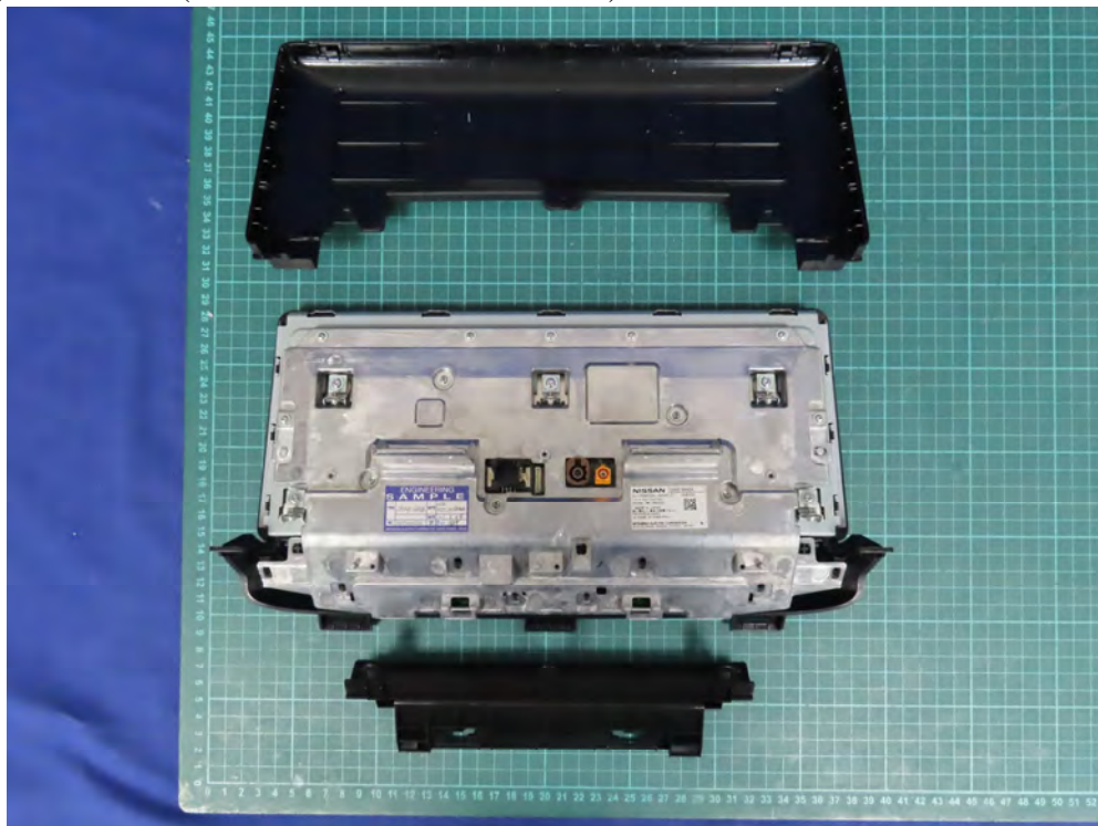
(99) EUT Photo (Monitor with WLAN Antenna 2)
