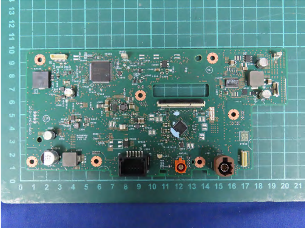
(113)EUT Photo (Monitor with WLAN Antenna 3)
