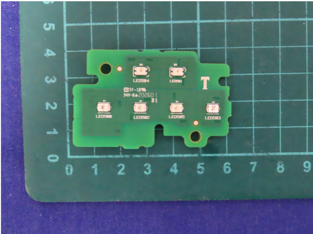
(95) EUT Photo (Monitor with WLAN Antenna 1)
