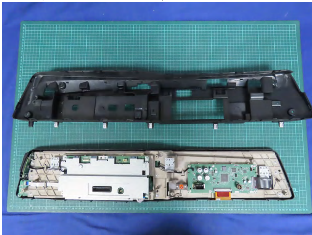
(75) EUT Photo (Monitor with WLAN Antenna 1)
