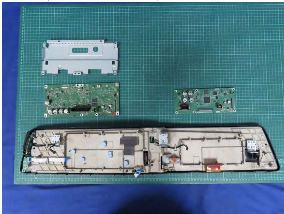
(77) EUT Photo (Monitor with WLAN Antenna 1)
