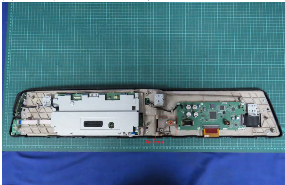
(76) EUT Photo (Monitor with WLAN Antenna 1)
