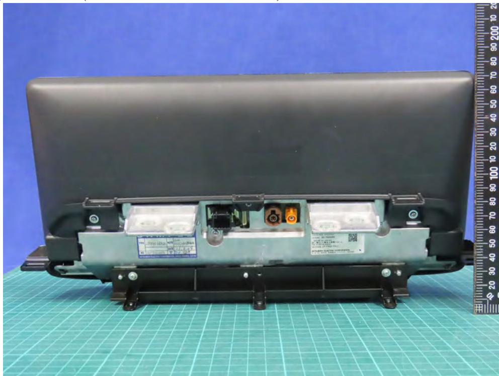
(19) EUT Photo (Monitor with WLAN Antenna 2)
