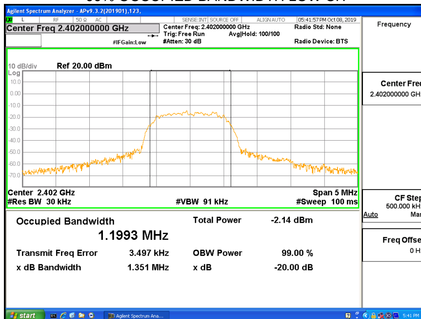
99% OCCUPIED BANDWIDTH LOW CH
