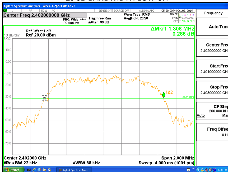
20 dB BANDWIDTH LOW CH
