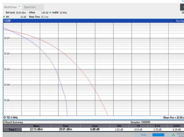
Band12-10MHz-QPSK-23095-50RB#0
