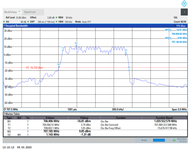
Band12-1.4MHz-QPSK-23095-6RB#0
