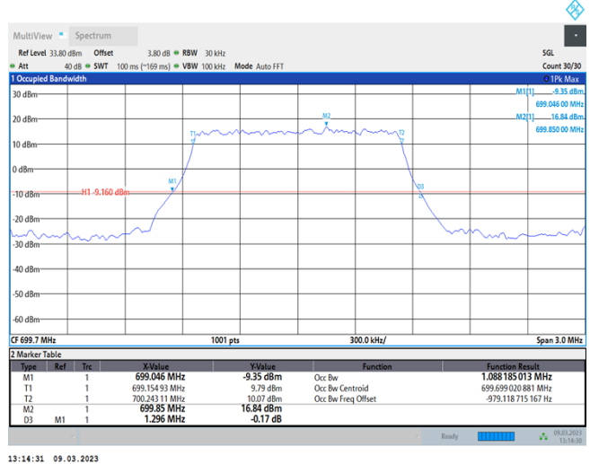
Band12-1.4MHz-QPSK-23095-6RB#0
