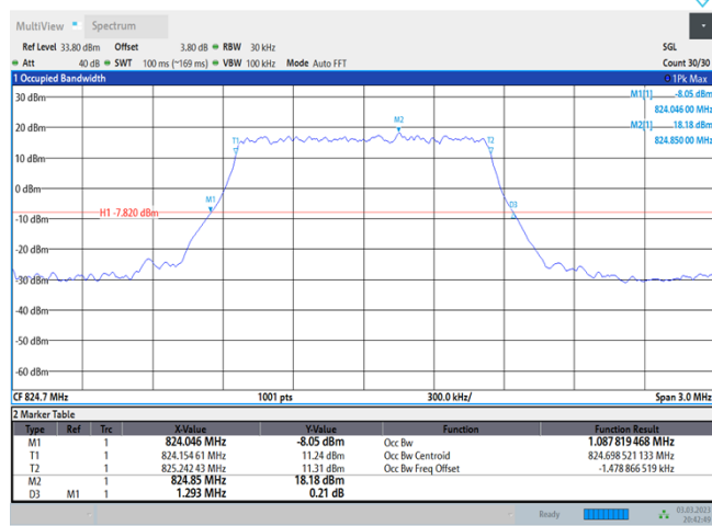
Band5-1.4MHz-QPSK-20525-6RB#0
