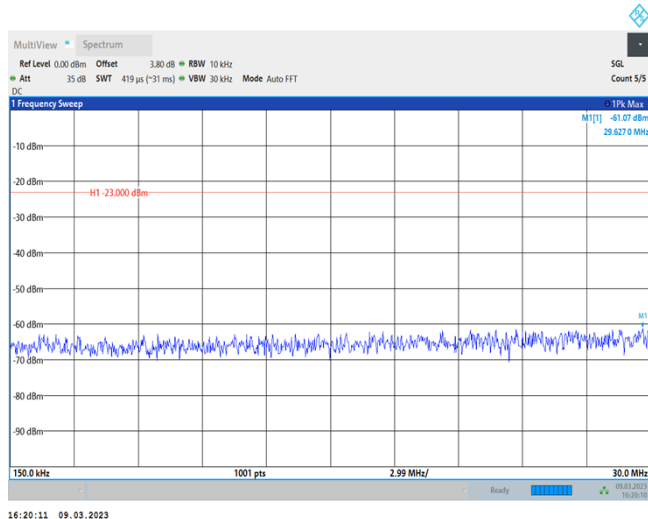
Band5-10MHz-QPSK-20450-1RB#0-Range2:0.15~30MHz
