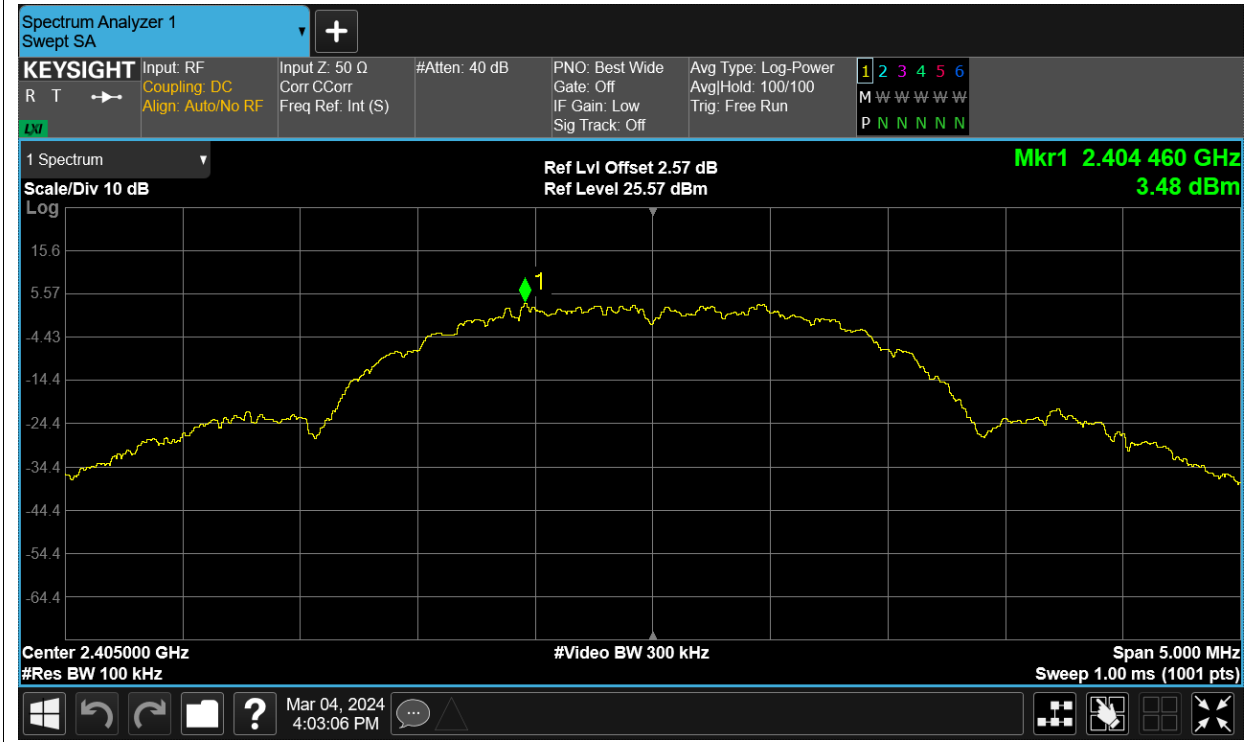
Band Edge NVNT ZIGBEE 2405MHz Ant1 Emission
