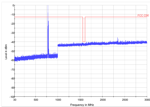
LTE Band 135MHzCH-High 30MHz~3GHz
