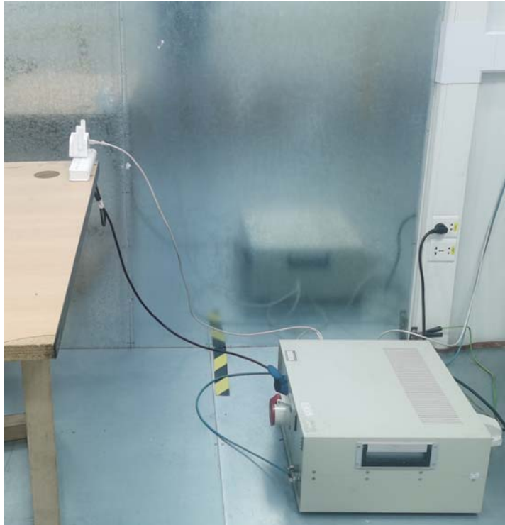
Conducted Emission Test Setup:
