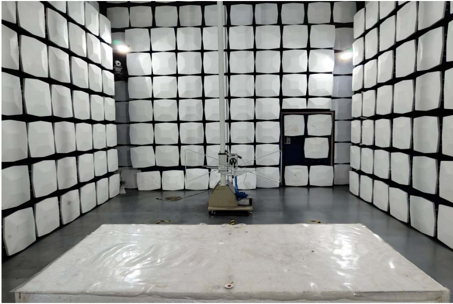
Radiated Emission Test Setup:
