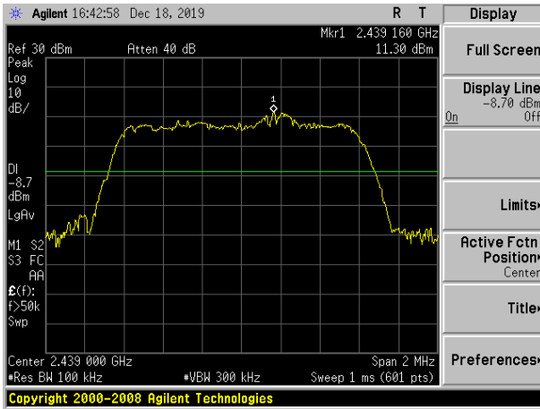
QPSK on channel 18
