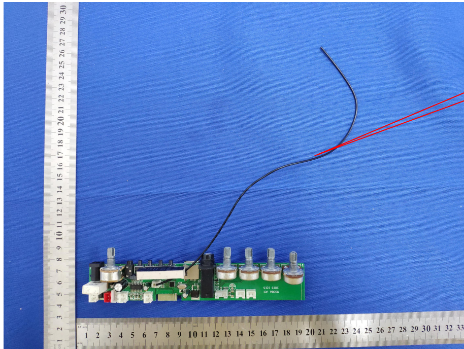
FM Antenna
