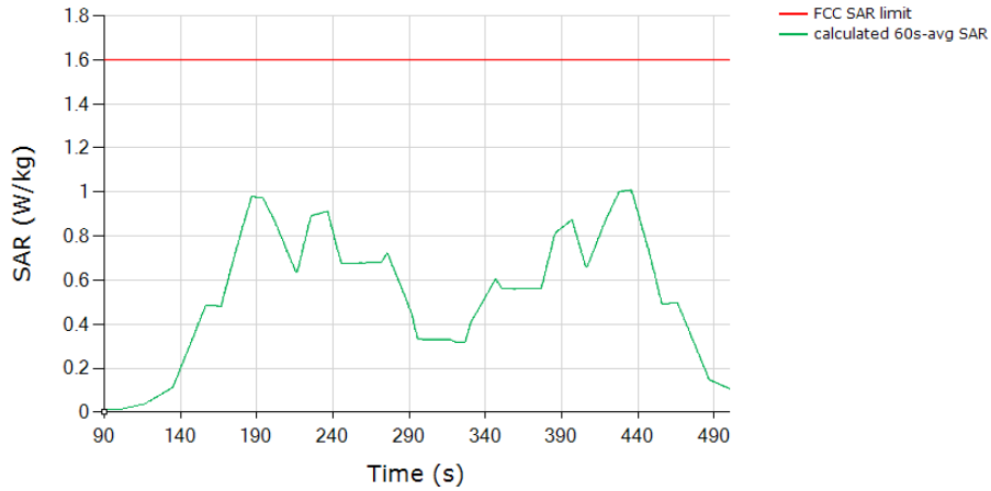
SAR (Test Sequence 2) Tech: NRSUB6SA, Band 77
