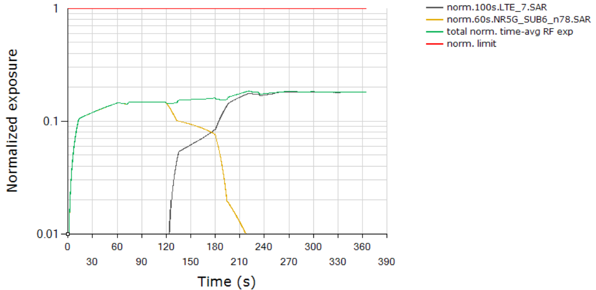
Total Normalized Time-averaged RF Exposure Tech: LTE, Band 7 / Tech: NR5G SUB6, Band n78
