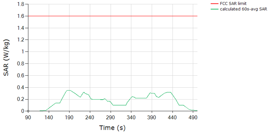
SAR (Test Sequence 2) Tech: NRSUB6SA, Band 78
