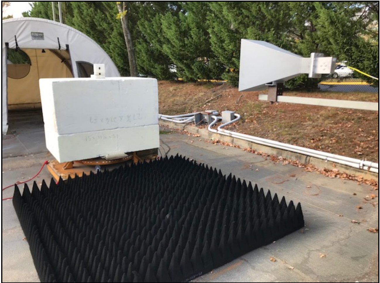
Photograph 4: Radiated Emissions Testing – Back View (Spurious Emissions, >1 GHz)
