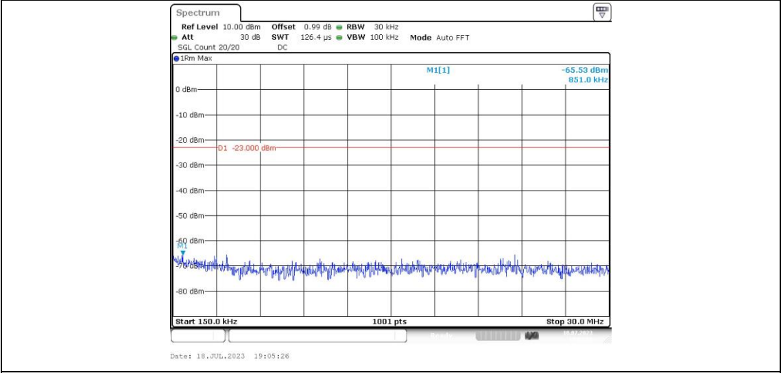
Band2-9400-2-0.15~30MHz
