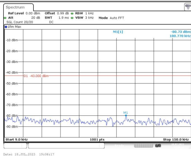
Band2-9538-2-0.009~0.15MHz
