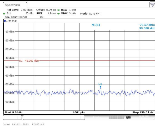
Band2-9538-2-0.009~0.15MHz
