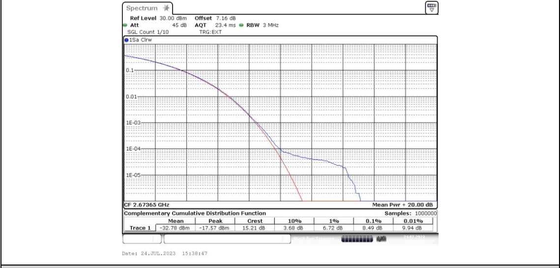
41-41-20MHz-15MHz-16QAM-16QAM-39750-39921-100RB#0-75RB#0
