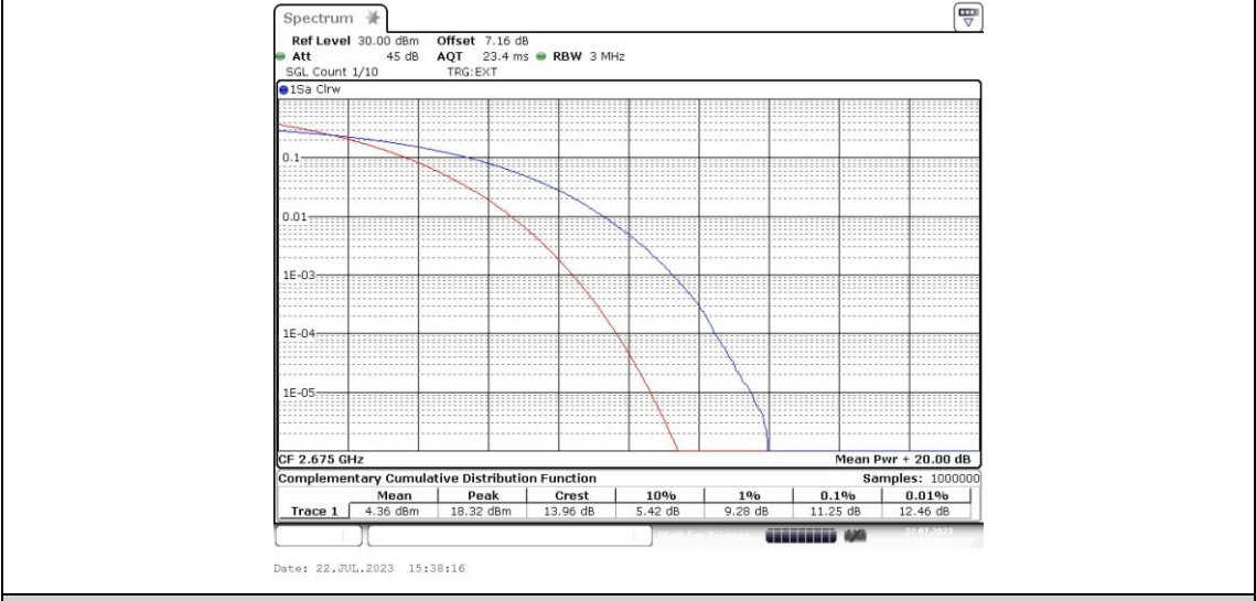
41-41-15MHz-20MHz-QPSK-QPSK-39728-39899-75RB#0-100RB#0
