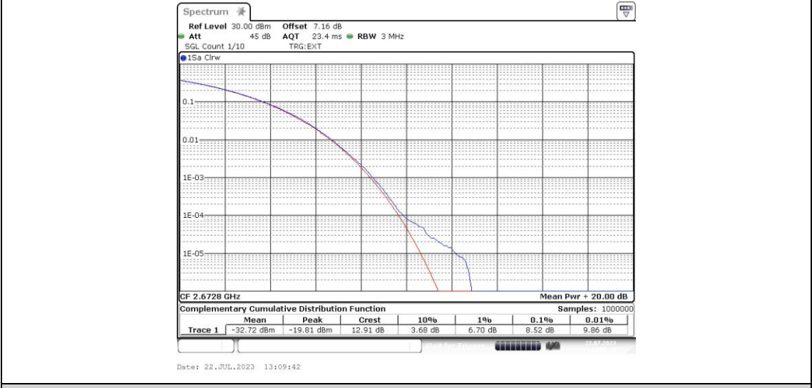
41-41-10MHz-20MHz-16QAM-16QAM-39705-39849-50RB#0-100RB#0
