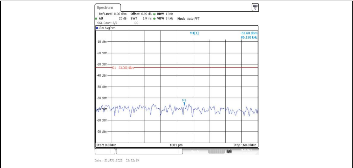
Band25-15MHz-16QAM-26615-1RB#0-Range1:0.009~0.15MHz-PASS
