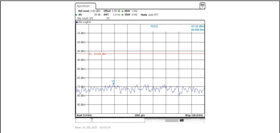
Band25-20MHz-QPSK-26365-1RB#0-Range1:0.009~0.15MHz-PASS
