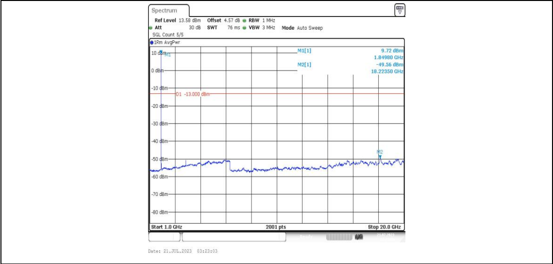
Band25-20MHz-16QAM-26140-1RB#0-Range4:1000~20000MHz-PASS
