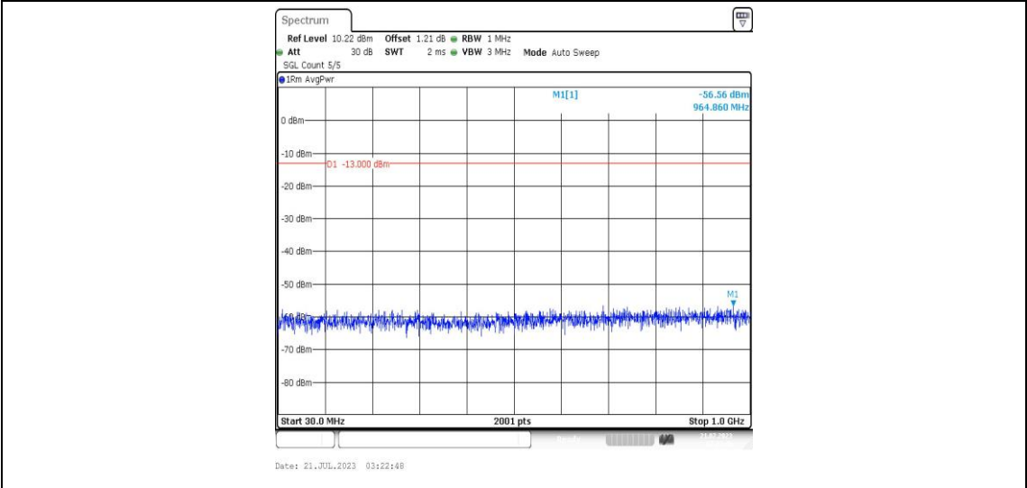
Band25-20MHz-16QAM-26140-1RB#0-Range3:30~1000MHz-PASS
