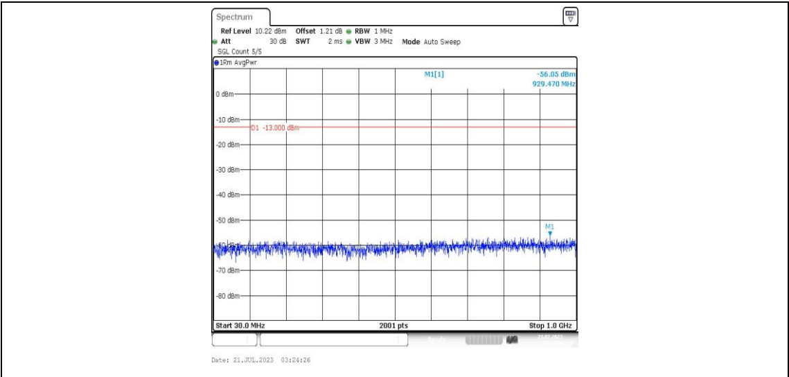
Band25-20MHz-16QAM-26365-1RB#0-Range3:30~1000MHz-PASS
