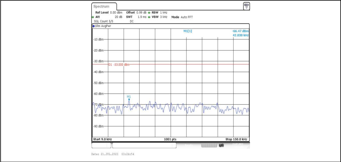
Band25-20MHz-QPSK-26590-1RB#0-Range1:0.009~0.15MHz-PASS
