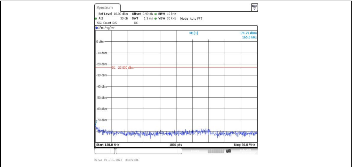
Band25-20MHz-16QAM-26140-1RB#0-Range2:0.15~30MHz-PASS
