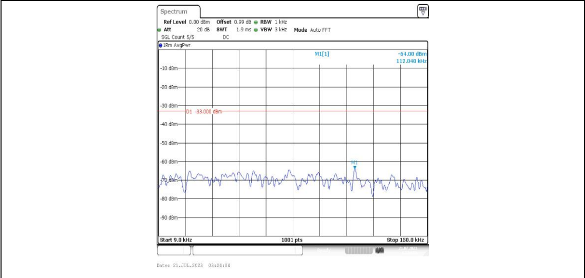
Band25-20MHz-16QAM-26365-1RB#0-Range1:0.009~0.15MHz-PASS
