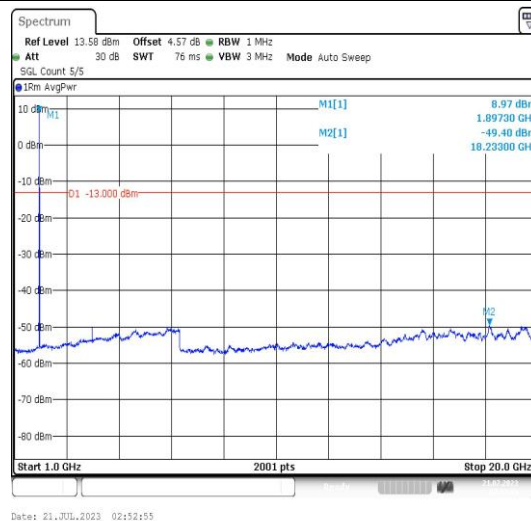
Band25-15MHz-16QAM-26615-1RB#0-Range4:1000~20000MHz-PASS
