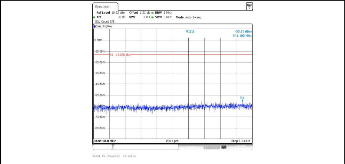
Band25-20MHz-16QAM-26590-1RB#0-Range3:30~1000MHz-PASS
