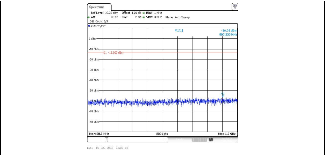
Band25-20MHz-QPSK-26140-1RB#0-Range3:30~1000MHz-PASS
