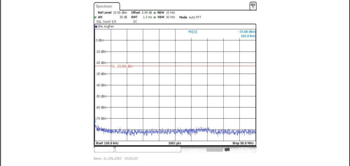
Band25-15MHz-16QAM-26615-1RB#0-Range2:0.15~30MHz-PASS
