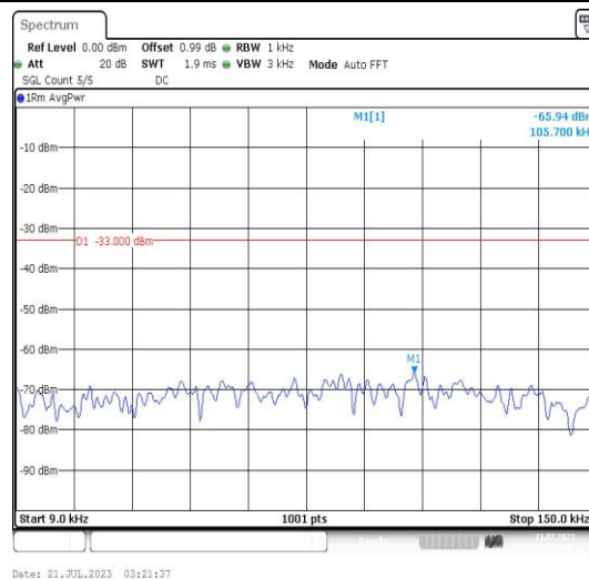
Band25-20MHz-QPSK-26140-1RB#0-Range1:0.009~0.15MHz-PASS
