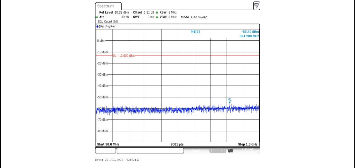
Band25-15MHz-16QAM-26615-1RB#0-Range3:30~1000MHz-PASS
