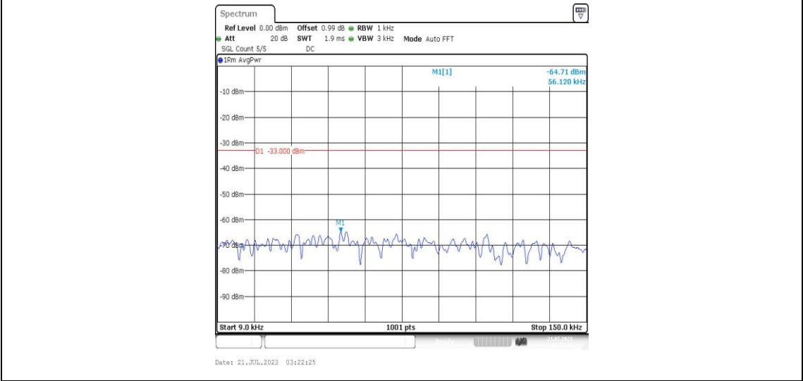
Band25-20MHz-16QAM-26140-1RB#0-Range1:0.009~0.15MHz-PASS
