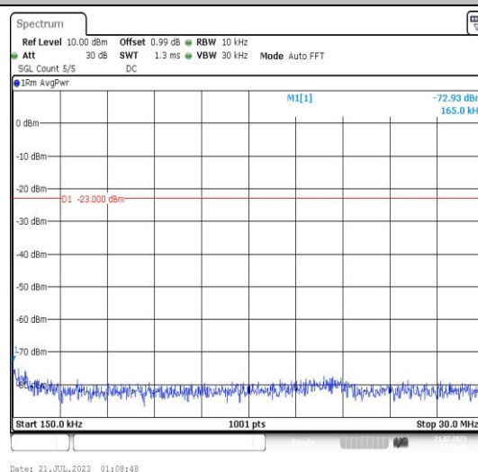
Band25-3MHz-QPSK-26055-1RB#0-Range2:0.15~30MHz-PASS
