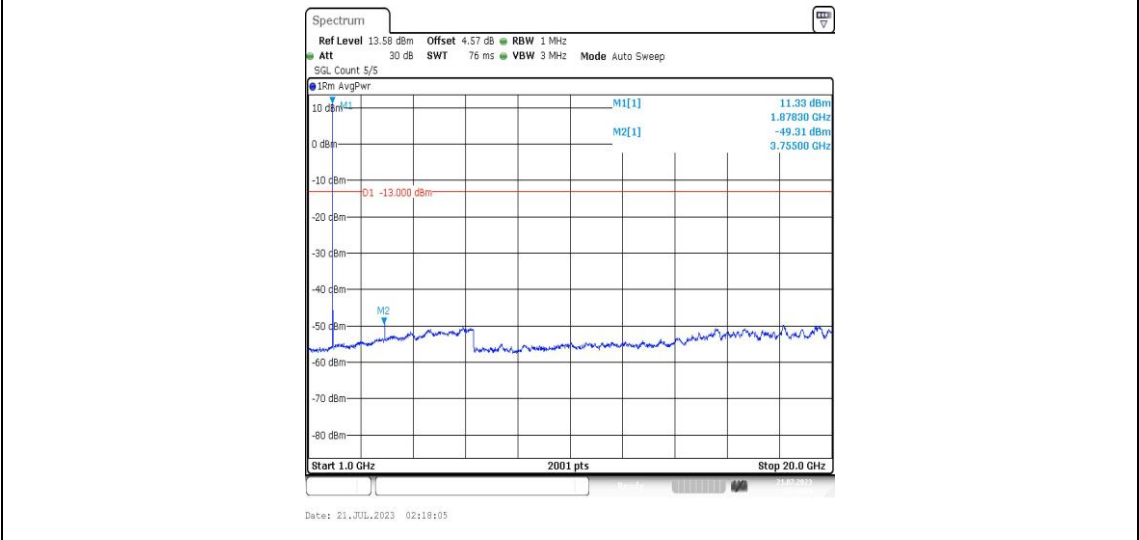
Band25-10MHz-16QAM-26365-1RB#0-Range4:1000~20000MHz-PASS
