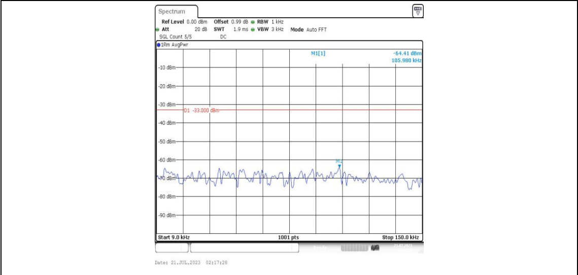
Band25-10MHz-16QAM-26365-1RB#0-Range1:0.009~0.15MHz-PASS
