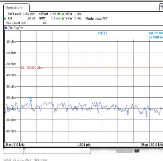
Band25-10MHz-16QAM-26090-1RB#0-Range1:0.009~0.15MHz-PASS
