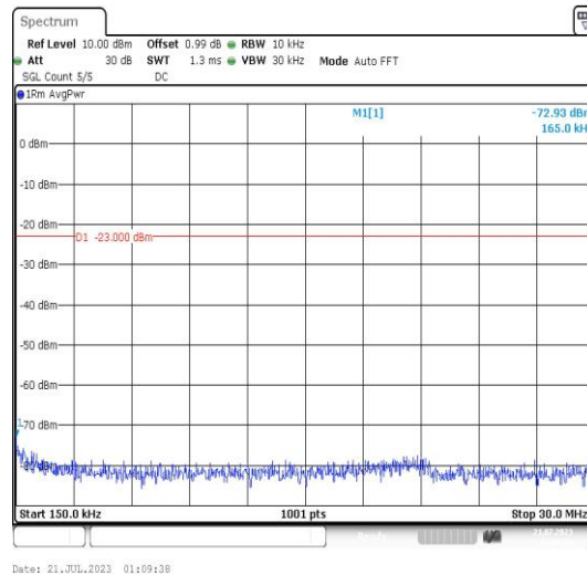
Band25-3MHz-16QAM-26055-1RB#0-Range2:0.15~30MHz-PASS
