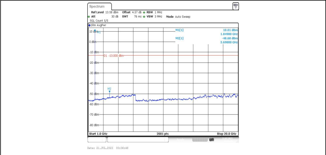
Band25-1.4MHz-QPSK-26047-1RB#0-Range4:1000~20000MHz-PASS
