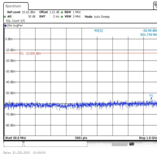
Band25-3MHz-16QAM-26055-1RB#0-Range3:30~1000MHz-PASS
