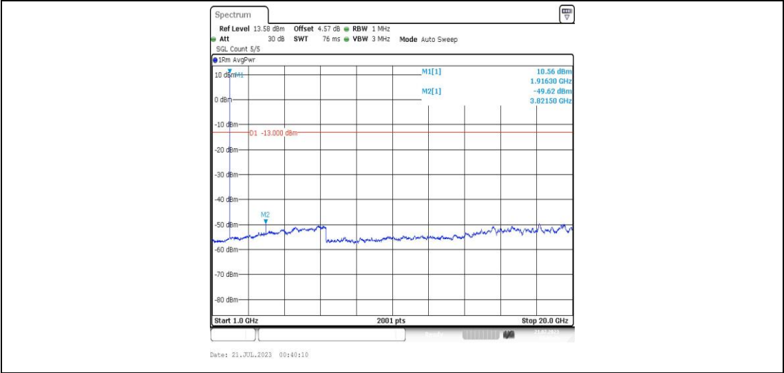
Band25-1.4MHz-QPSK-26683-1RB#0-Range4:1000~20000MHz-PASS
