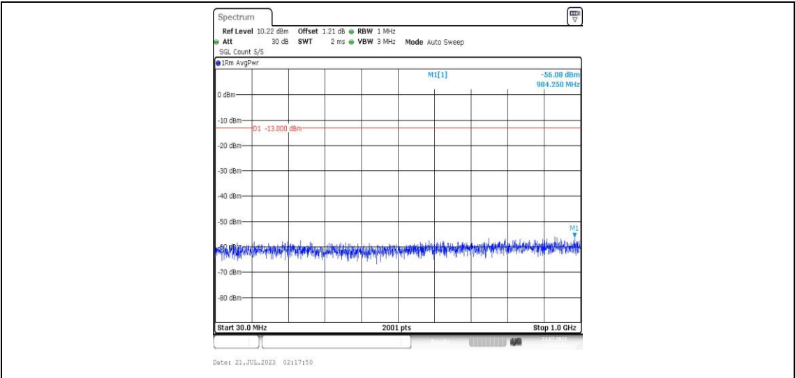
Band25-10MHz-16QAM-26365-1RB#0-Range3:30~1000MHz-PASS
