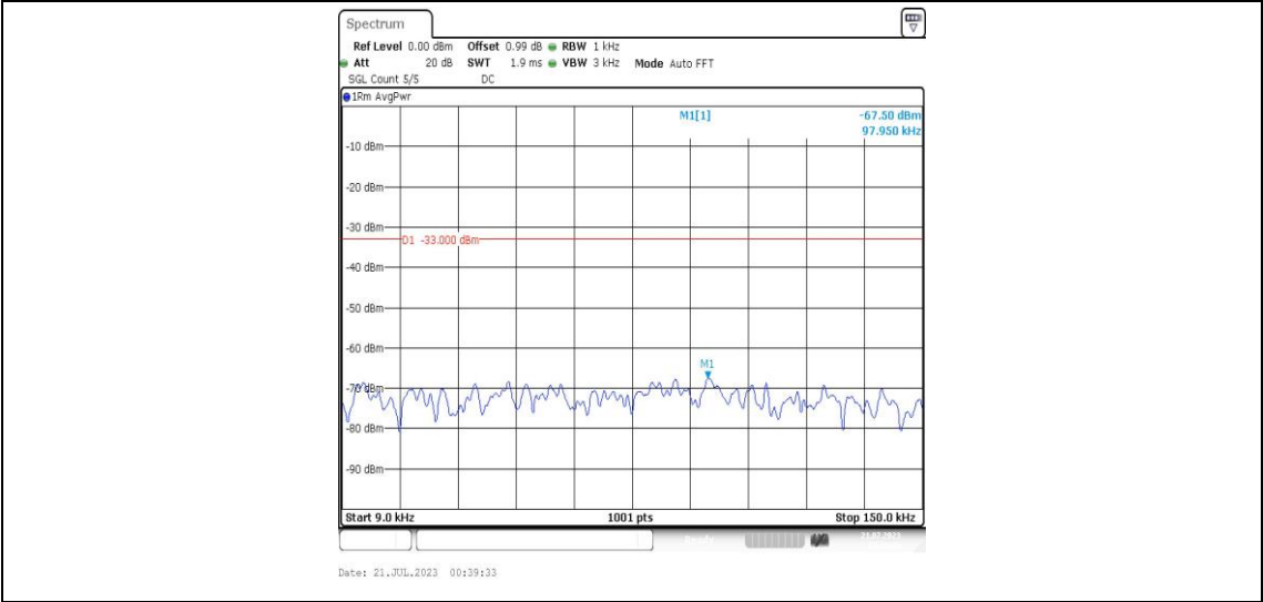
Band25-1.4MHz-QPSK-26683-1RB#0-Range1:0.009~0.15MHz-PASS
