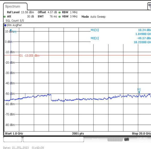
Band25-5MHz-QPSK-26065-1RB#0-Range4:1000~20000MHz-PASS
