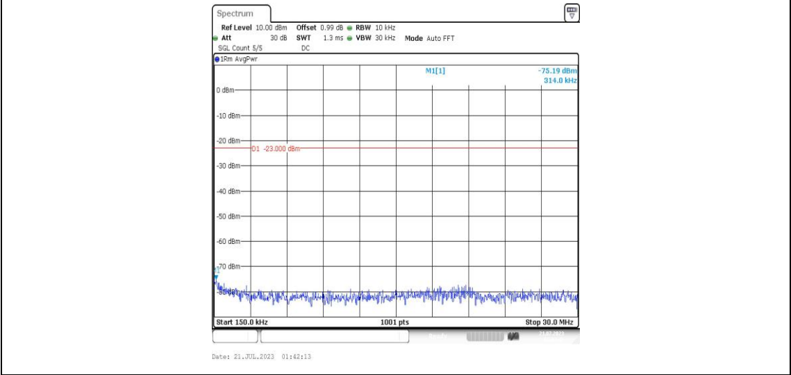
Band25-5MHz-QPSK-26065-1RB#0-Range2:0.15~30MHz-PASS
