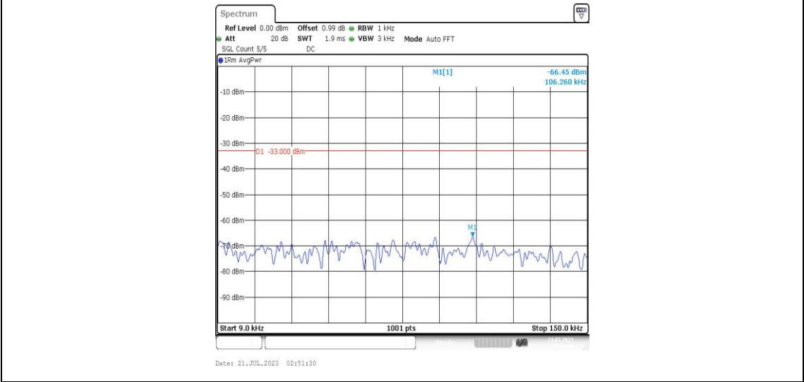
Band25-15MHz-QPSK-26615-1RB#0-Range1:0.009~0.15MHz-PASS
