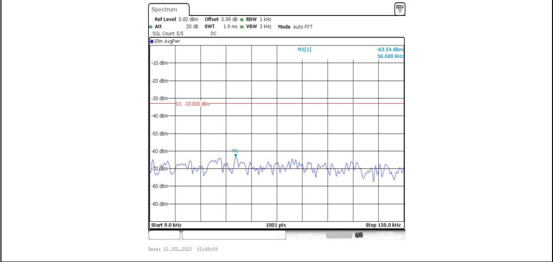
Band25-15MHz-16QAM-26115-1RB#0-Range1:0.009~0.15MHz-PASS
