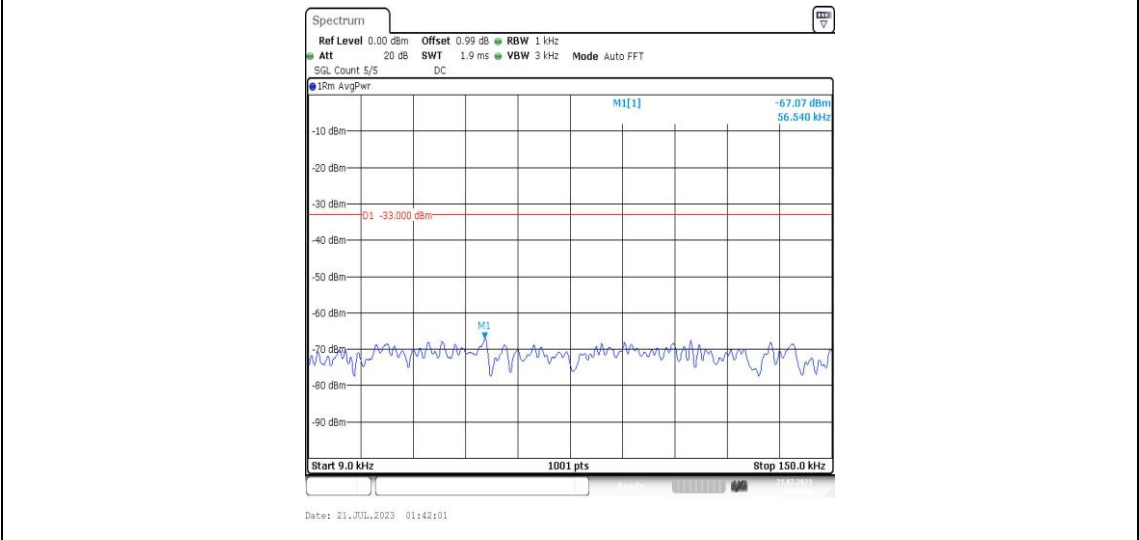
Band25-5MHz-QPSK-26065-1RB#0-Range1:0.009~0.15MHz-PASS
