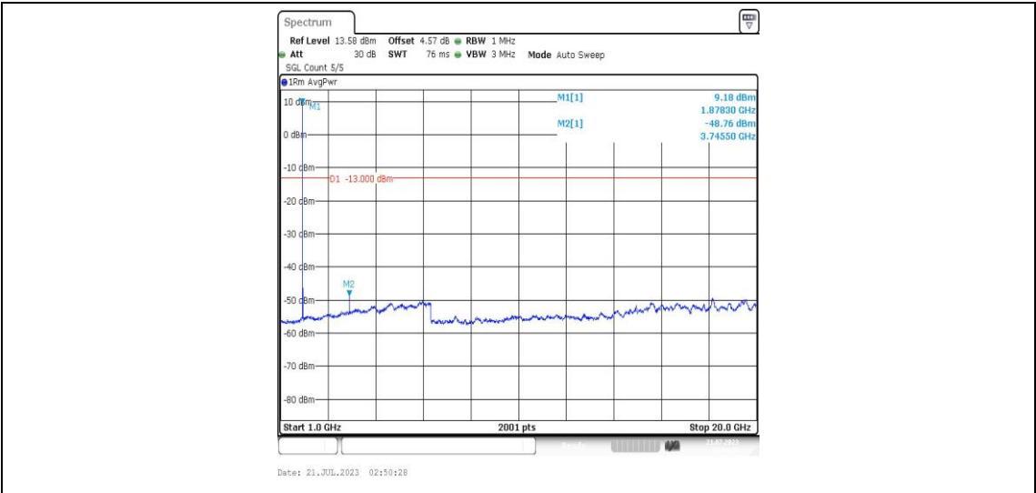
Band25-15MHz-QPSK-26365-1RB#0-Range4:1000~20000MHz-PASS
