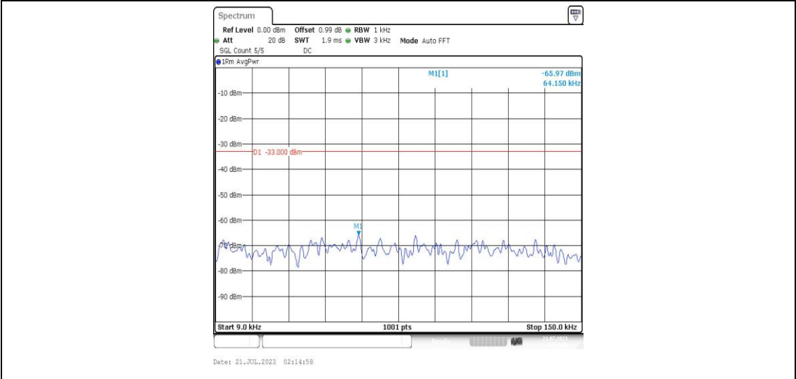
Band25-10MHz-QPSK-26090-1RB#0-Range1:0.009~0.15MHz-PASS
