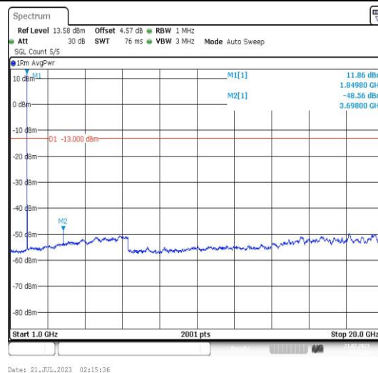
Band25-10MHz-QPSK-26090-1RB#0-Range4:1000~20000MHz-PASS
