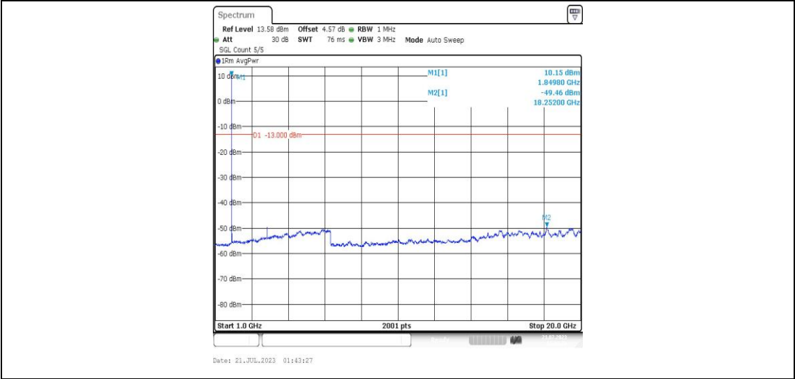
Band25-5MHz-16QAM-26065-1RB#0-Range4:1000~20000MHz-PASS
