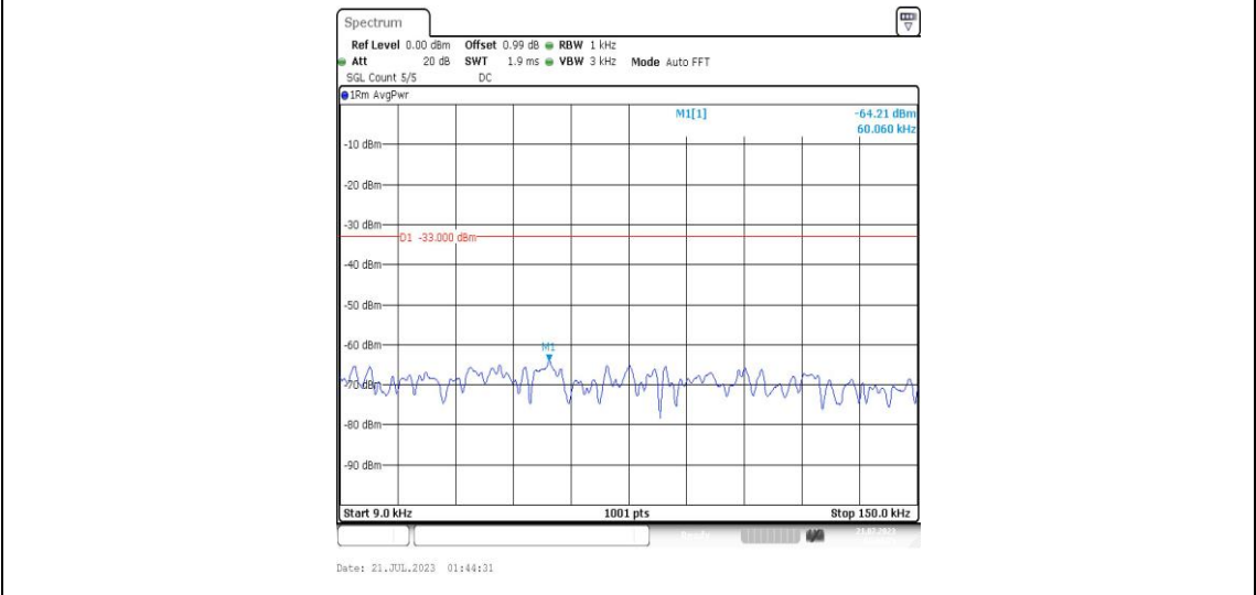
Band25-5MHz-16QAM-26365-1RB#0-Range1:0.009~0.15MHz-PASS
