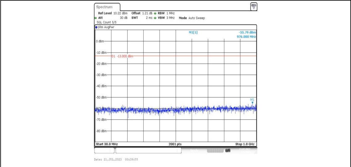
Band25-1.4MHz-QPSK-26683-1RB#0-Range3:30~1000MHz-PASS
