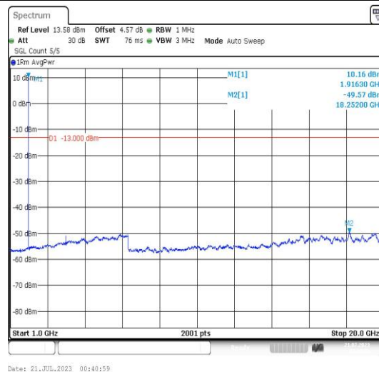
Band25-1.4MHz-16QAM-26683-1RB#0-Range4:1000~20000MHz-PASS
