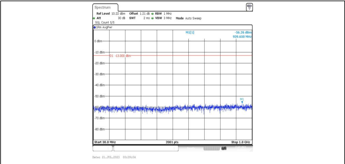
Band25-1.4MHz-16QAM-26365-1RB#0-Range3:30~1000MHz-PASS
