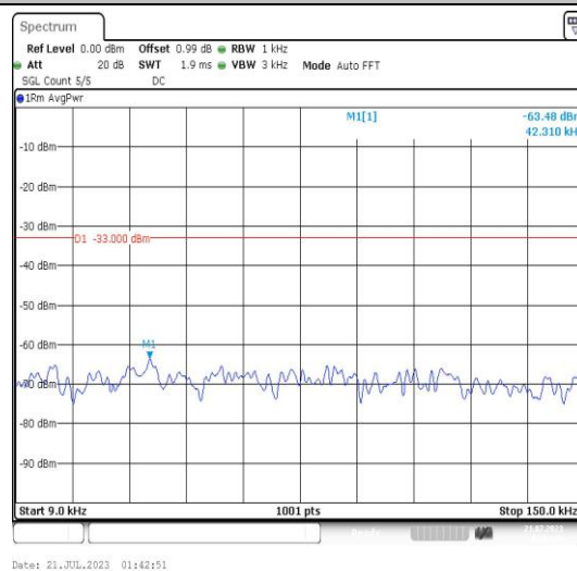
Band25-5MHz-16QAM-26065-1RB#0-Range1:0.009~0.15MHz-PASS
