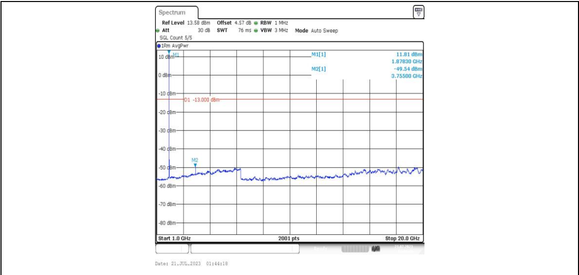
Band25-5MHz-QPSK-26365-1RB#0-Range4:1000~20000MHz-PASS
