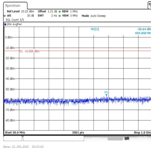
Band25-10MHz-QPSK-26090-1RB#0-Range3:30~1000MHz-PASS
