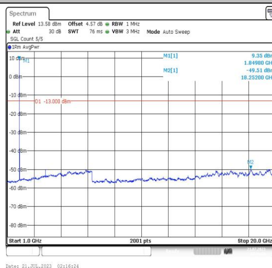
Band25-10MHz-16QAM-26090-1RB#0-Range4:1000~20000MHz-PASS
