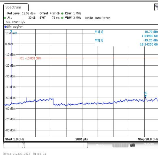
Band25-3MHz-16QAM-26055-1RB#0-Range4:1000~20000MHz-PASS
