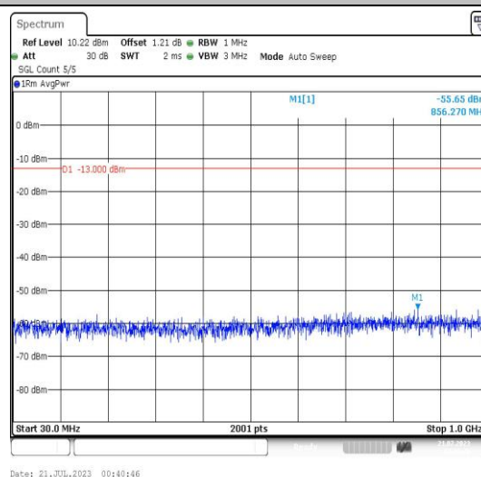
Band25-1.4MHz-16QAM-26683-1RB#0-Range3:30~1000MHz-PASS
