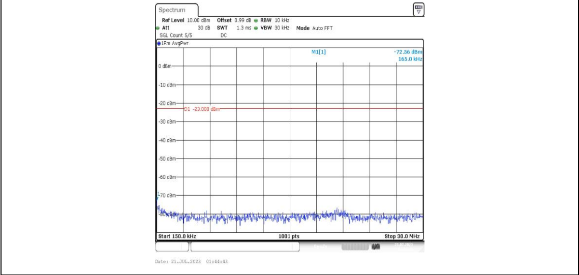
Band25-5MHz-16QAM-26365-1RB#0-Range2:0.15~30MHz-PASS
