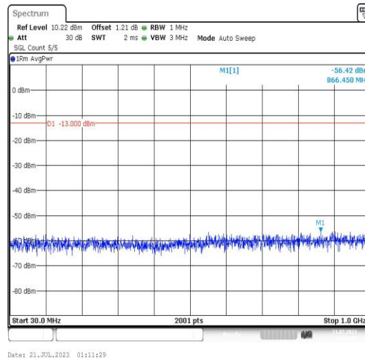
Band25-3MHz-16QAM-26365-1RB#0-Range3:30~1000MHz-PASS
