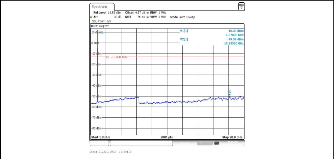
Band25-1.4MHz-16QAM-26365-1RB#0-Range4:1000~20000MHz-PASS
