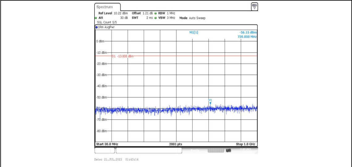
Band25-5MHz-16QAM-26065-1RB#0-Range3:30~1000MHz-PASS
