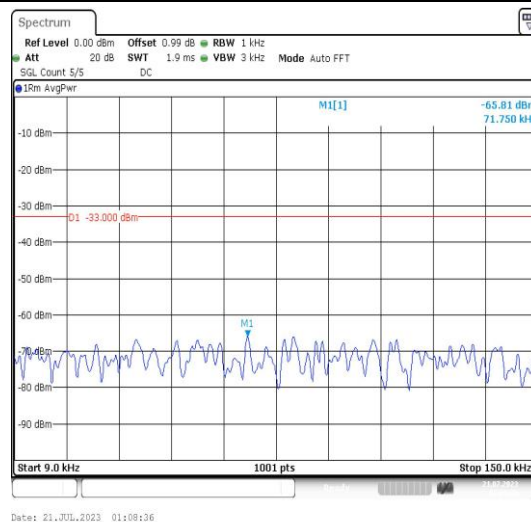
Band25-3MHz-QPSK-26055-1RB#0-Range1:0.009~0.15MHz-PASS
