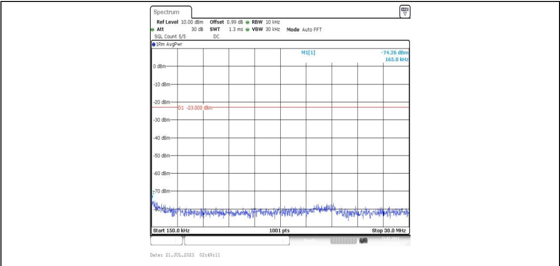
Band25-15MHz-16QAM-26115-1RB#0-Range2:0.15~30MHz-PASS
