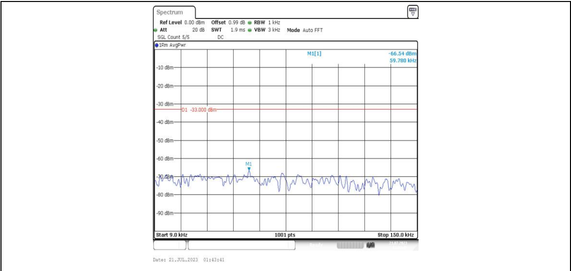
Band25-5MHz-QPSK-26365-1RB#0-Range1:0.009~0.15MHz-PASS
