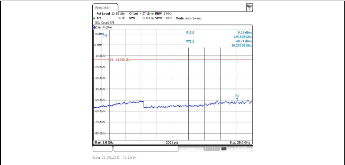
Band25-3MHz-16QAM-26675-1RB#0-Range4:1000~20000MHz-PASS
