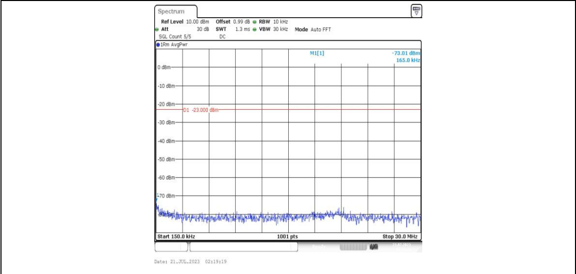
Band25-10MHz-16QAM-26640-1RB#0-Range2:0.15~30MHz-PASS
