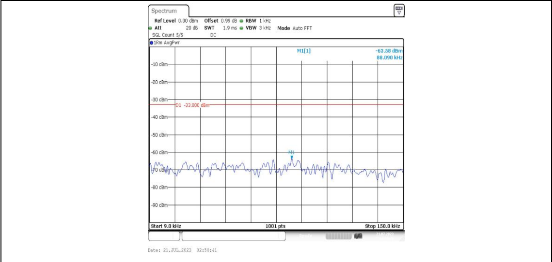
Band25-15MHz-16QAM-26365-1RB#0-Range1:0.009~0.15MHz-PASS
