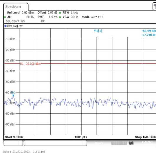
Band25-3MHz-16QAM-26365-1RB#0-Range1:0.009~0.15MHz-PASS
