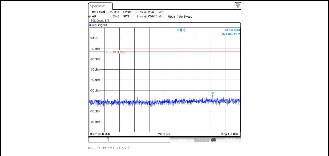
Band25-15MHz-QPSK-26365-1RB#0-Range3:30~1000MHz-PASS
