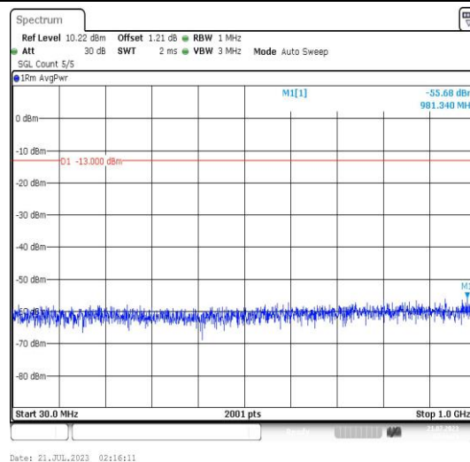
Band25-10MHz-16QAM-26090-1RB#0-Range3:30~1000MHz-PASS
