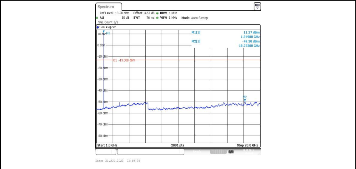
Band25-15MHz-16QAM-26115-1RB#0-Range4:1000~20000MHz-PASS
