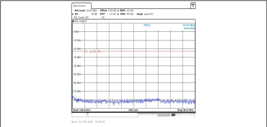
Band25-5MHz-QPSK-26665-1RB#0-Range2:0.15~30MHz-PASS
