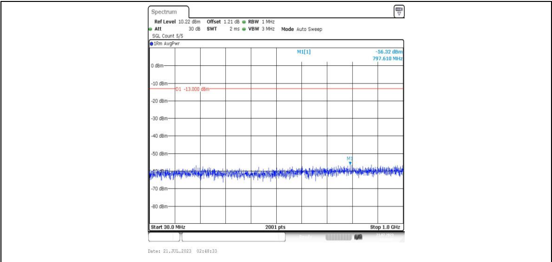
Band25-15MHz-QPSK-26115-1RB#0-Range3:30~1000MHz-PASS
