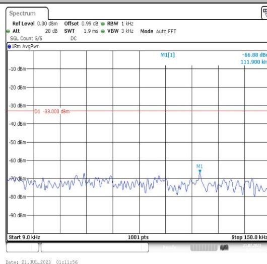
Band25-3MHz-QPSK-26675-1RB#0-Range1:0.009~0.15MHz-PASS
