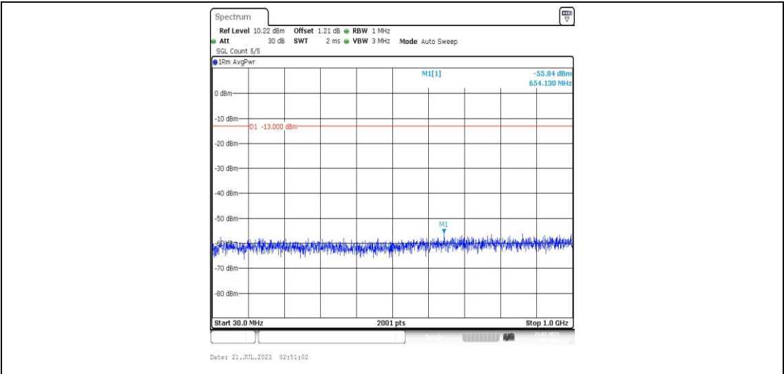
Band25-15MHz-16QAM-26365-1RB#0-Range3:30~1000MHz-PASS
