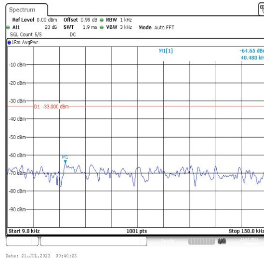
Band25-1.4MHz-16QAM-26683-1RB#0-Range1:0.009~0.15MHz-PASS
