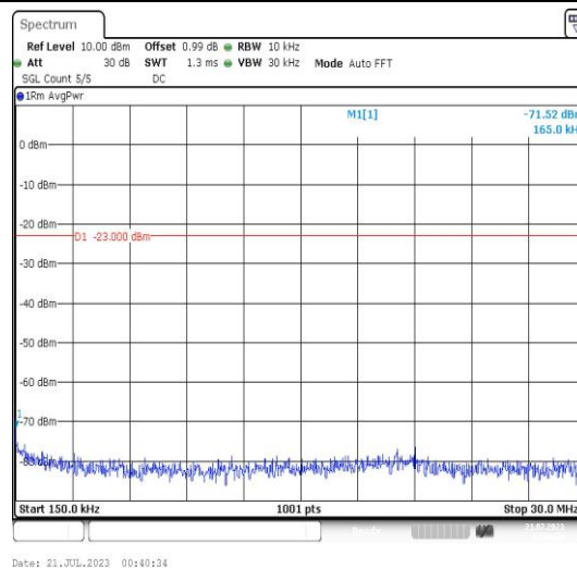
Band25-1.4MHz-16QAM-26683-1RB#0-Range2:0.15~30MHz-PASS
