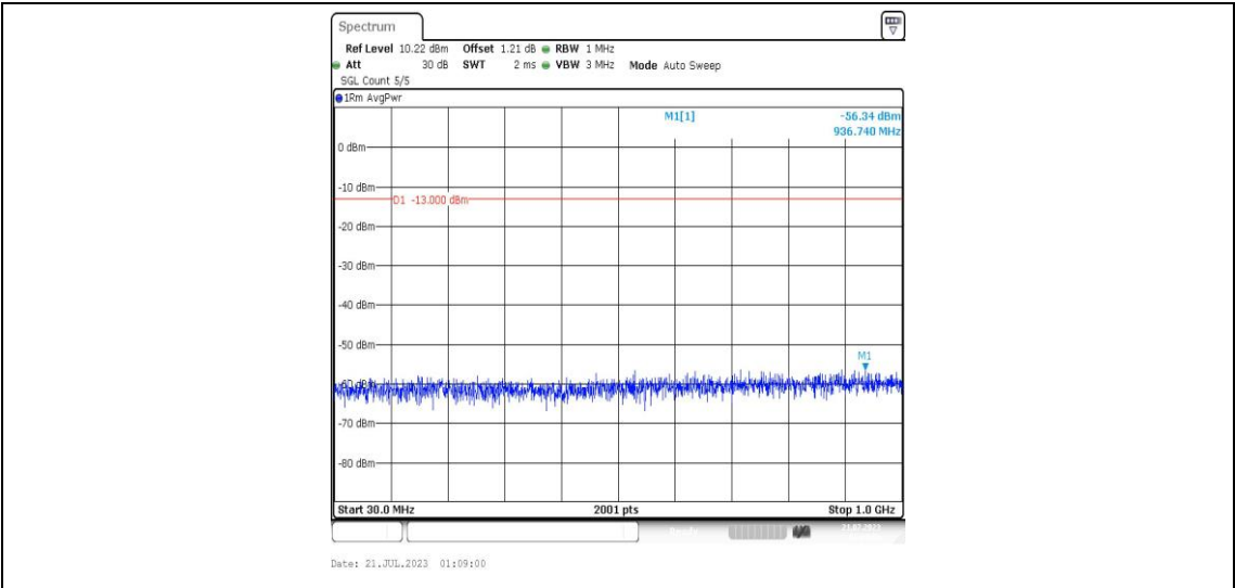
Band25-3MHz-QPSK-26055-1RB#0-Range3:30~1000MHz-PASS
