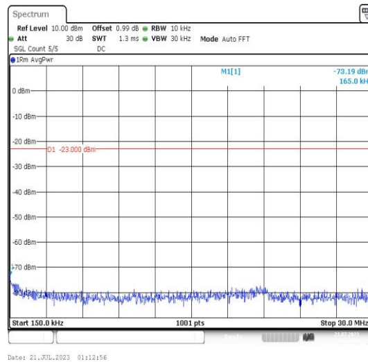
Band25-3MHz-16QAM-26675-1RB#0-Range2:0.15~30MHz-PASS
