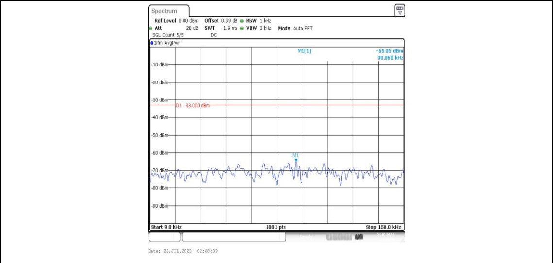
Band25-15MHz-QPSK-26115-1RB#0-Range1:0.009~0.15MHz-PASS
