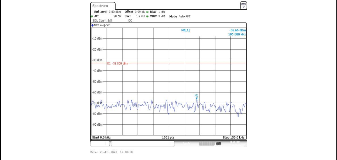
Band25-10MHz-QPSK-26640-1RB#0-Range1:0.009~0.15MHz-PASS
