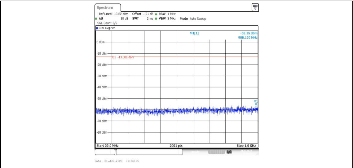
Band25-1.4MHz-QPSK-26047-1RB#0-Range3:30~1000MHz-PASS
