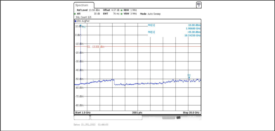
Band25-5MHz-QPSK-26665-1RB#0-Range4:1000~20000MHz-PASS
