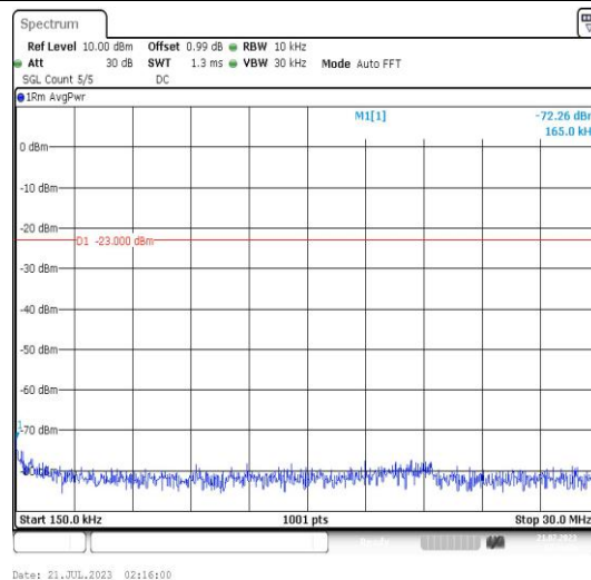
Band25-10MHz-16QAM-26090-1RB#0-Range2:0.15~30MHz-PASS
