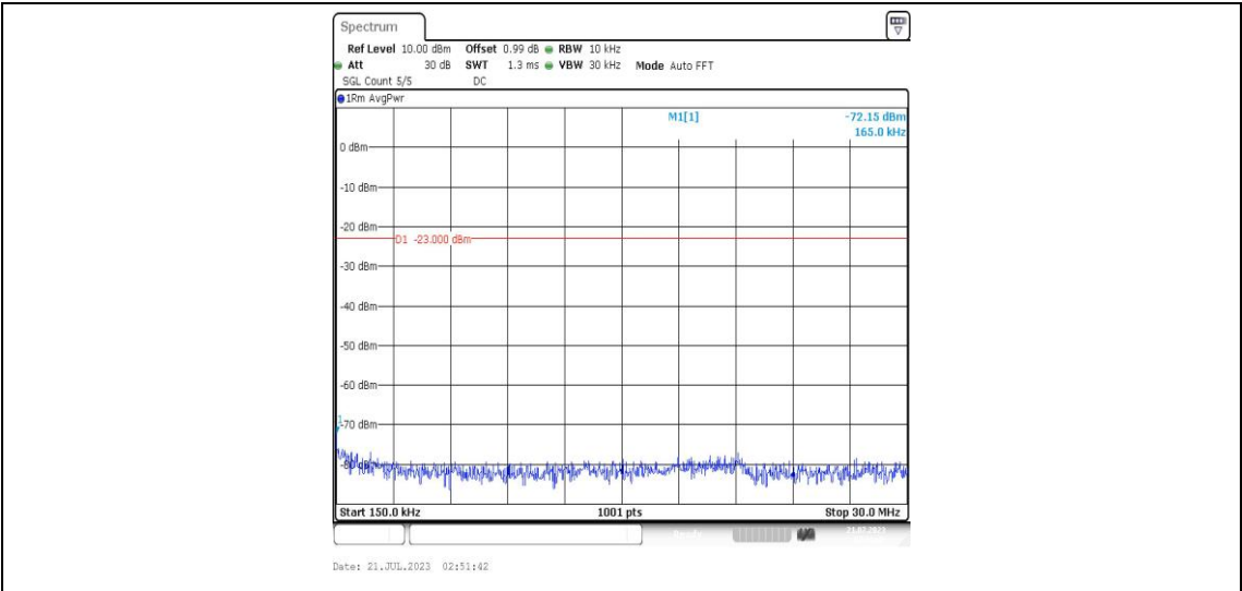
Band25-15MHz-QPSK-26615-1RB#0-Range2:0.15~30MHz-PASS
