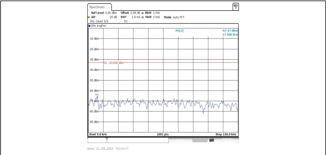
Band25-3MHz-QPSK-26365-1RB#0-Range1:0.009~0.15MHz-PASS
