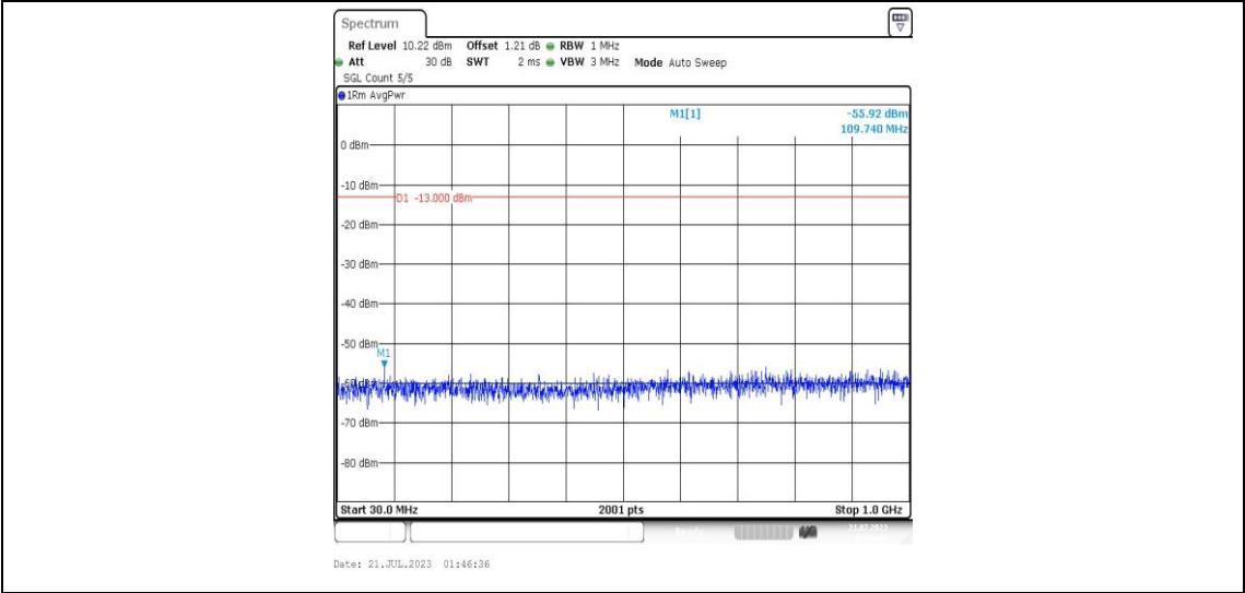
Band25-5MHz-16QAM-26665-1RB#0-Range3:30~1000MHz-PASS
