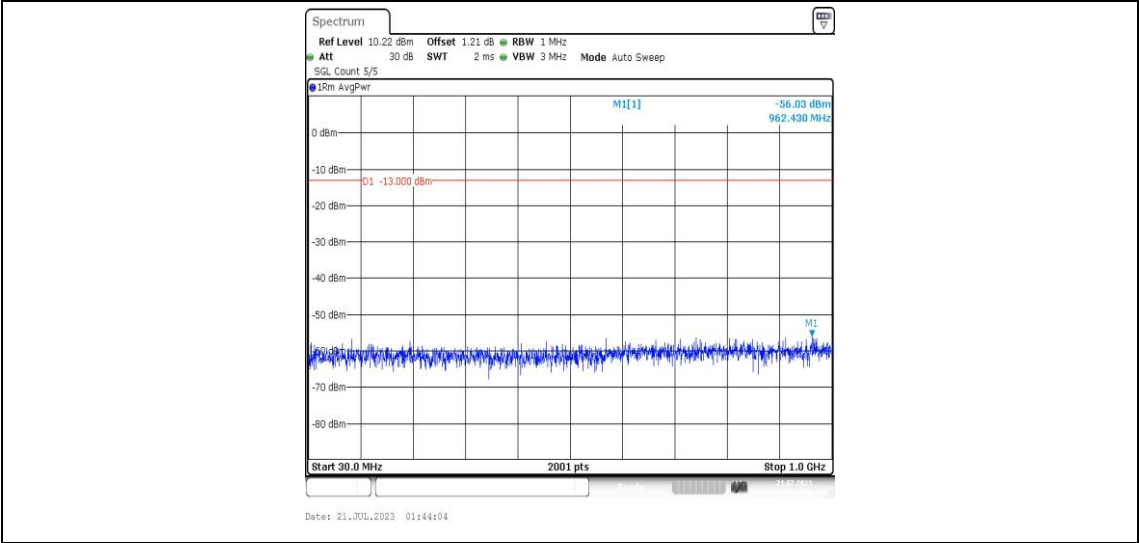
Band25-5MHz-QPSK-26365-1RB#0-Range3:30~1000MHz-PASS
