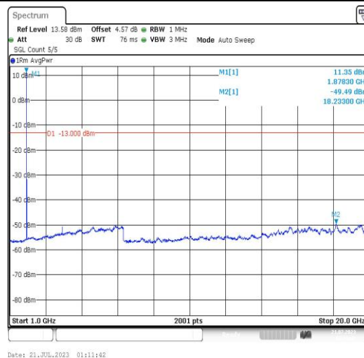
Band25-3MHz-16QAM-26365-1RB#0-Range4:1000~20000MHz-PASS
