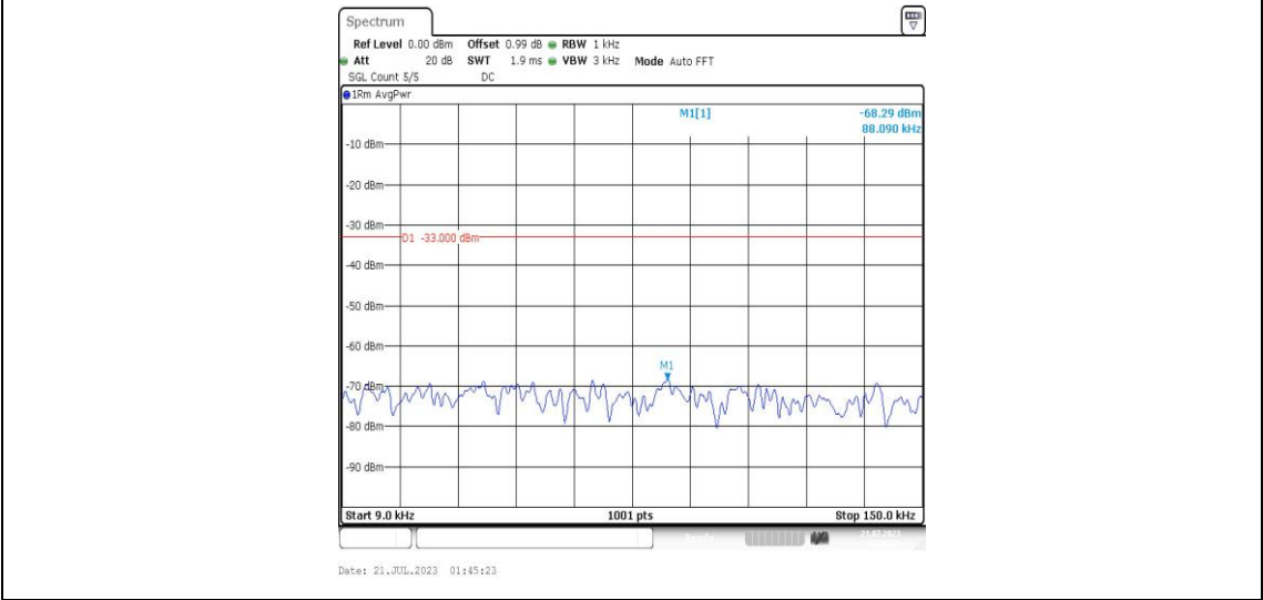
Band25-5MHz-QPSK-26665-1RB#0-Range1:0.009~0.15MHz-PASS
