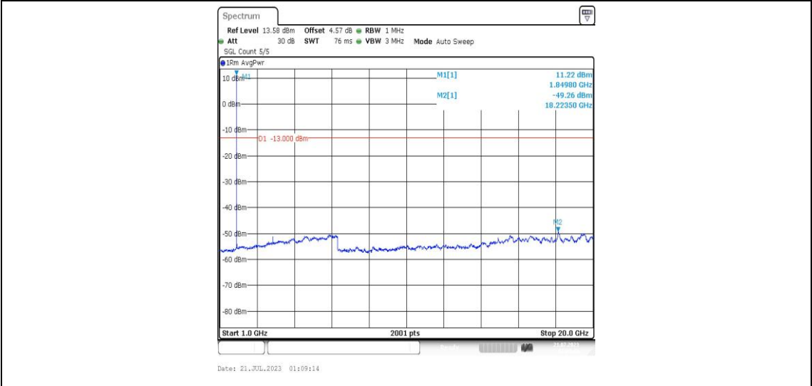
Band25-3MHz-QPSK-26055-1RB#0-Range4:1000~20000MHz-PASS
