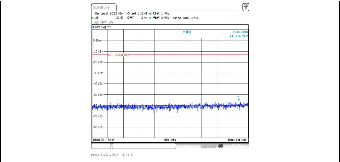
Band25-5MHz-16QAM-26365-1RB#0-Range3:30~1000MHz-PASS
