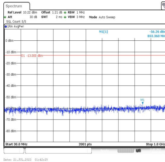
Band25-5MHz-QPSK-26065-1RB#0-Range3:30~1000MHz-PASS
