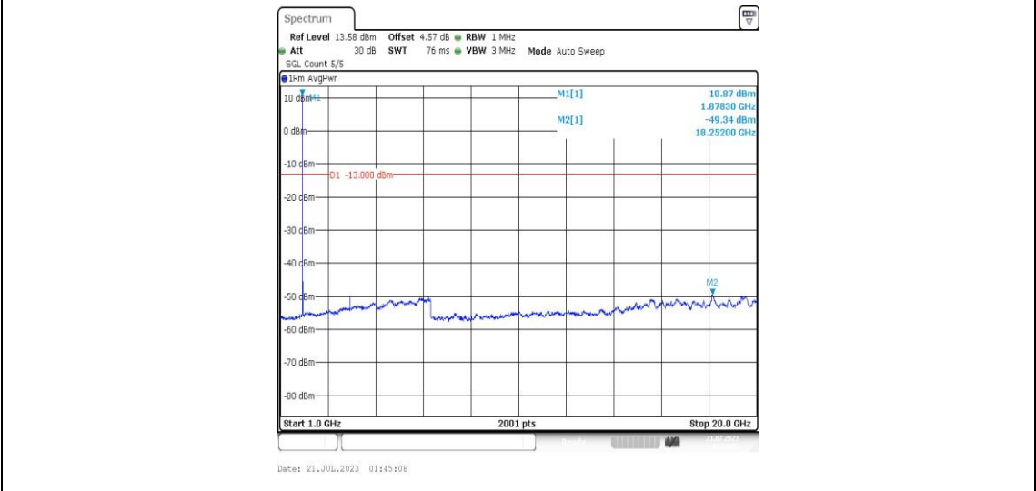
Band25-5MHz-16QAM-26365-1RB#0-Range4:1000~20000MHz-PASS
