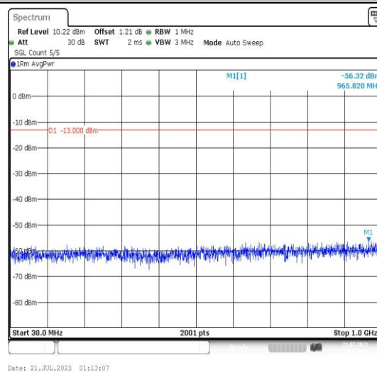
Band25-3MHz-16QAM-26675-1RB#0-Range3:30~1000MHz-PASS
