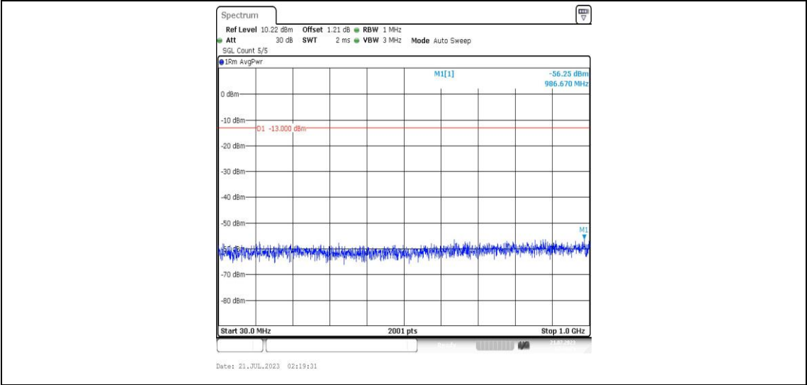
Band25-10MHz-16QAM-26640-1RB#0-Range3:30~1000MHz-PASS
