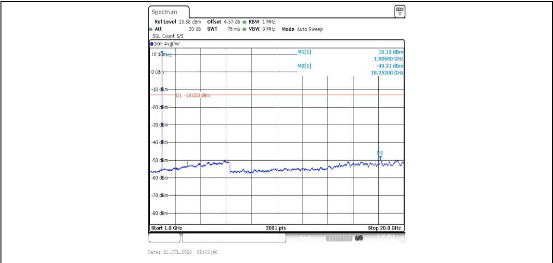
Band25-10MHz-16QAM-26640-1RB#0-Range4:1000~20000MHz-PASS
