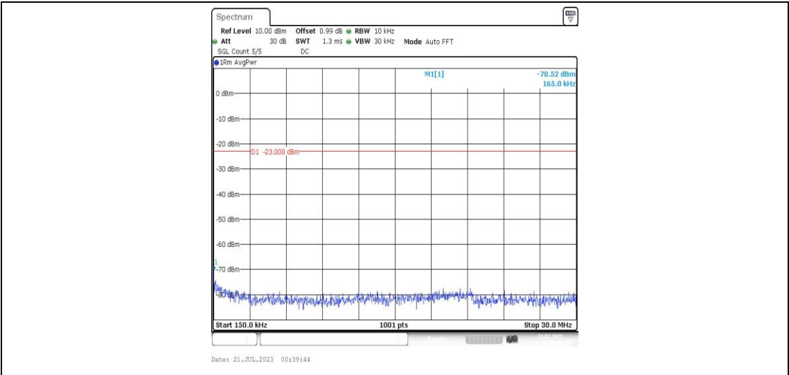
Band25-1.4MHz-QPSK-26683-1RB#0-Range2:0.15~30MHz-PASS
