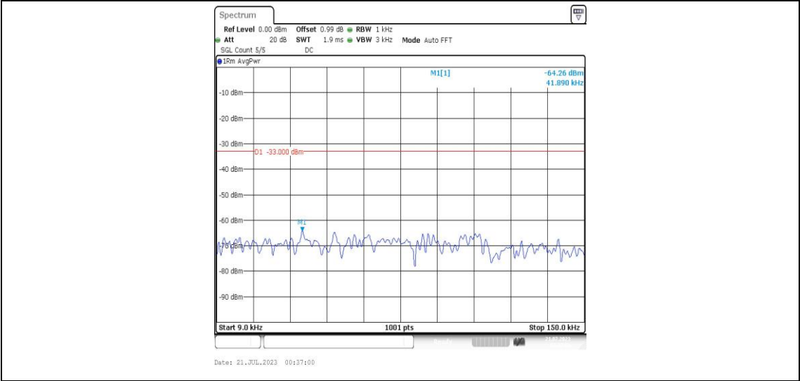
Band25-1.4MHz-16QAM-26047-1RB#0-Range1:0.009~0.15MHz-PASS
