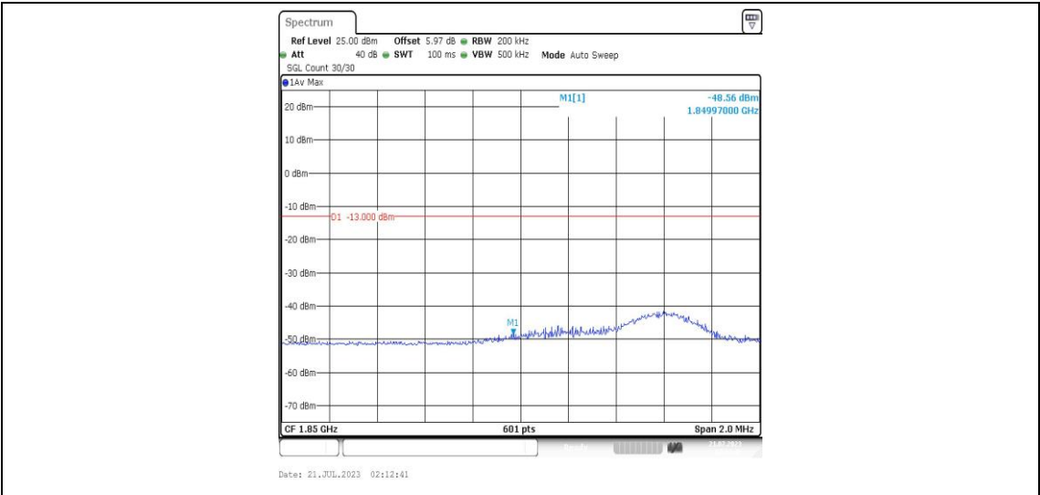
Band25-10MHz-16QAM-26090-1RB#49-PASS
