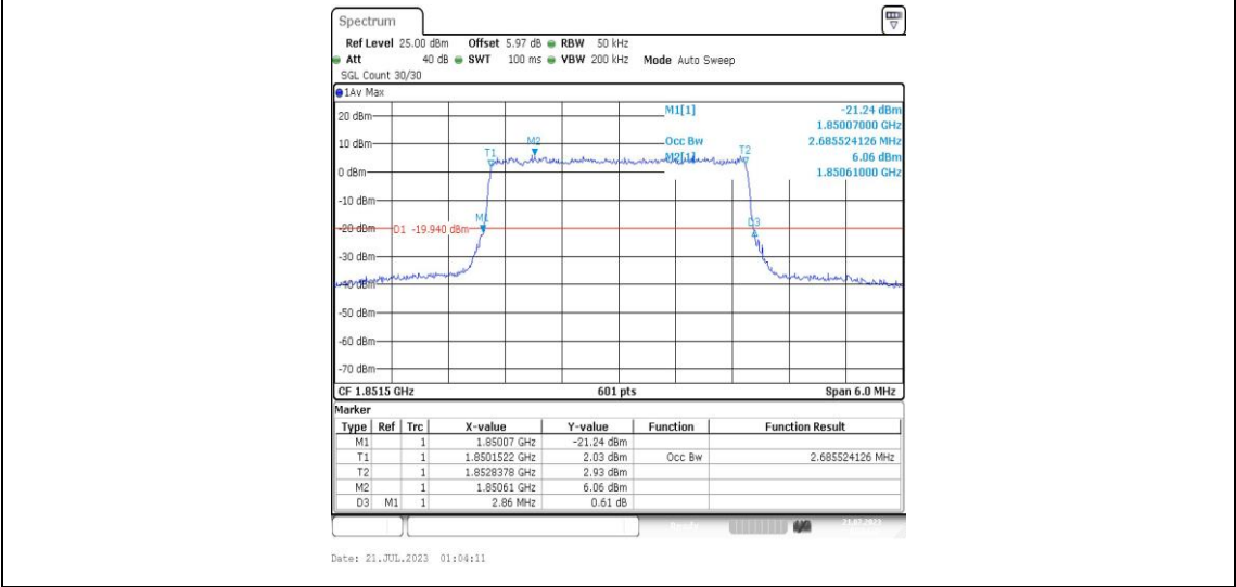
Band25-3MHz-16QAM-26055-15RB#0-PASS
