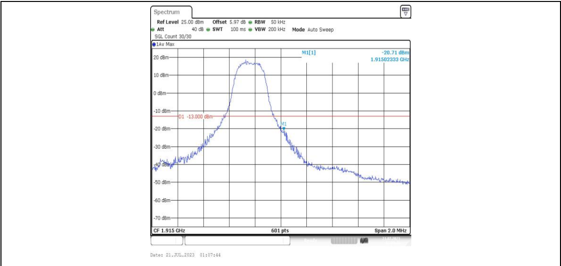
Band25-3MHz-16QAM-26675-1RB#14-PASS
