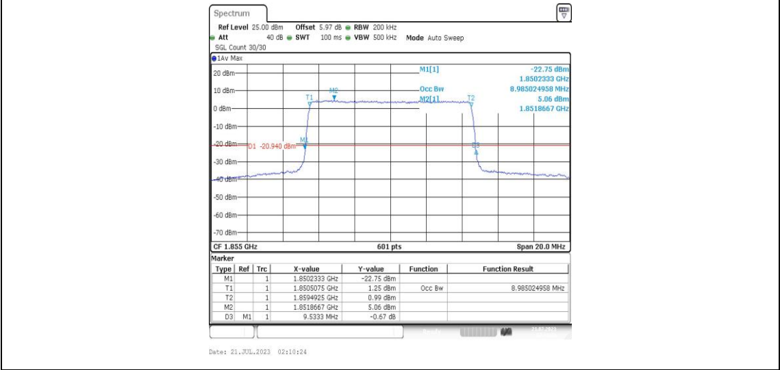
Band25-10MHz-16QAM-26090-50RB#0-PASS
