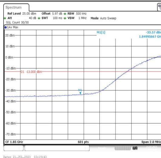
Band25-20MHz-16QAM-26140-100RB#0-PASS
