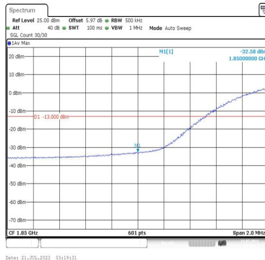
Band25-20MHz-QPSK-26140-100RB#0-PASS
