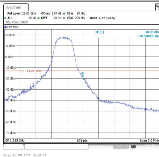
Band25-3MHz-QPSK-26675-1RB#14-PASS
