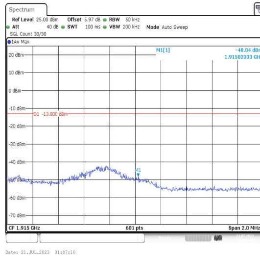
Band25-3MHz-QPSK-26675-1RB#0-PASS
