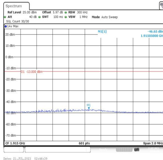
Band25-15MHz-QPSK-26615-1RB#0-PASS
