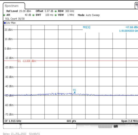
Band25-15MHz-16QAM-26615-1RB#0-PASS
