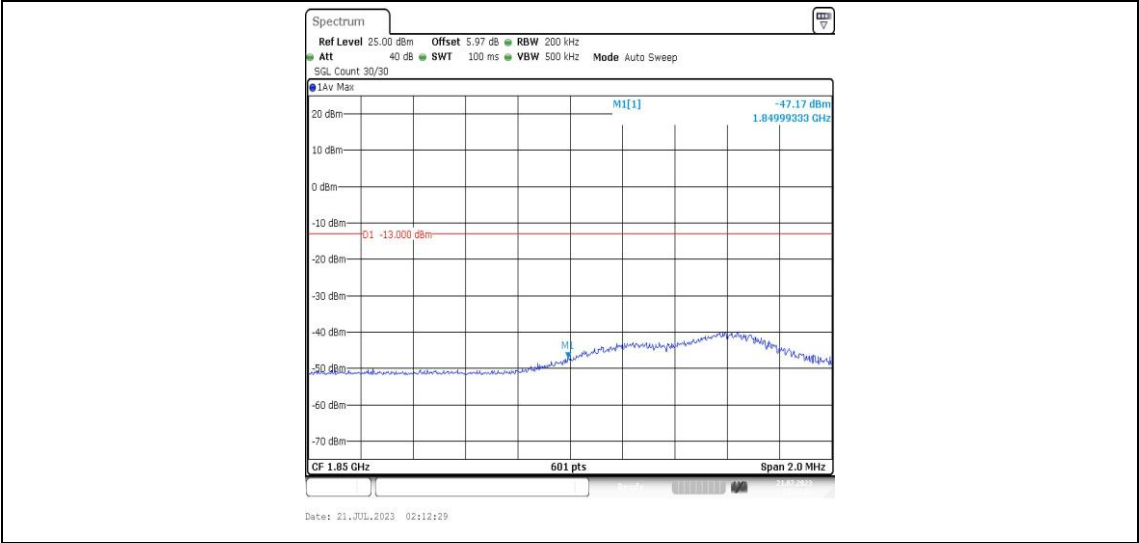
Band25-10MHz-QPSK-26090-1RB#49-PASS
