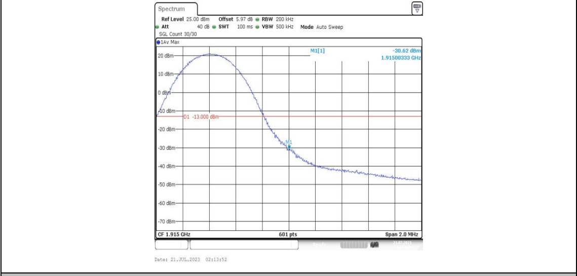
Band25-10MHz-QPSK-26640-1RB#49-PASS
