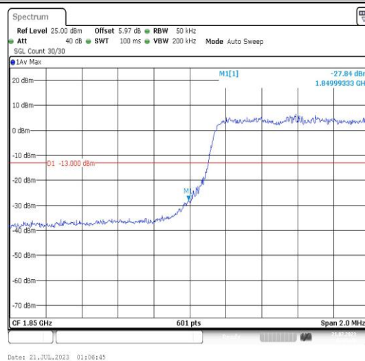
Band25-3MHz-16QAM-26055-15RB#0-PASS
