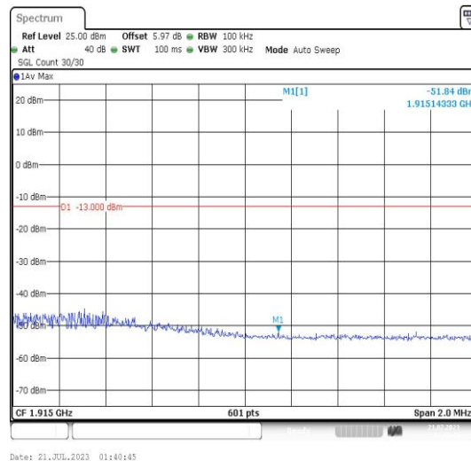
Band25-5MHz-16QAM-26665-1RB#0-PASS
