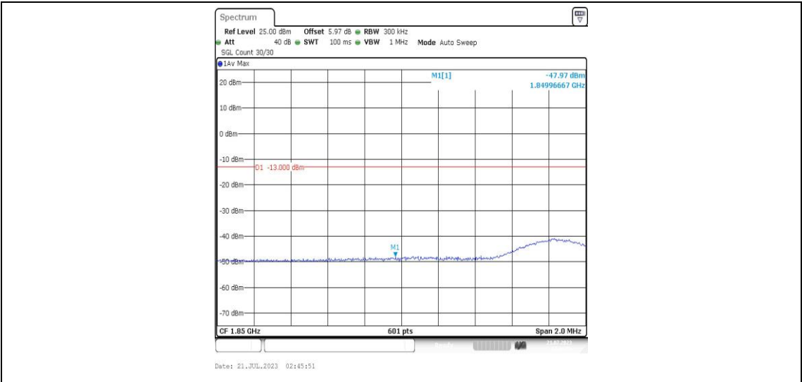
Band25-15MHz-16QAM-26115-1RB#74-PASS
