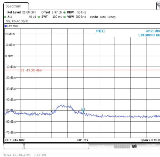
Band25-3MHz-16QAM-26675-1RB#0-PASS
