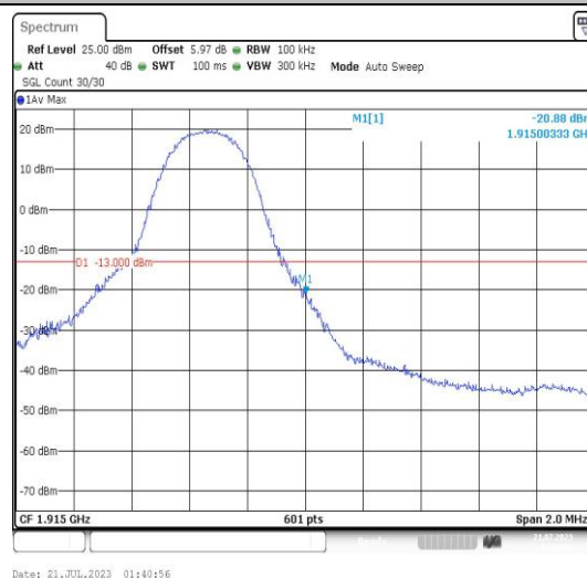
Band25-5MHz-QPSK-26665-1RB#24-PASS
