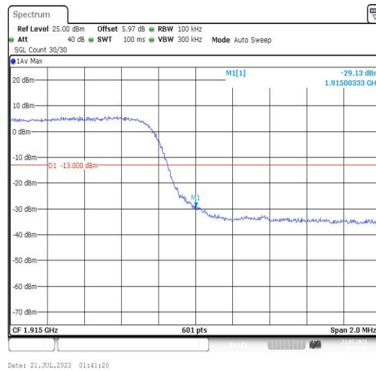
Band25-5MHz-QPSK-26665-25RB#0-PASS
