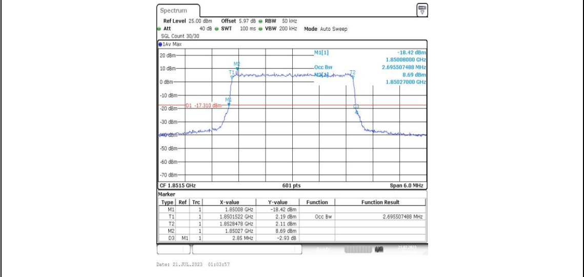
Band25-3MHz-QPSK-26055-15RB#0-PASS
