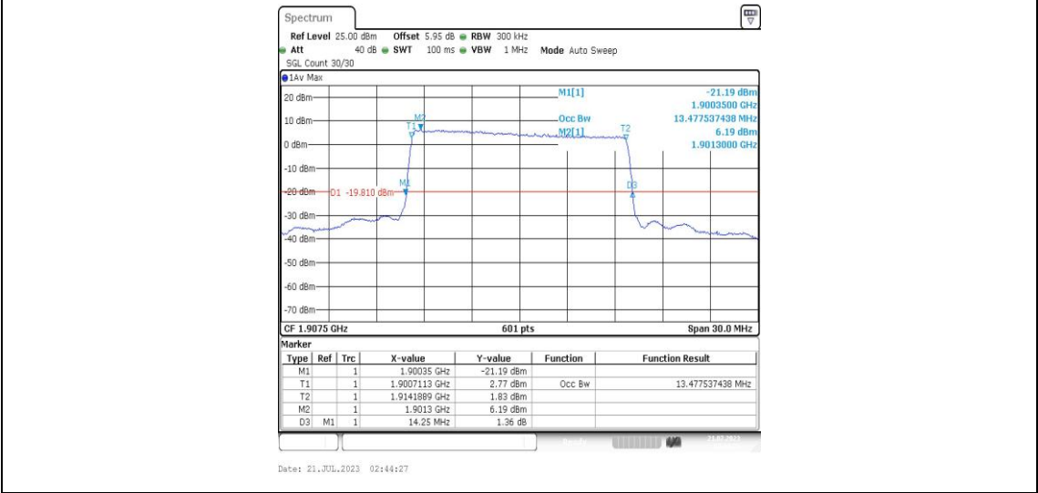
Band25-15MHz-QPSK-26615-75RB#0-PASS
