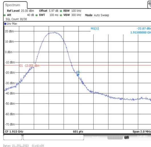
Band25-5MHz-16QAM-26665-1RB#24-PASS
