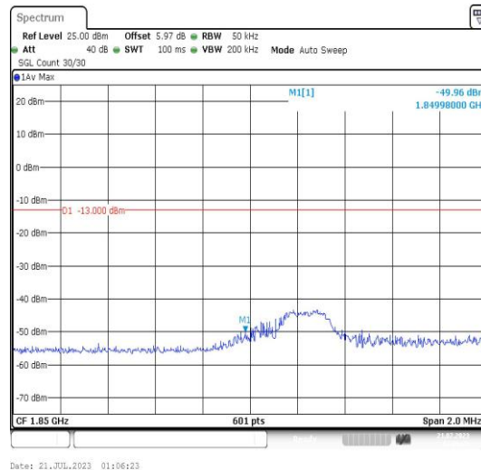
Band25-3MHz-16QAM-26055-1RB#14-PASS
