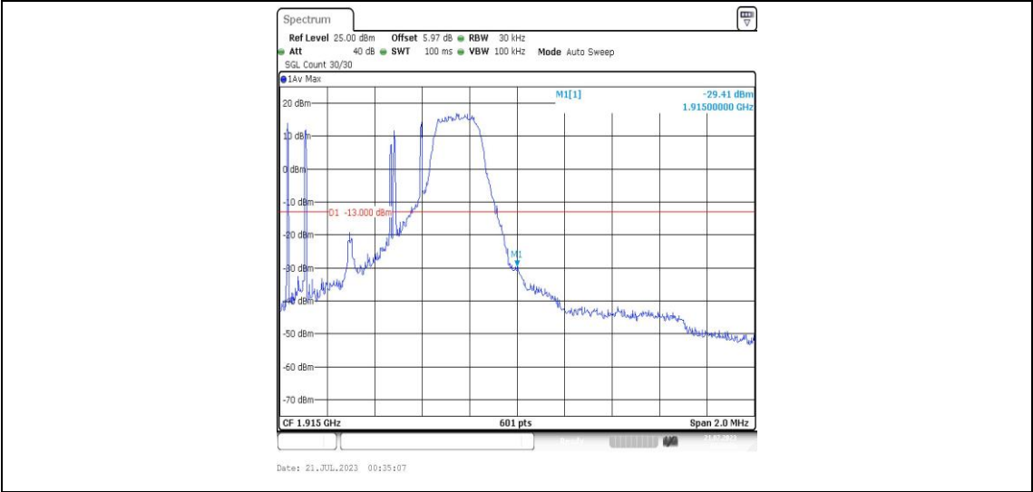
Band25-1.4MHz-QPSK-26683-1RB#5-PASS
