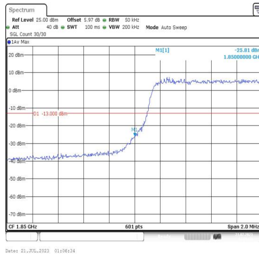
Band25-3MHz-QPSK-26055-15RB#0-PASS
