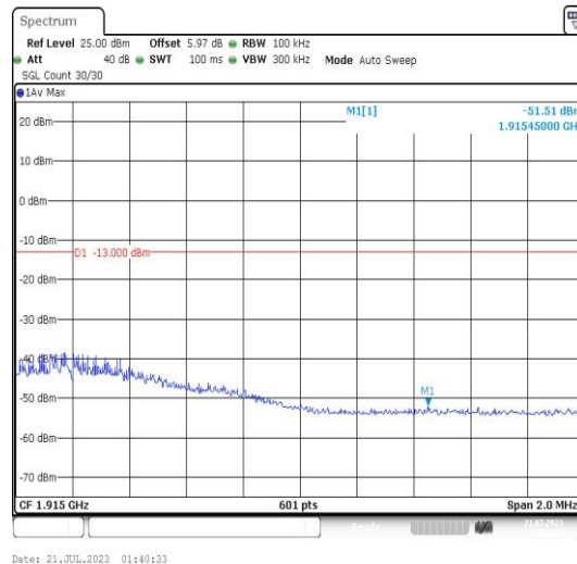
Band25-5MHz-QPSK-26665-1RB#0-PASS
