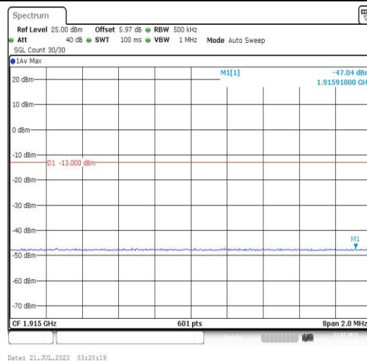
Band25-20MHz-16QAM-26590-1RB#0-PASS
