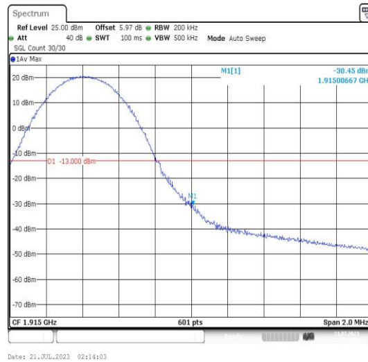
Band25-10MHz-16QAM-26640-1RB#49-PASS
