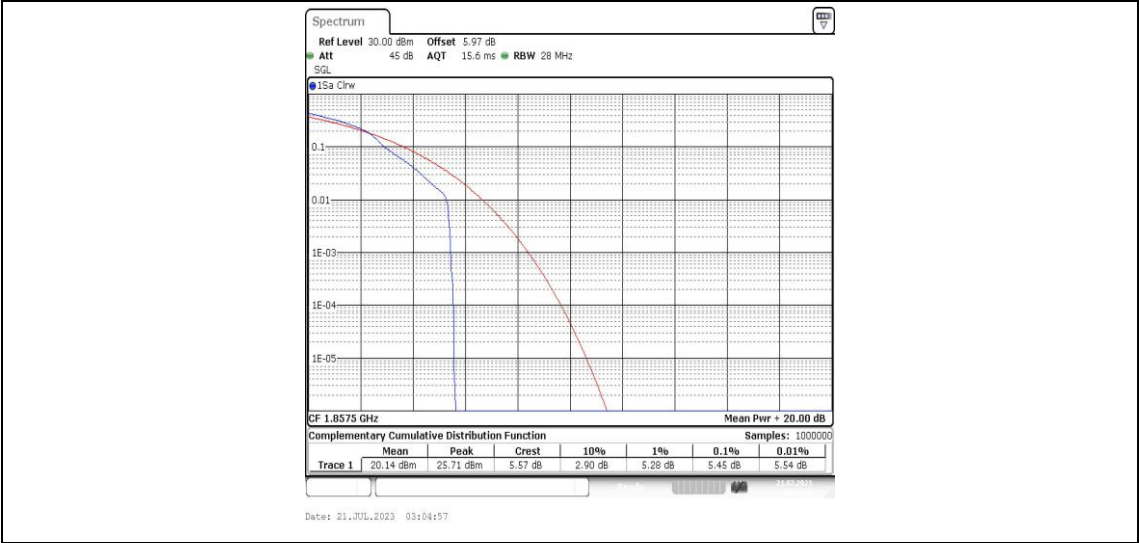
Band25-15MHz-16QAM-26115-1RB#0-PASS
