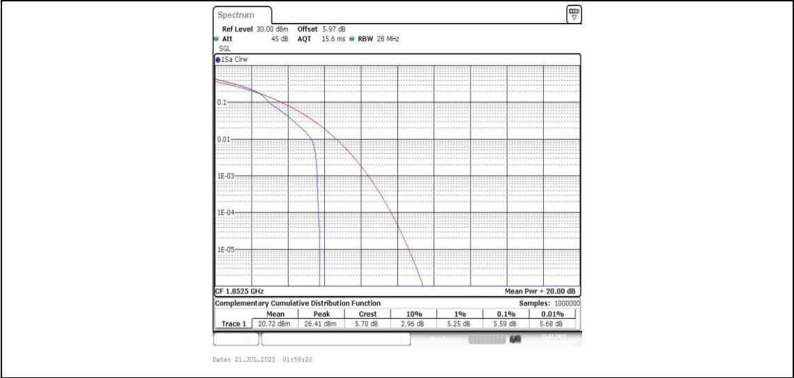
Band25-5MHz-16QAM-26065-1RB#0-PASS
