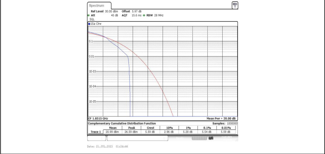
Band25-3MHz-16QAM-26055-1RB#0-PASS
