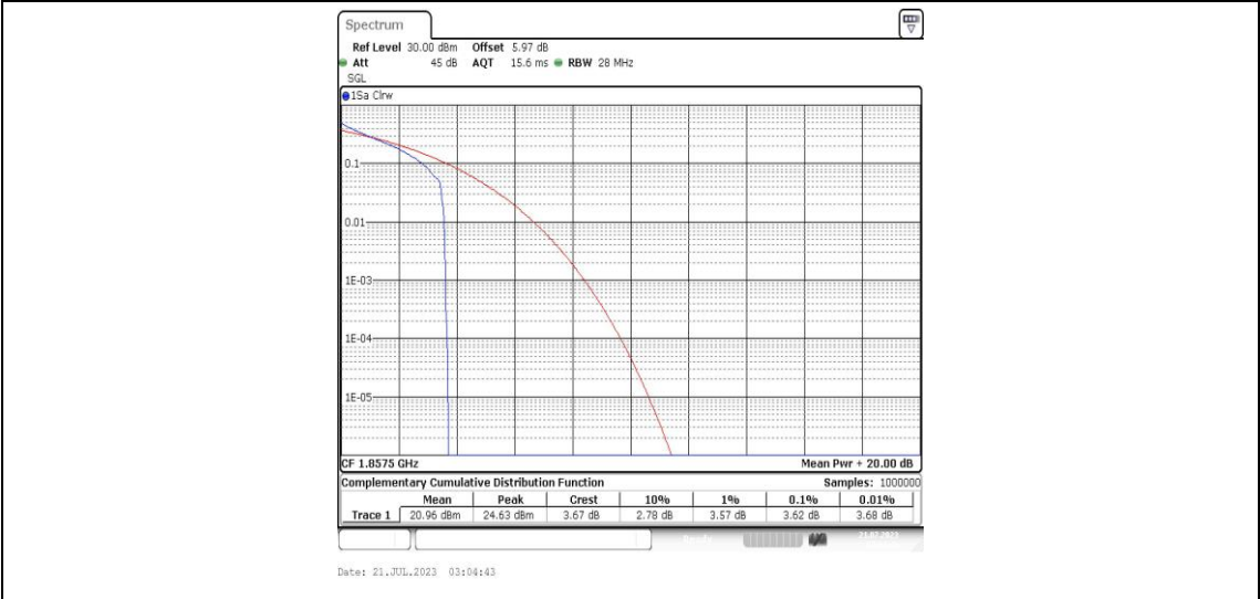
Band25-15MHz-QPSK-26115-1RB#0-PASS
