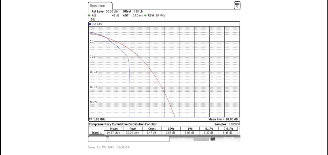
Band25-20MHz-16QAM-26140-1RB#0-PASS
