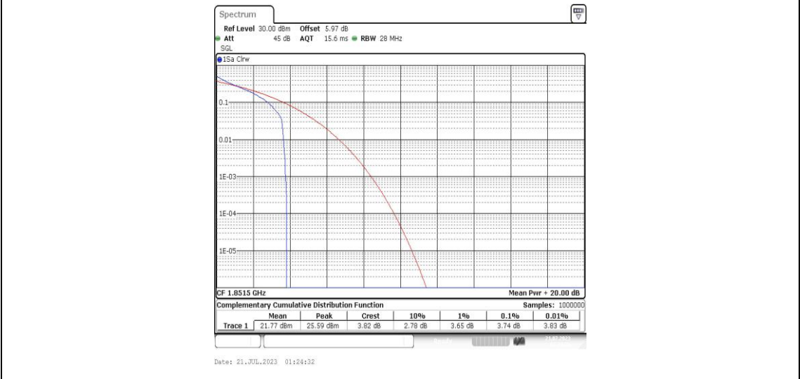
Band25-3MHz-QPSK-26055-1RB#0-PASS
