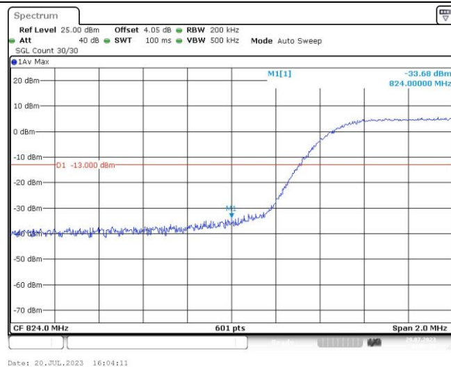
Band5-10MHz-QPSK-20600-1RB#0
