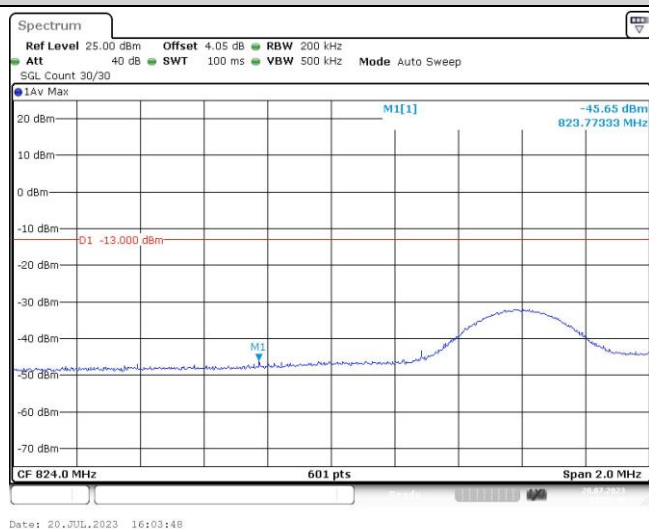
Band5-10MHz-QPSK-20450-50RB#0
