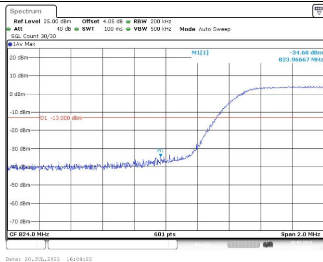
Band5-10MHz-16QAM-20600-1RB#0
