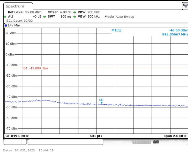
Band5-10MHz-16QAM-20600-1RB#49
