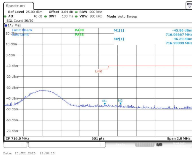
Band12-10MHz-QPSK-23130-1RB#49
