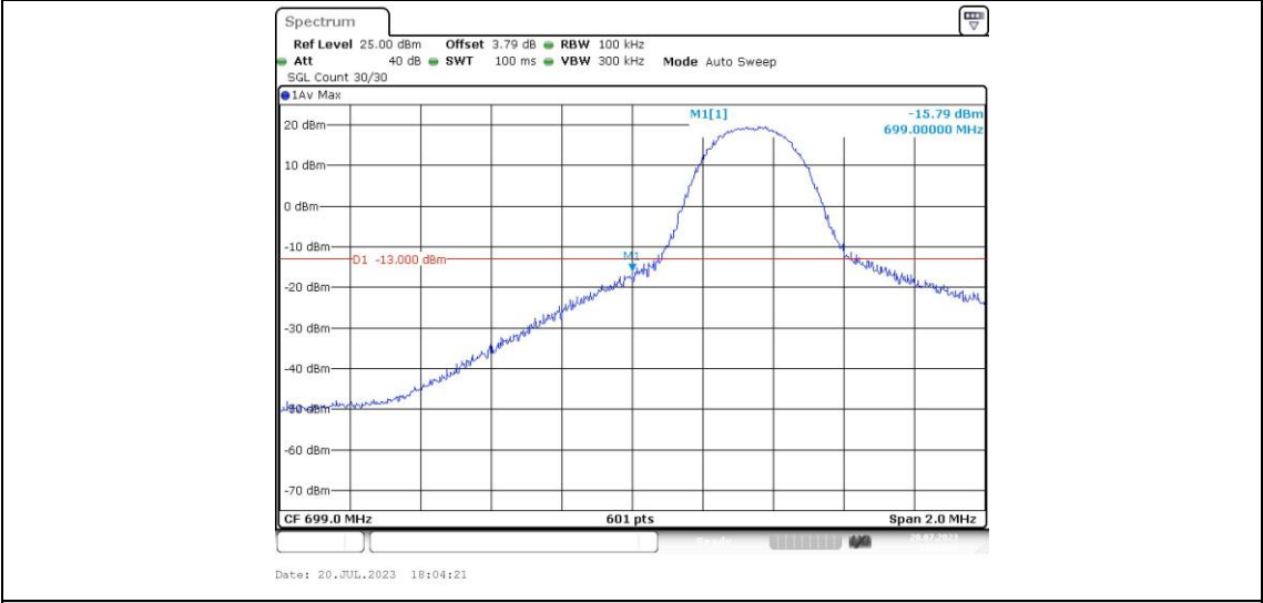
Band12-5MHz-QPSK-23035-1RB#24
