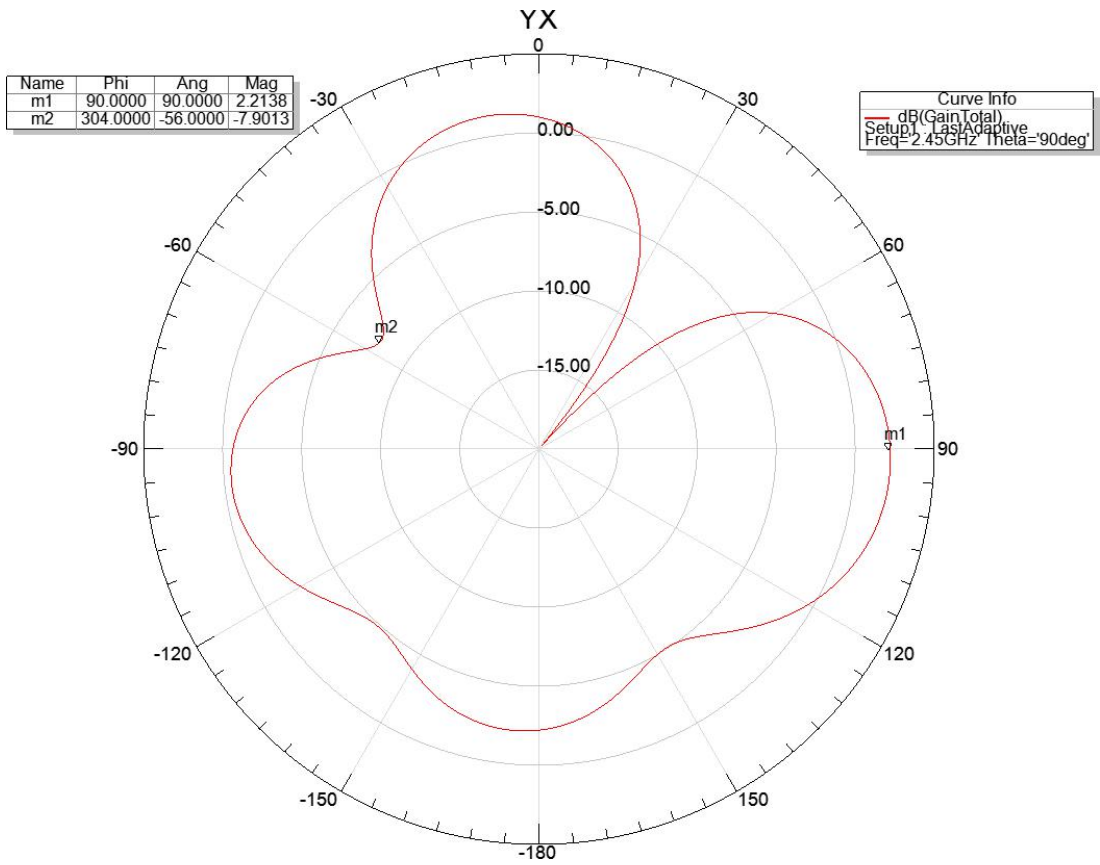
Radiation Pattern 2
