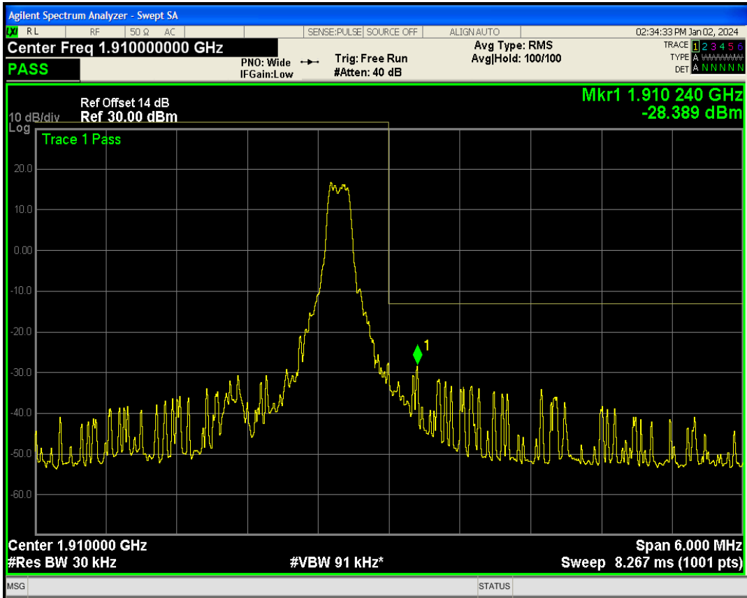
Band2 QPSK BW=3MHz Channel=19185 RB Size=6 Position=#Max NB Index=1
