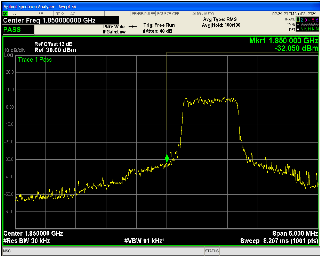
Band2 QPSK BW=3MHz Channel=19185 RB Size=1 Position=#Max NB Index=1
