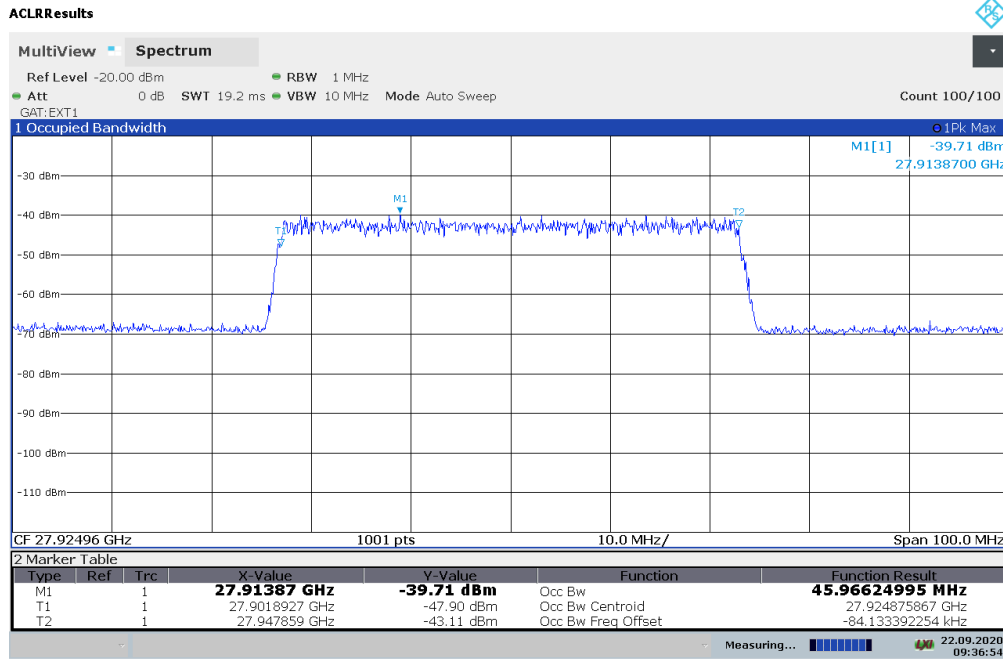
Plot 6-1. Occupied Bandwidth Input at 0.5dB below AGC Threshold.
