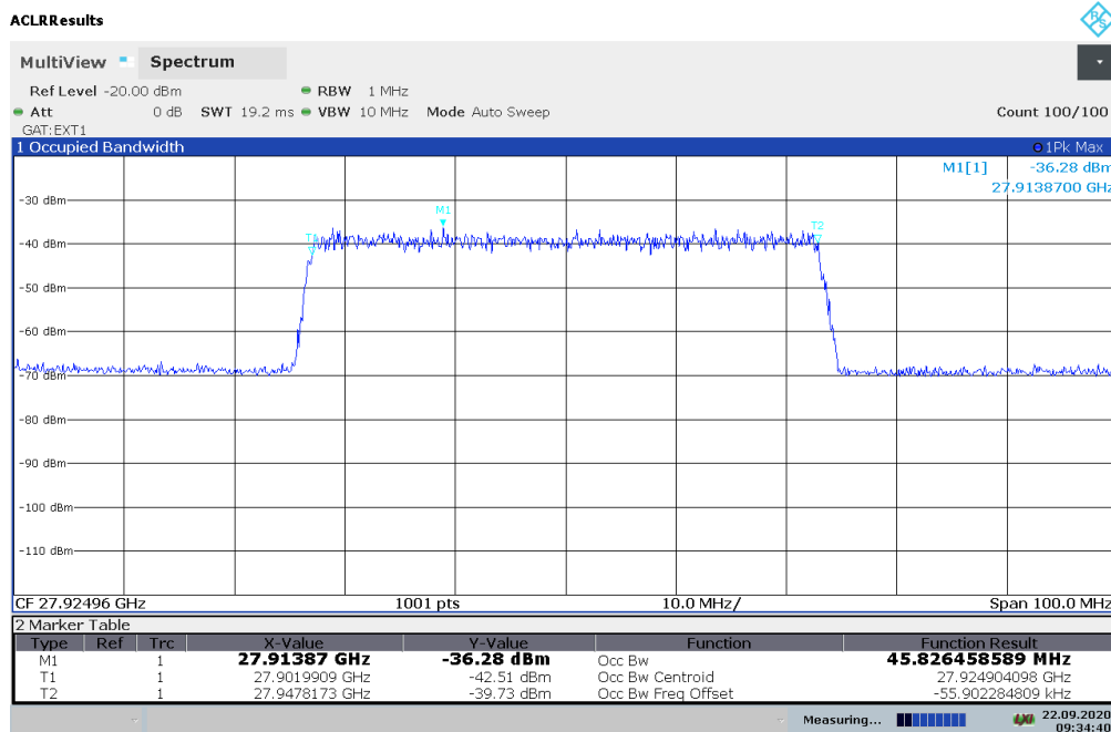
Plot 6-2. Occupied Bandwidth Input at 3dB above AGC Threshold.
