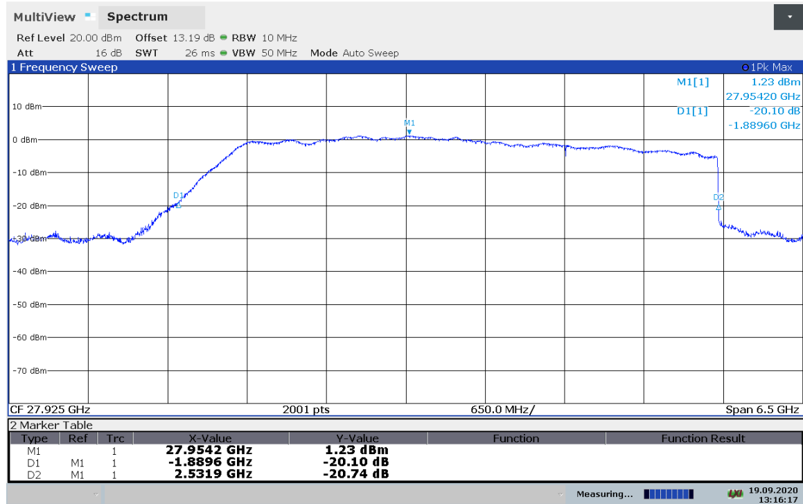
Plot 6-9. HBF Antenna Out-Of-Band Rejection
