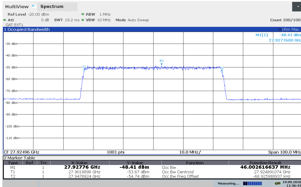
Plot 6-1. HBF Antenna Occupied Bandwidth Input at 0.5dB below AGC Threshold.
