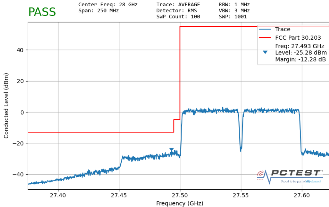
Plot 6-5. HBF Antenna Lower Band Edge Plot with 2 Carriers – Full RB.
