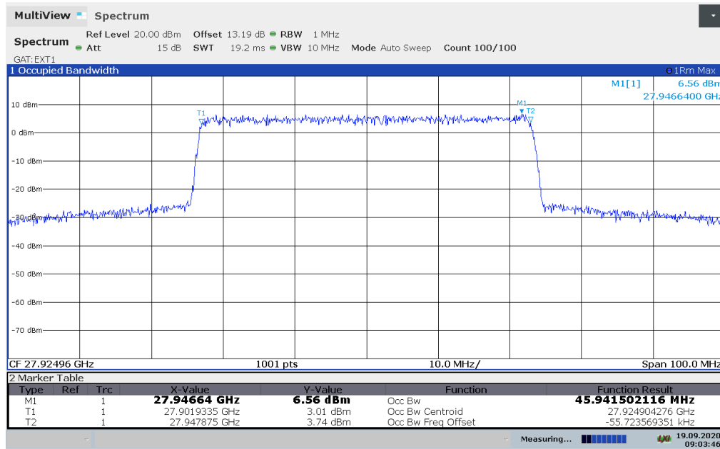
Plot 6-3. HBF Antenna Occupied Bandwidth Output at 0.5dB below AGC Threshold.
