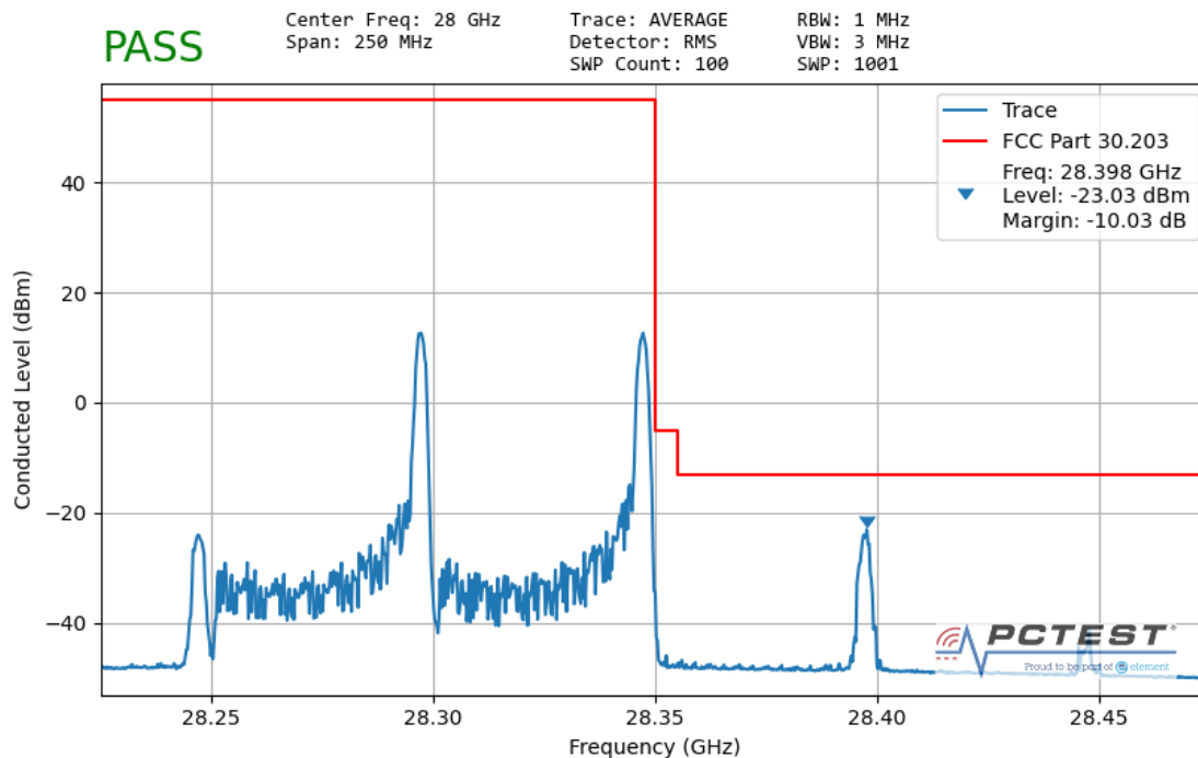
Plot 6-8. HBF Antenna Upper Band Edge Plot with 2 Carriers – 1RB.
