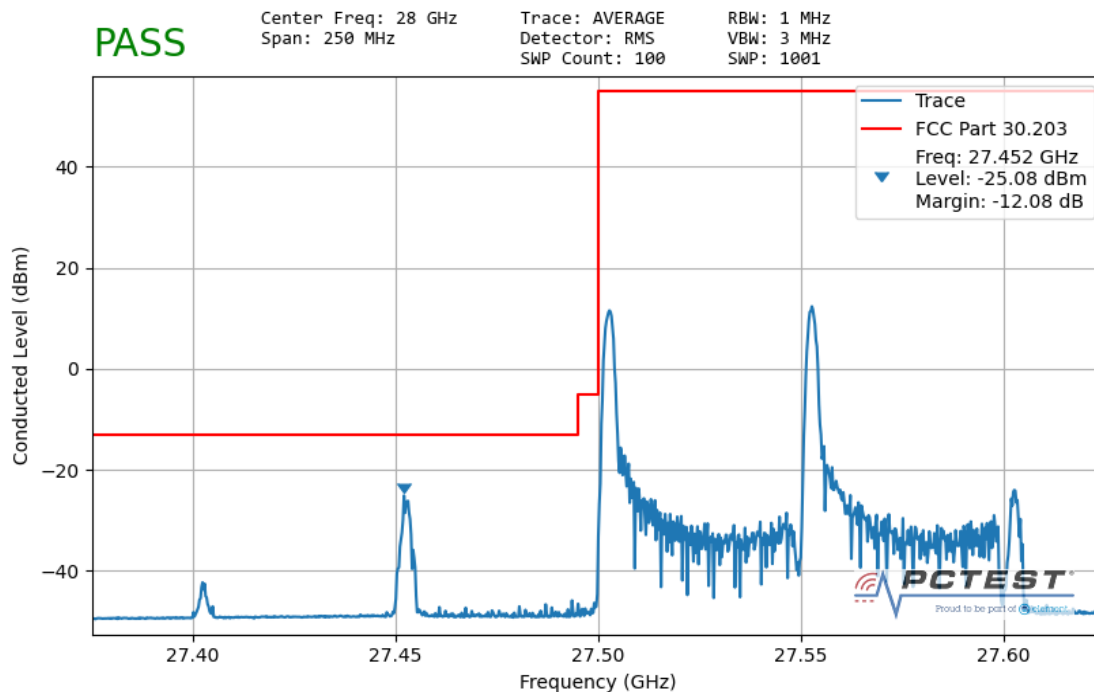
Plot 6-6. HBF Antenna Lower Band Edge Plot with 2 Carriers – 1RB.
