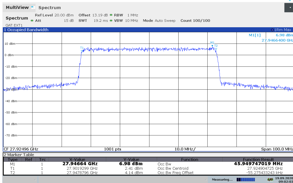
Plot 6-4. HBF Antenna Occupied Bandwidth Output at 3dB above AGC Threshold.
