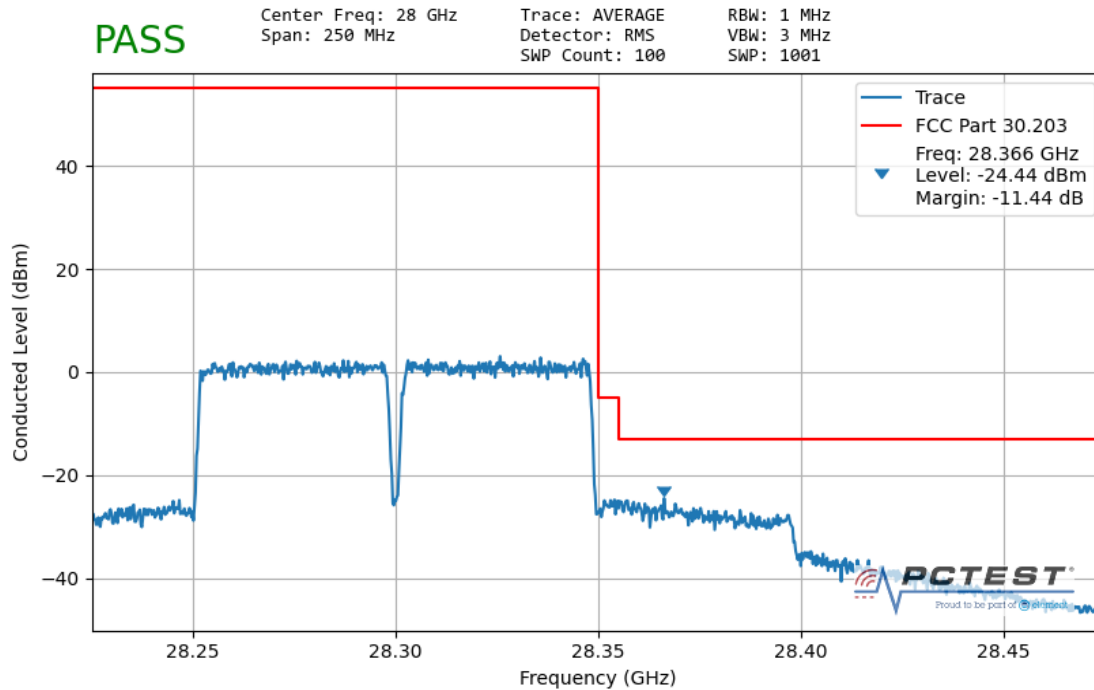
Plot 6-7. HBF Antenna Upper Band Edge Plot with 2 Carriers – Full RB.
