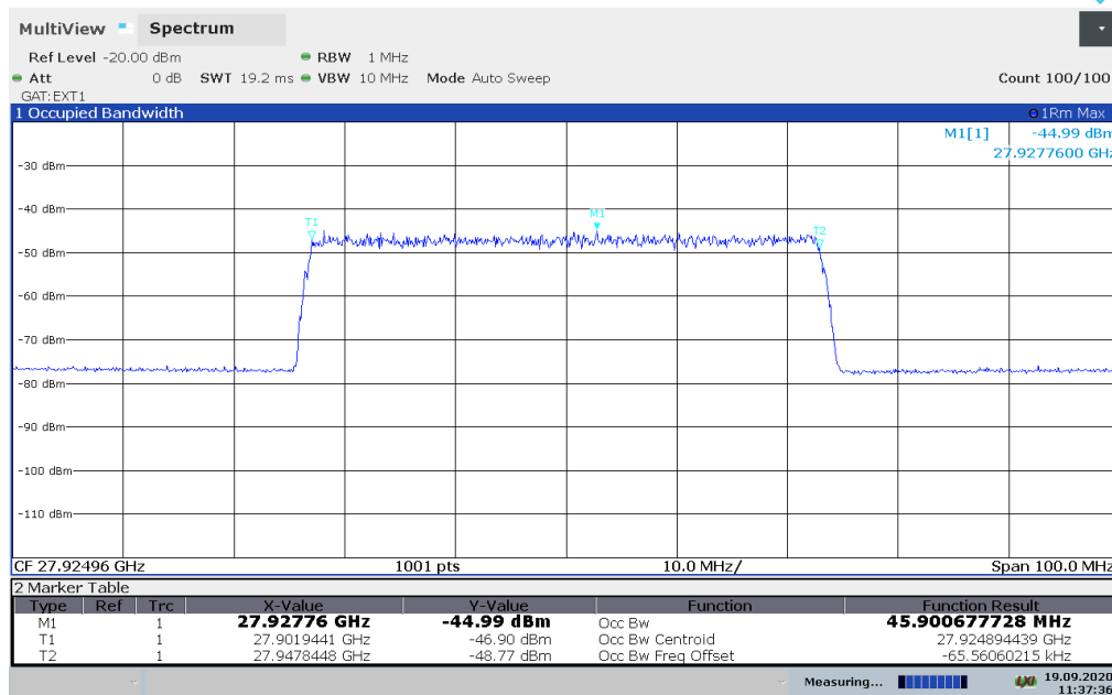
Plot 6-2. HBF Antenna Occupied Bandwidth Input at 3dB above AGC Threshold.
