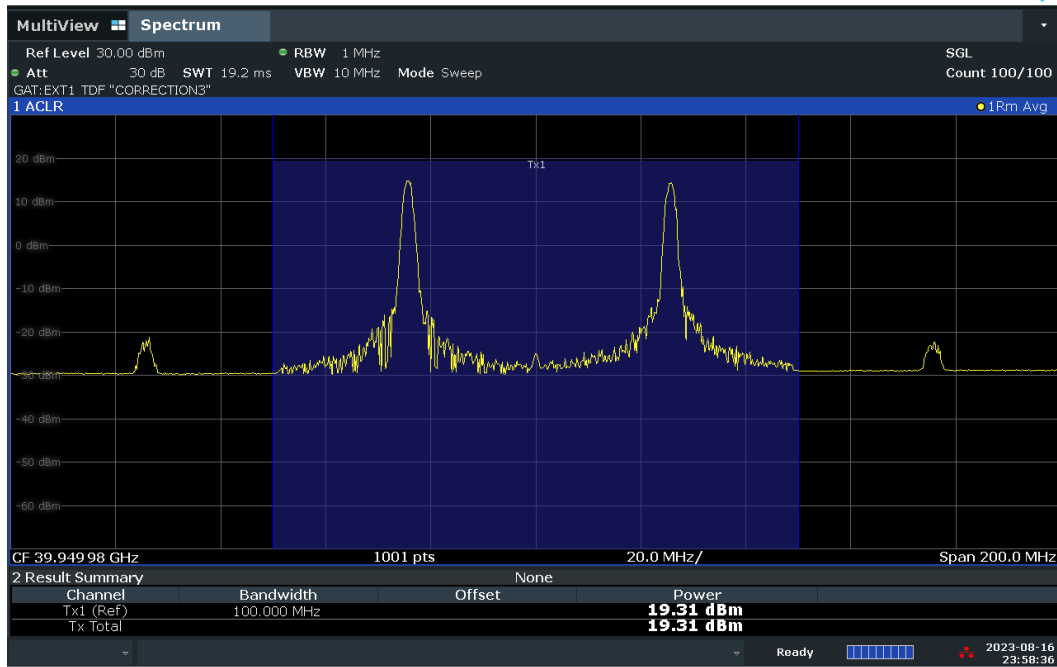
Plot 7-76. Conducted Power Plot – DFT-S – H-DL Polarization (50MHz-2CC – QPSK – High Ch. – 1 RB)
