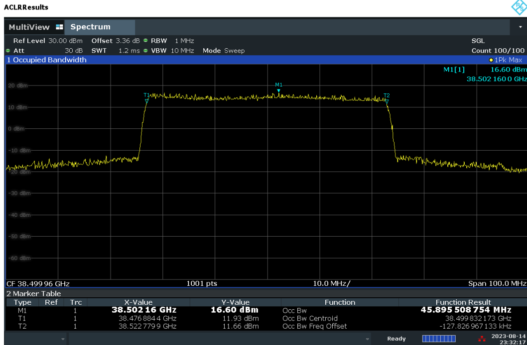
Plot 7-19. Occupied Bandwidth Plot – DFT-s – V-DL Polarization (50MHz-1CC – QPSK – Mid Channel)
