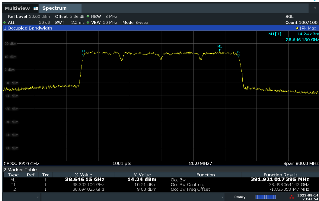
Plot 7-24. Occupied Bandwidth Plot – DFT-s – V-DL Polarization (100MHz-4CC – 16QAM – Mid Channel)
