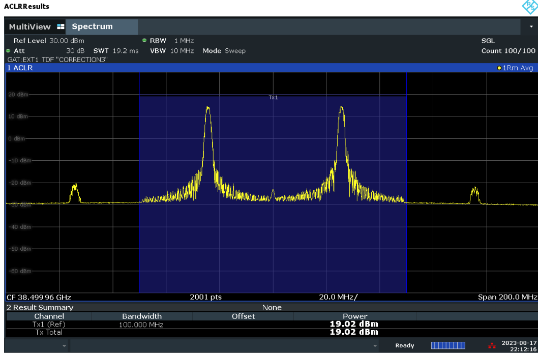
Plot 7-53. Conducted Power Plot – DFT-S – V-DL Polarization (50MHz-2CC – QPSK – Mid Ch. – 1 RB)
