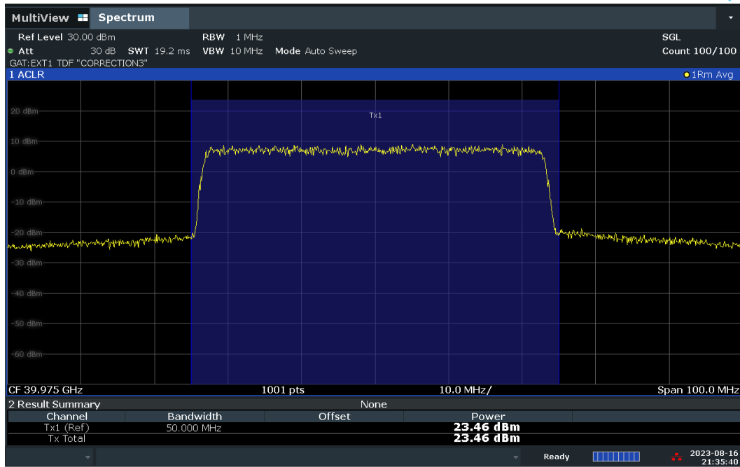
Plot 7-68. Conducted Power Plot – DFT-S – H-DL Polarization (50MHz-1CC – QPSK – High Ch. – Full RB)
