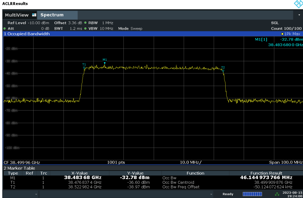
Plot 7-7. Occupied Bandwidth Input at 3dB above AGC Threshold – DFT-s – H-DL Polarization.
