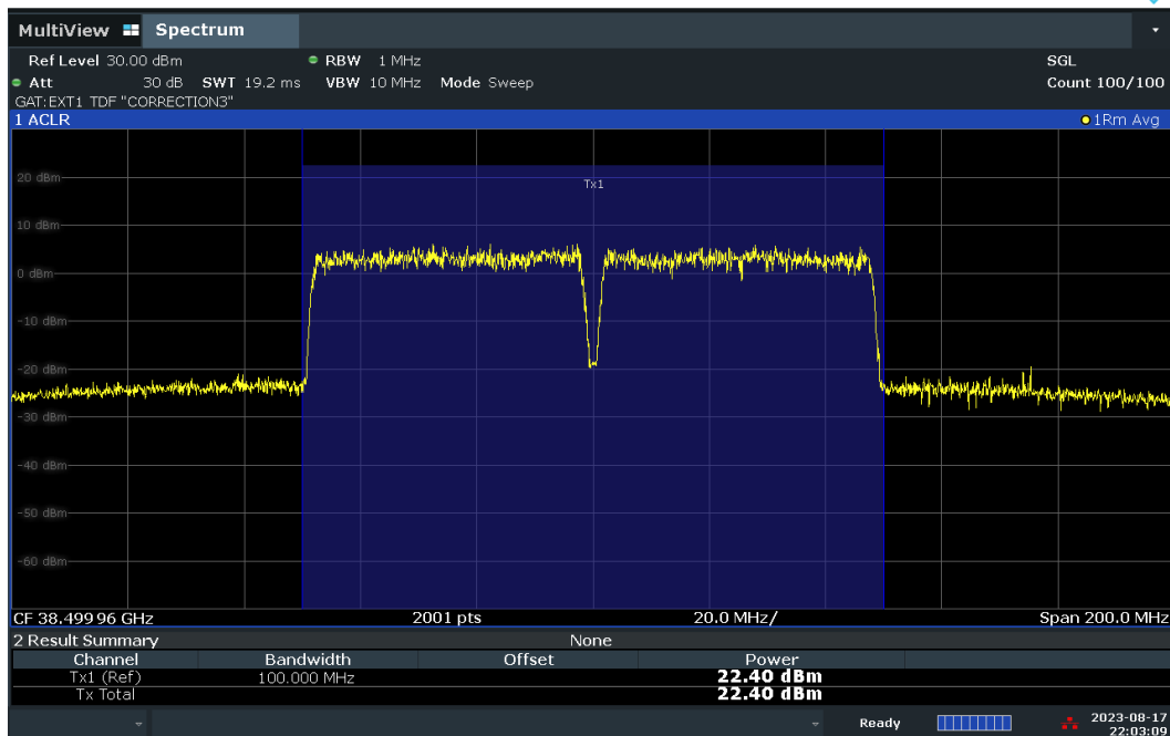
Plot 7-52. Conducted Power Plot – DFT-S – V-DL Polarization (50MHz-2CC – QPSK – Mid Ch. – Full RB)
