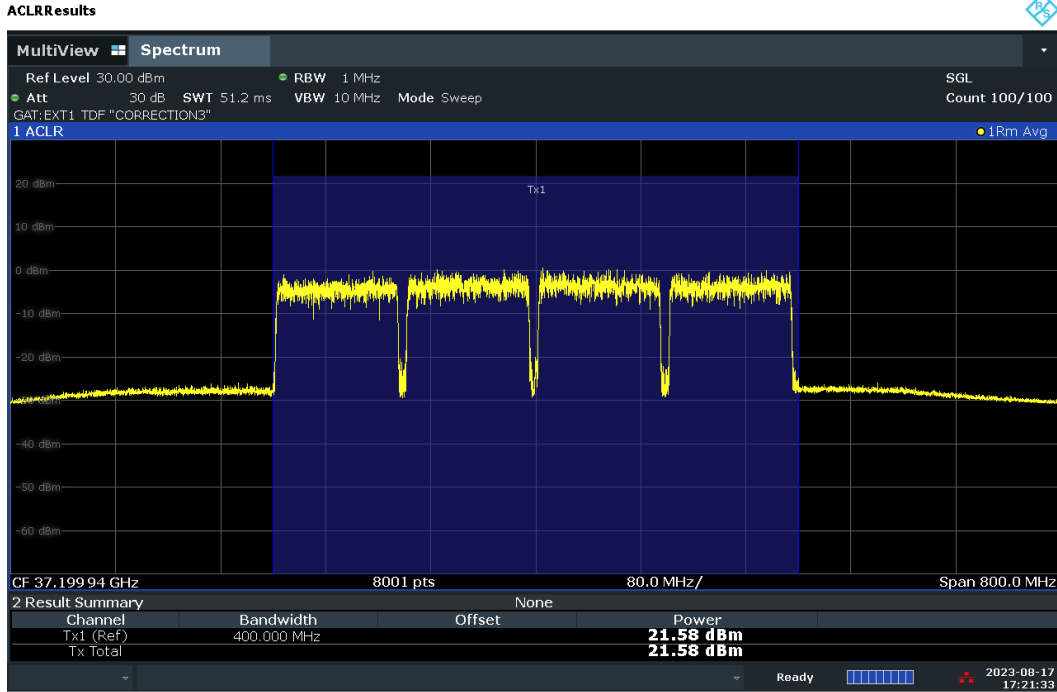
Plot 7-78. Conducted Power Plot – DFT-S – H-DL Polarization (100MHz-4CC – QPSK – Low Ch. – Full RB)
