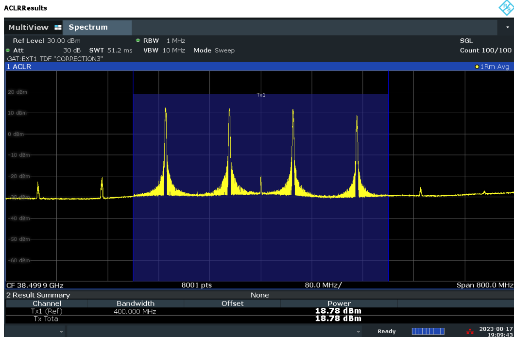
Plot 7-81. Conducted Power Plot – DFT-S – H-DL Polarization (100MHz-4CC – QPSK – Mid Ch. – 1 RB)
