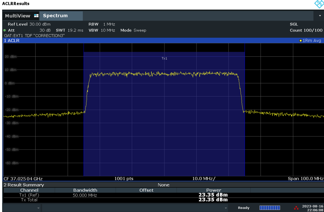
Plot 7-64. Conducted Power Plot – DFT-S – H-DL Polarization (50MHz-1CC – QPSK – Low Ch. – Full RB)
