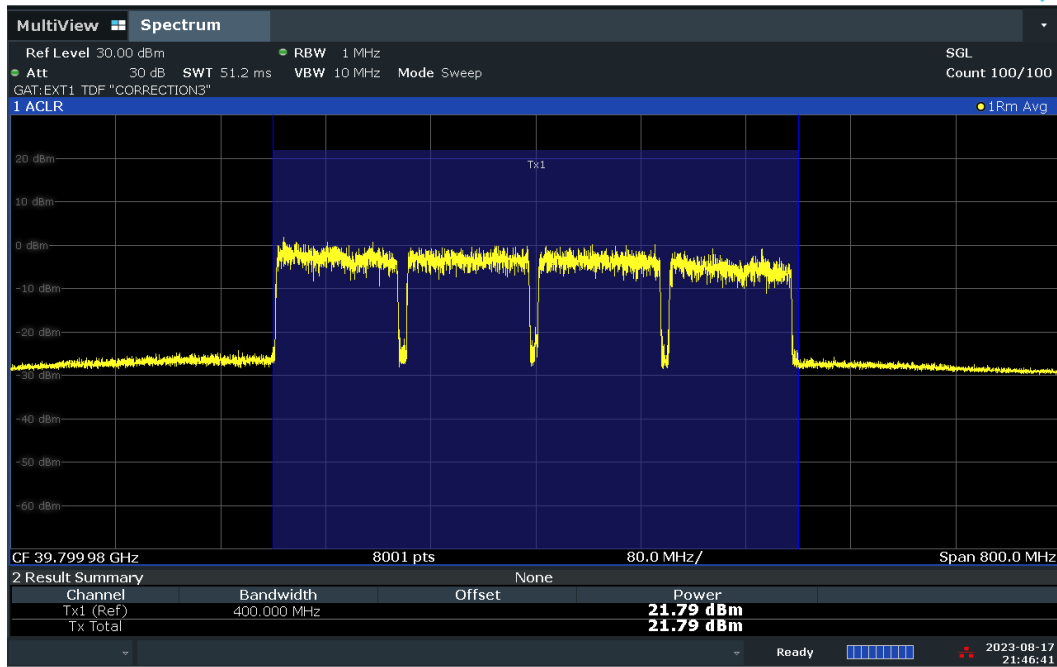
Plot 7-61. Conducted Power Plot – DFT-S – V-DL Polarization (100MHz-4CC – QPSK – High Ch. – Full RB)
