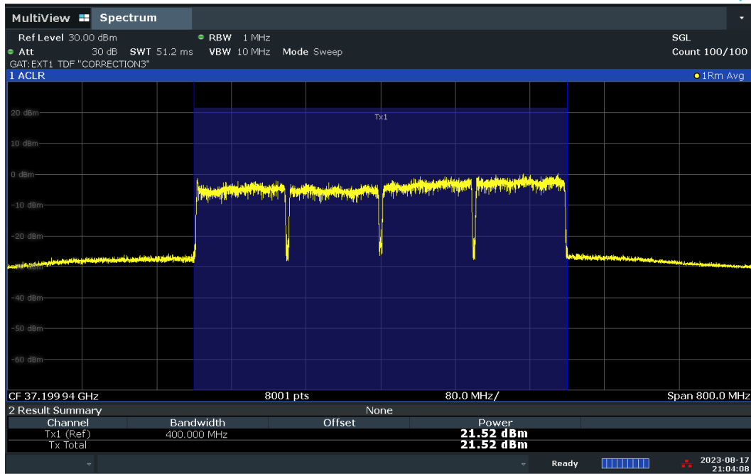
Plot 7-99. Conducted Power Plot – CP – V-DL Polarization (100MHz-4CC – QPSK – Low Ch. – Full RB)
