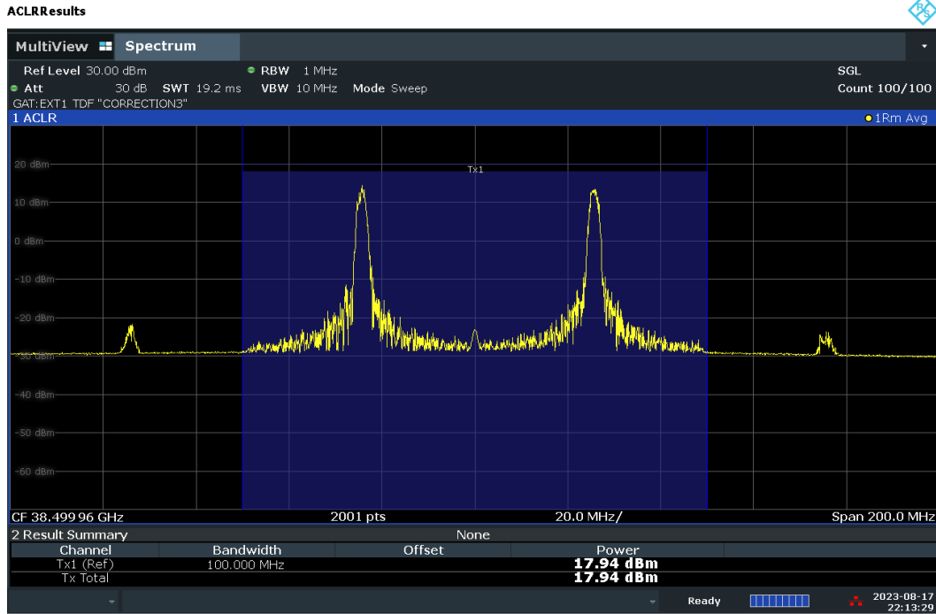
Plot 7-95. Conducted Power Plot – CP – V-DL Polarization (50MHz-2CC – QPSK – Mid Ch. – 1 RB)
