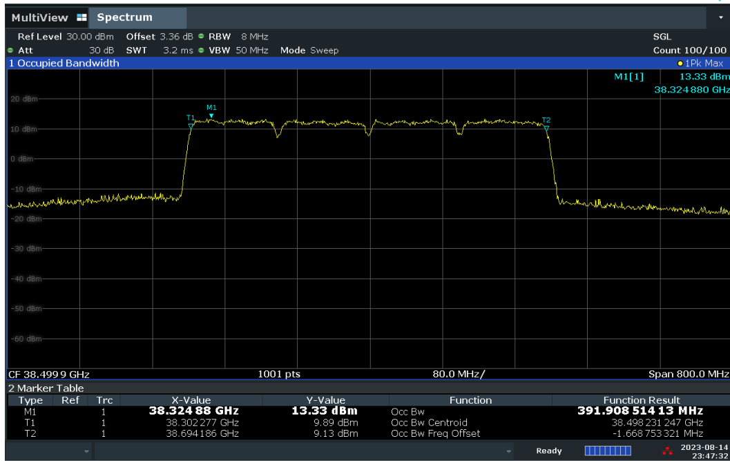
Plot 7-23. Occupied Bandwidth Plot – DFT-s – V-DL Polarization (100MHz-4CC – QPSK – Mid Channel)
