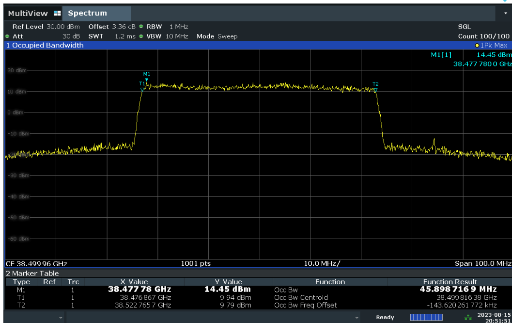
Plot 7-10. Occupied Bandwidth Output at 0.5dB below AGC Threshold – CP – V-DL Polarization.
