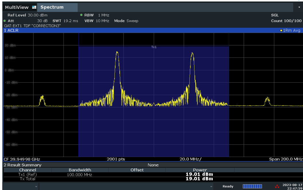
Plot 7-55. Conducted Power Plot – DFT-S – V-DL Polarization (50MHz-2CC – QPSK – High Ch. – 1 RB)
