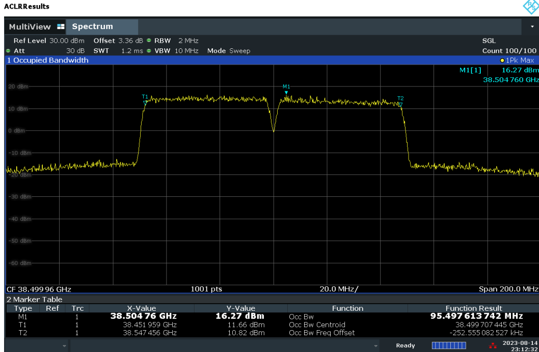
Plot 7-27. Occupied Bandwidth Plot – DFT-s – H-DL Polarization (50MHz-2CC – QPSK – Mid Channel)
