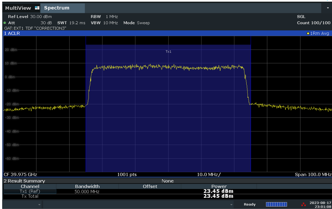
Plot 7-47. Conducted Power Plot – DFT-S – V-DL Polarization (50MHz-1CC – QPSK – High Ch. – Full RB)
