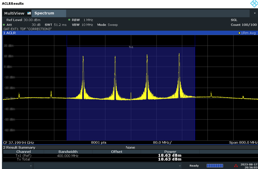
Plot 7-58. Conducted Power Plot – DFT-S – V-DL Polarization (100MHz-4CC – QPSK – Low Ch. – 1RB)
