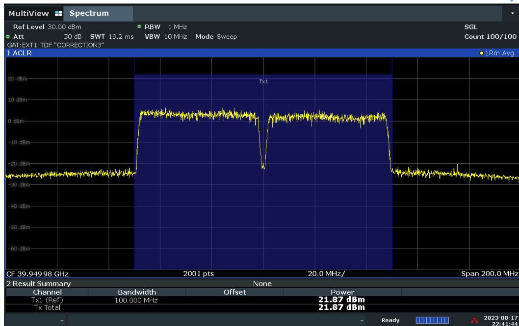
Plot 7-56. Conducted Power Plot – DFT-S – V-DL Polarization (50MHz-2CC – 16QAM – High Ch. – Full RB)
