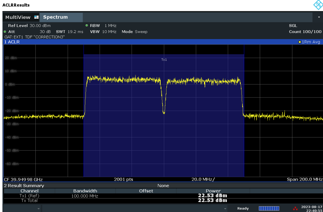
Plot 7-54. Conducted Power Plot – DFT-S – V-DL Polarization (50MHz-2CC – QPSK – High Ch. – Full RB)
