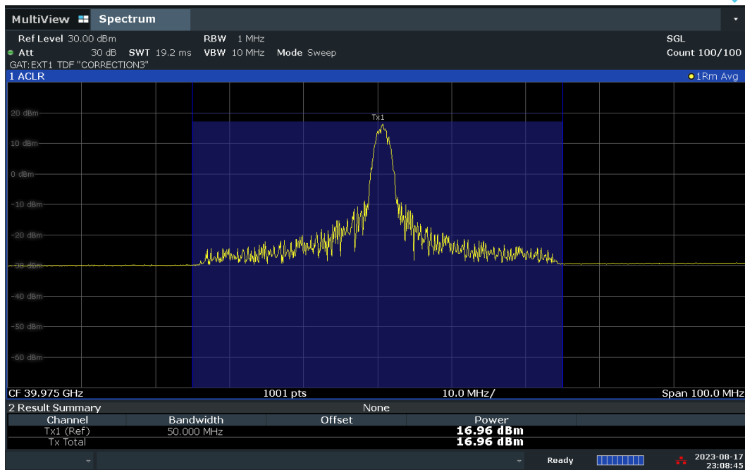
Plot 7-90. Conducted Power Plot – CP – V-DL Polarization (50MHz-1CC – QPSK – High Ch. – 1 RB)
