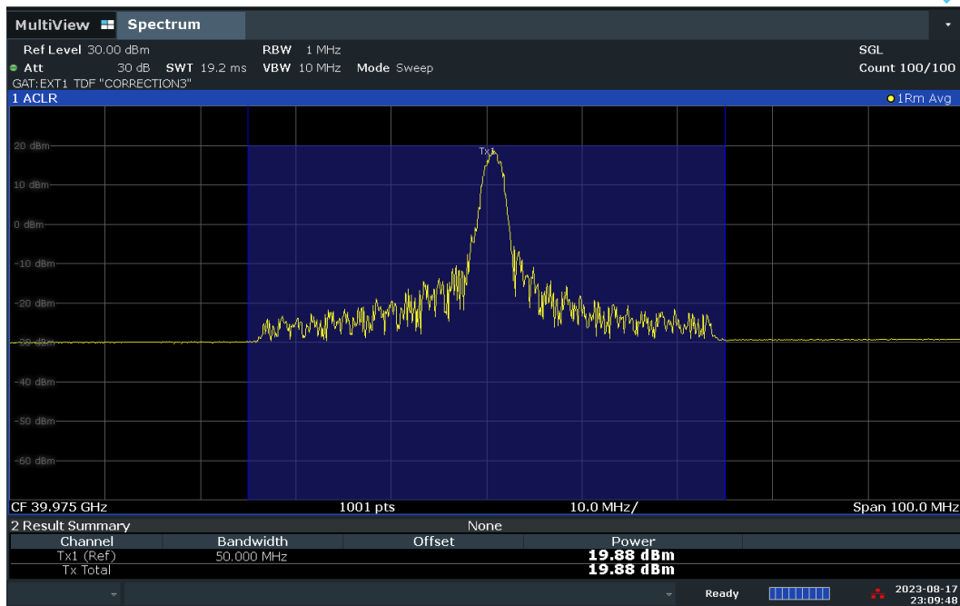
Plot 7-48. Conducted Power Plot – DFT-S – V-DL Polarization (50MHz-1CC – QPSK – High Ch. – 1 RB)
