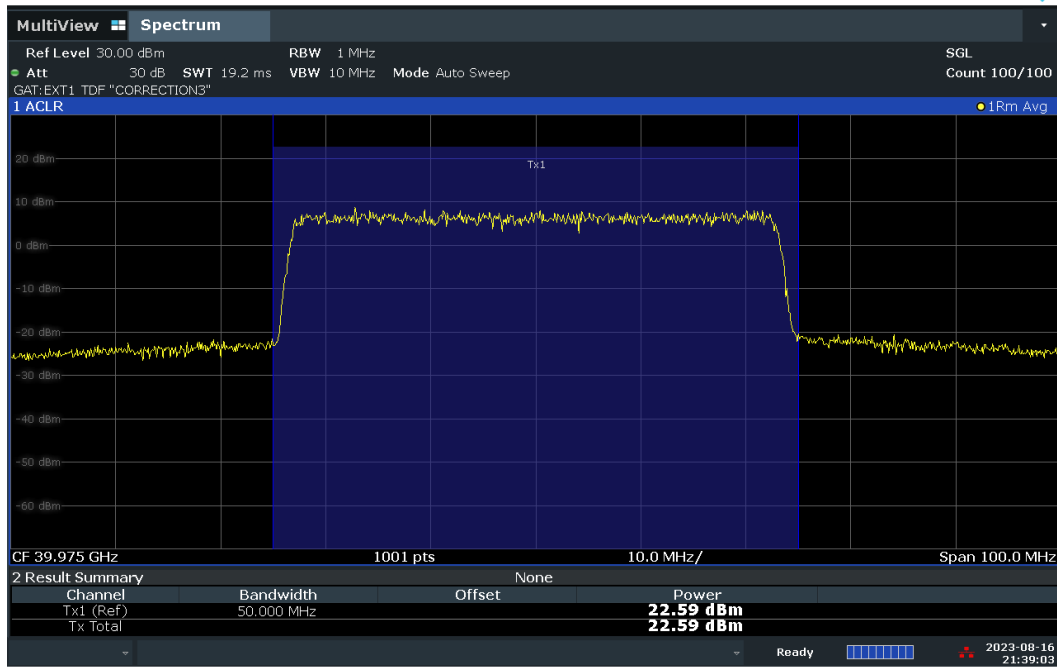
Plot 7-70. Conducted Power Plot – DFT-S – H-DL Polarization (50MHz-1CC – 16QAM – High Ch. – Full RB)
