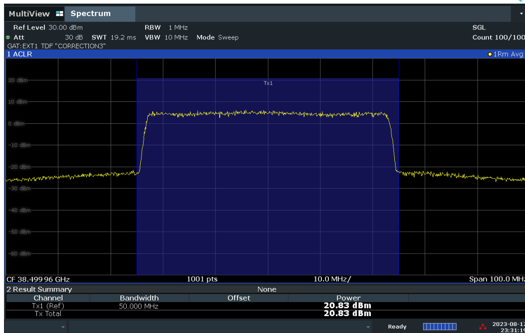
Plot 7-91. Conducted Power Plot – CP – V-DL Polarization (50MHz-1CC – 16QAM – Mid Ch. – Full RB)
