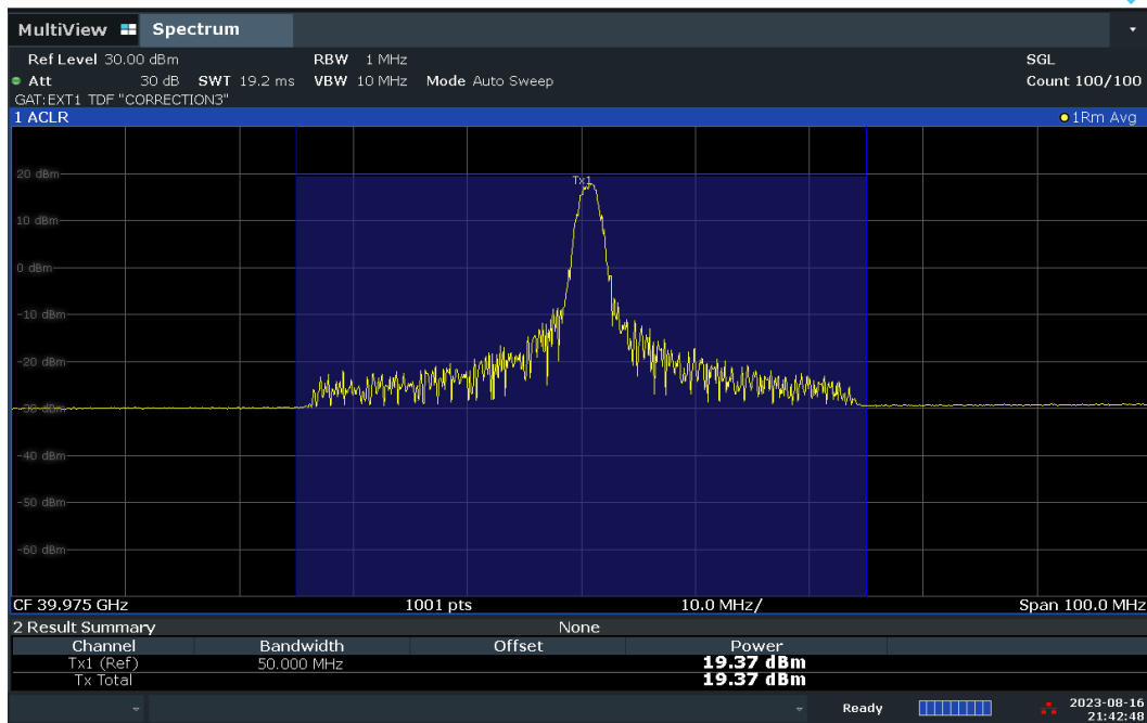
Plot 7-69. Conducted Power Plot – DFT-S – H-DL Polarization (50MHz-1CC – QPSK – High Ch. – 1 RB)
