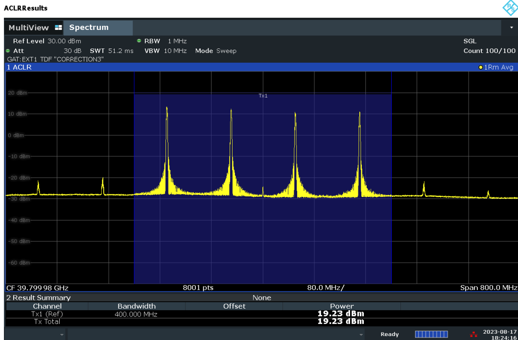
Plot 7-83. Conducted Power Plot – DFT-S – H-DL Polarization (100MHz-4CC – QPSK – High Ch. – 1 RB)
