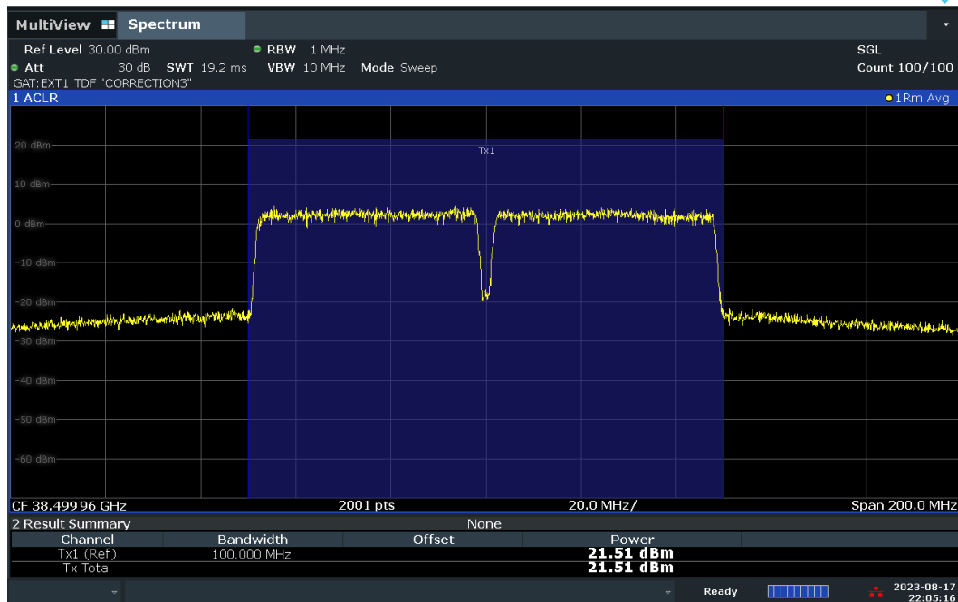
Plot 7-98. Conducted Power Plot – CP – V-DL Polarization (50MHz-2CC – 16QAM – Mid Ch. – Full RB)
