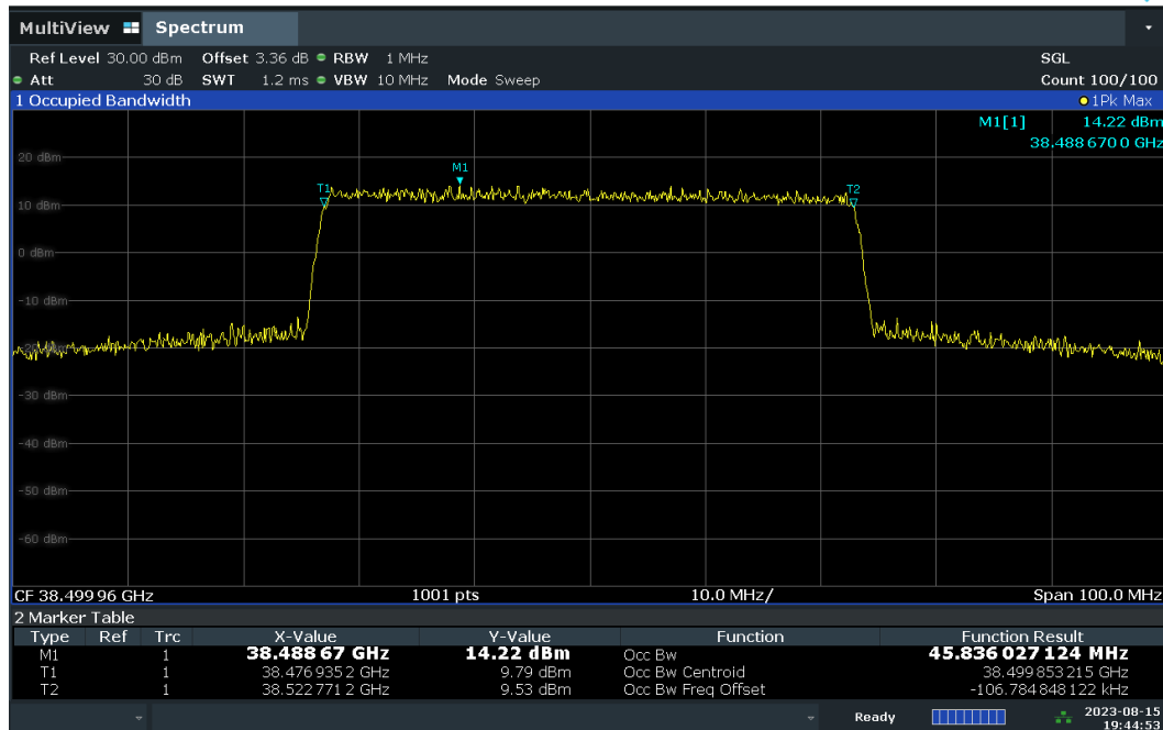
Plot 7-14. Occupied Bandwidth Output at 0.5dB below AGC Threshold – CP – H-DL Polarization.
