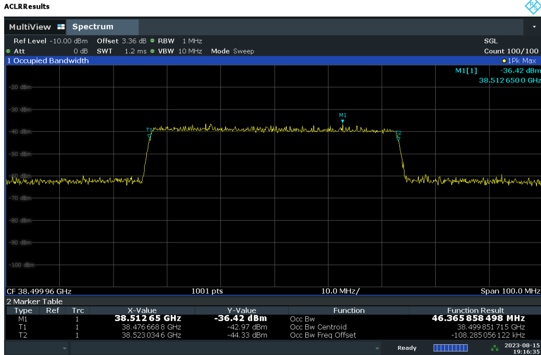
Plot 7-5. Occupied Bandwidth Input at 0.5dB below AGC Threshold – DFT-s – H-DL Polarization.
