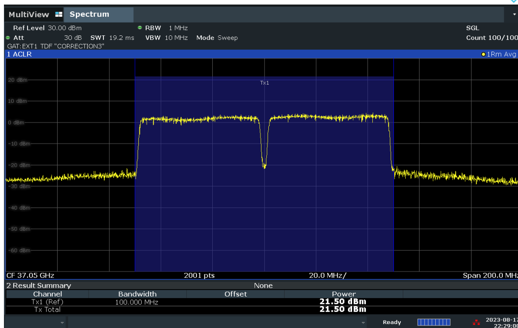
Plot 7-92. Conducted Power Plot – CP – V-DL Polarization (50MHz-2CC – QPSK – Low Ch. – Full RB)
