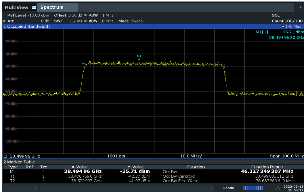
Plot 7-9. Occupied Bandwidth Input at 0.5dB below AGC Threshold – CP – V-DL Polarization.
