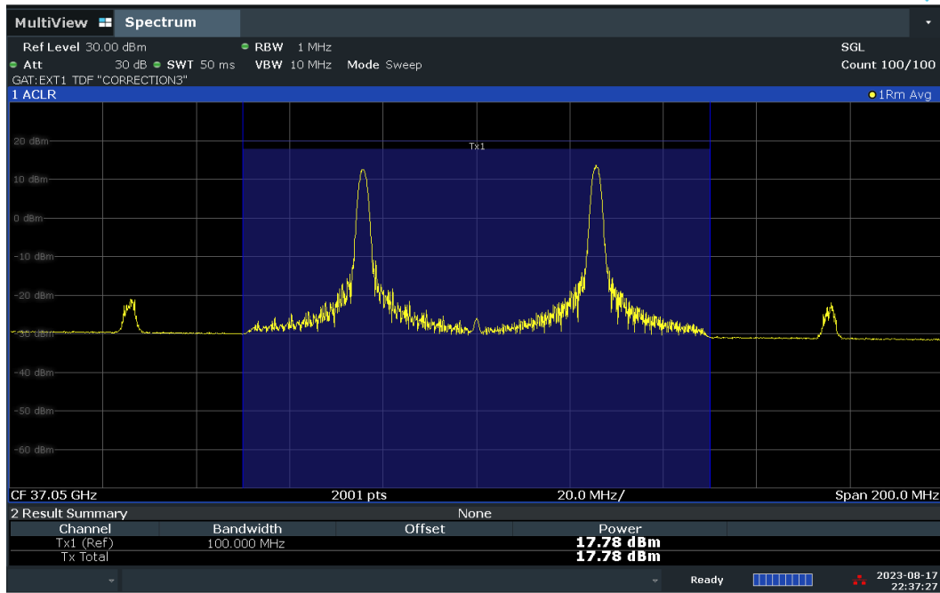
Plot 7-93. Conducted Power Plot – CP – V-DL Polarization (50MHz-2CC – QPSK – Low Ch. – 1RB)
