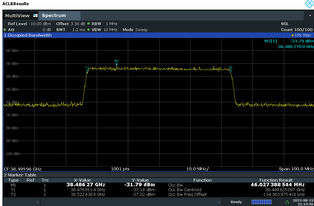
Plot 7-3. Occupied Bandwidth Input at 3dB above AGC Threshold – DFT-s – V-DL Polarization.
