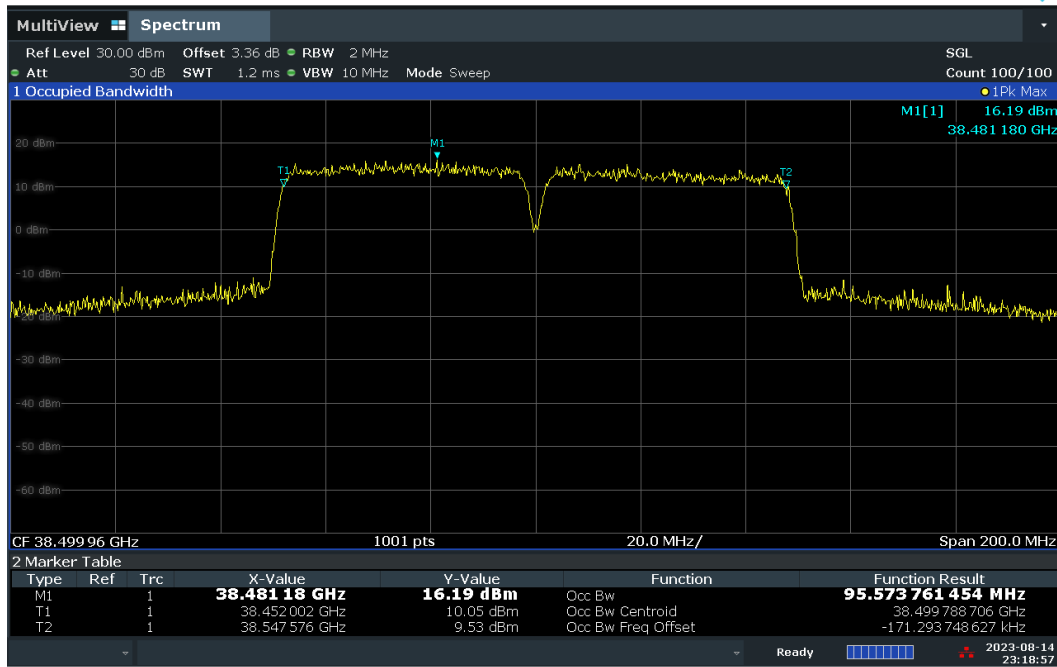
Plot 7-39. Occupied Bandwidth Plot – CP – H-DL Polarization (50MHz-2CC – QPSK – Mid Channel)
