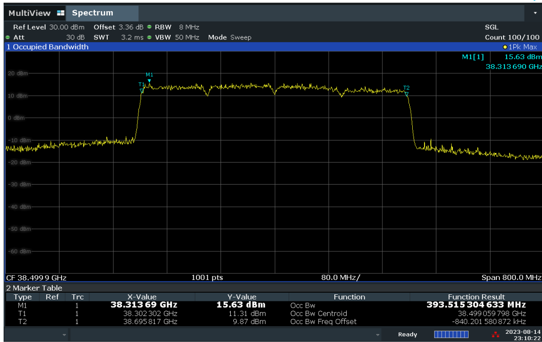
Plot 7-41. Occupied Bandwidth Plot – CP – H-DL Polarization (100MHz-4CC – QPSK – Mid Channel)
