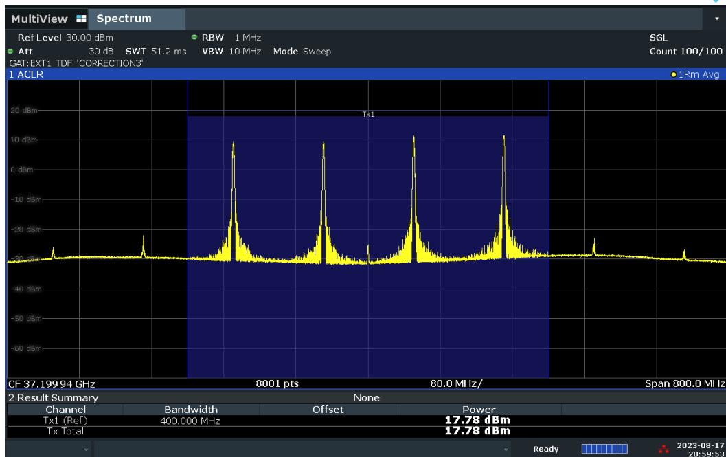
Plot 7-100. Conducted Power Plot – CP – V-DL Polarization (100MHz-4CC – QPSK – Low Ch. – 1RB)
