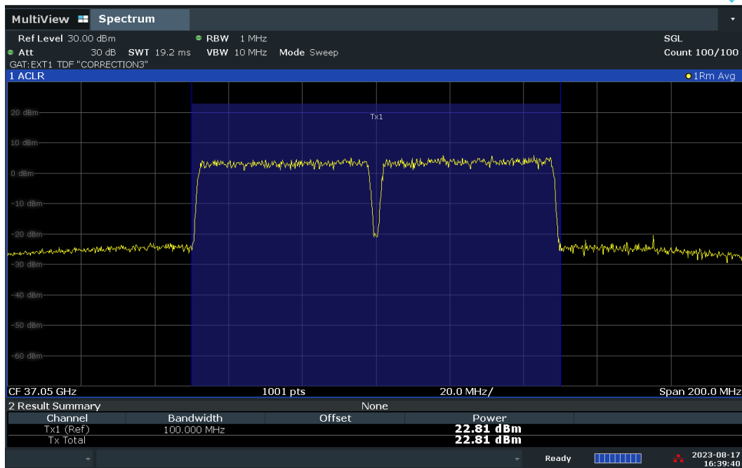
Plot 7-71. Conducted Power Plot – DFT-S – H-DL Polarization (50MHz-2CC – QPSK – Low Ch. – Full RB)
