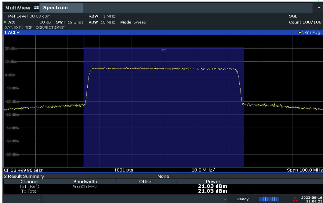
Plot 7-108. Conducted Power Plot – CP – H-DL Polarization (50MHz-1CC – QPSK – Mid Ch. – Full RB)
