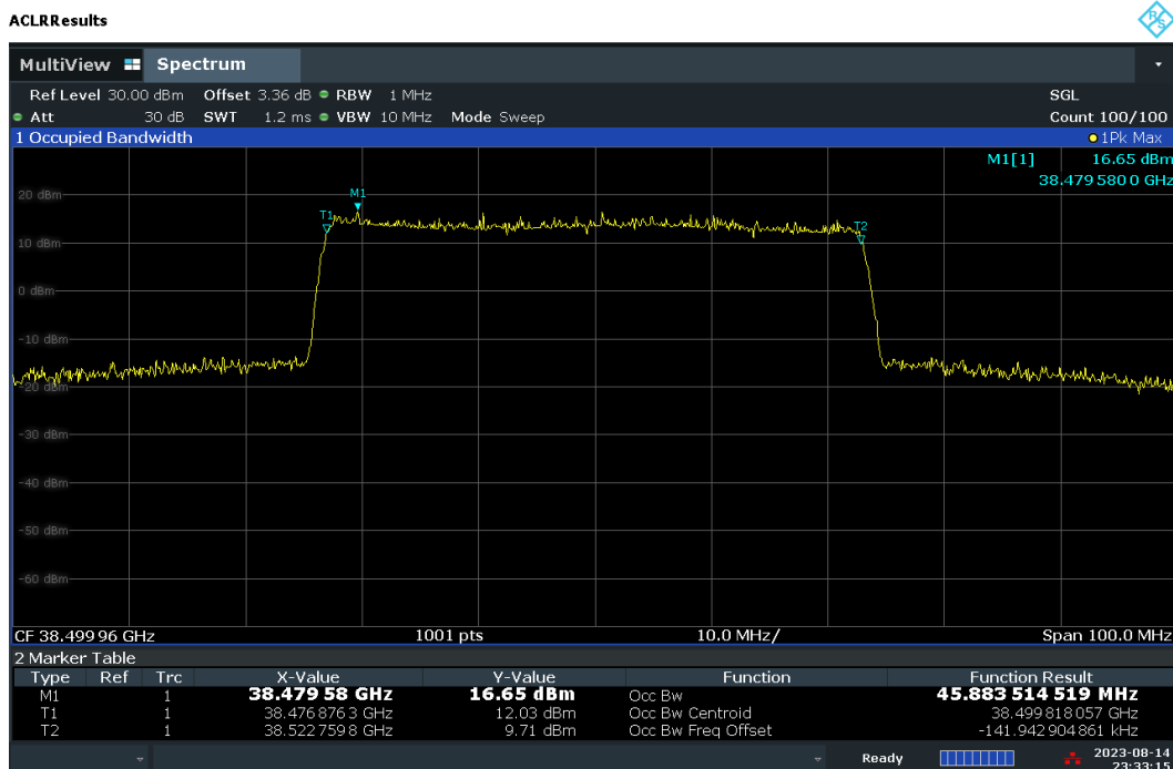
Plot 7-20. Occupied Bandwidth Plot – DFT-s – V-DL Polarization (50MHz-1CC – 16QAM – Mid Channel)
