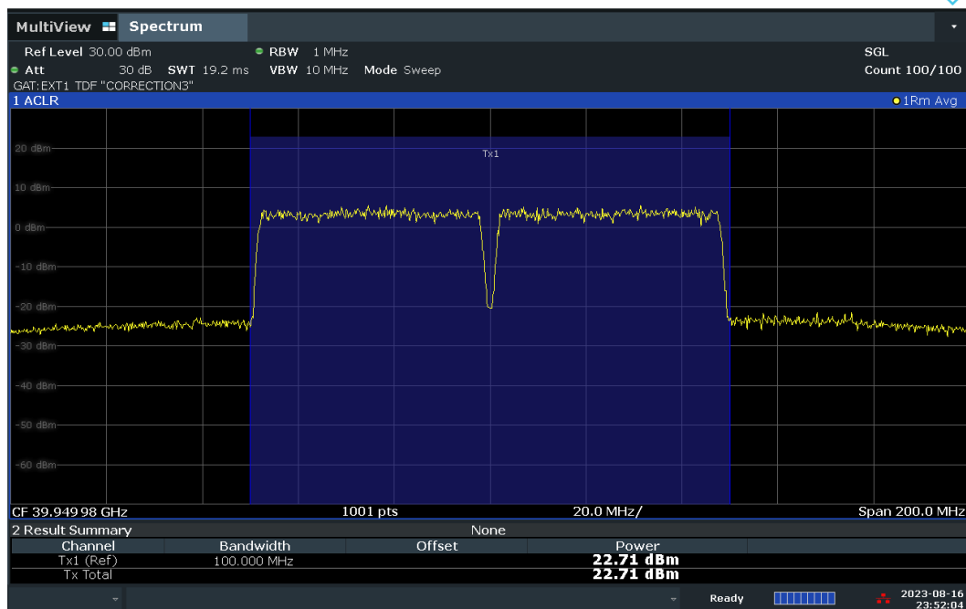
Plot 7-75. Conducted Power Plot – DFT-S – H-DL Polarization (50MHz-2CC – QPSK – High Ch. – Full RB)
