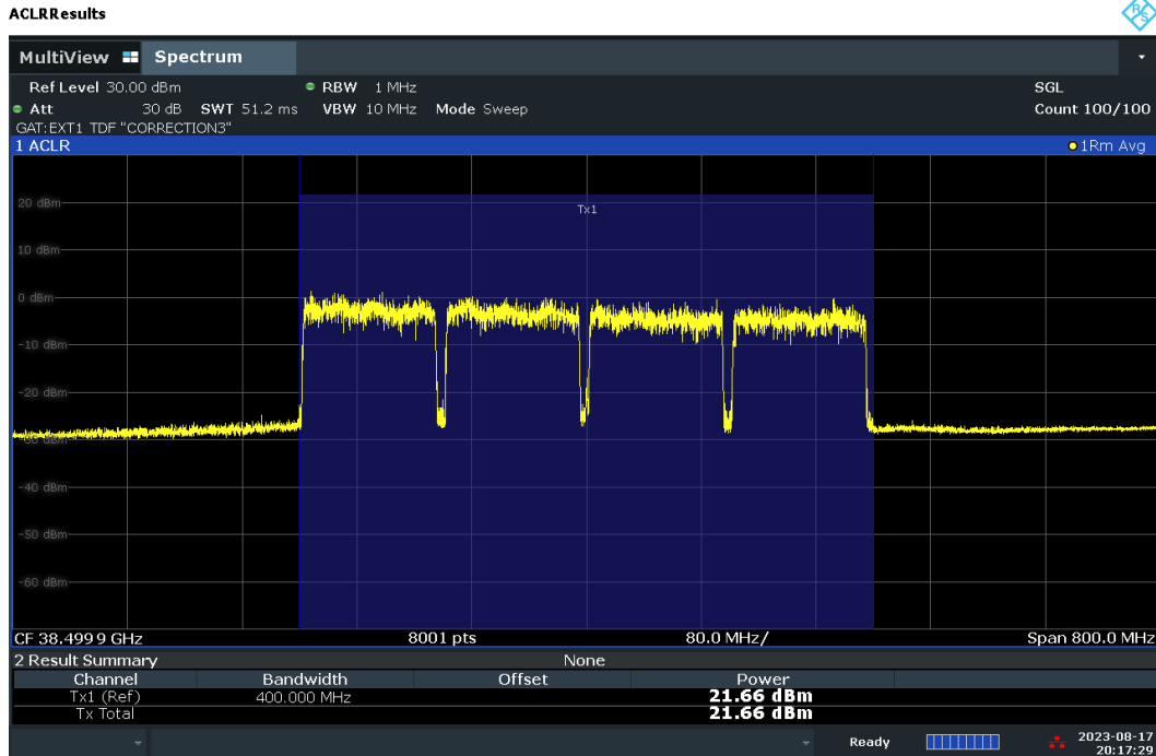
Plot 7-59. Conducted Power Plot – DFT-S – V-DL Polarization (100MHz-4CC – QPSK – Mid Ch. – Full RB)
