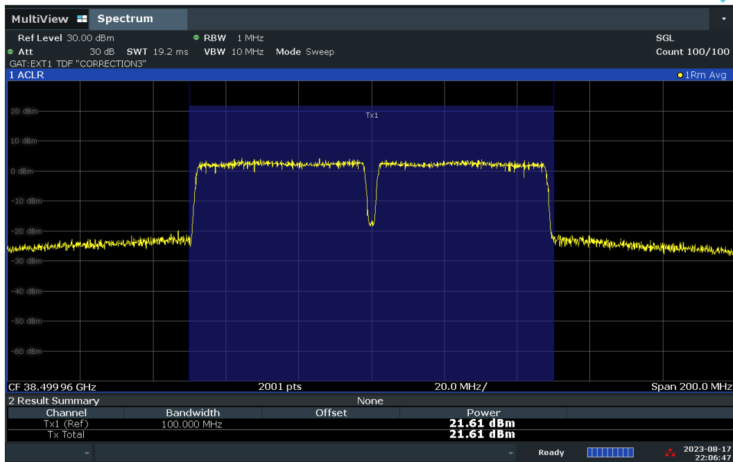
Plot 7-94. Conducted Power Plot – CP – V-DL Polarization (50MHz-2CC – QPSK – Mid Ch. – Full RB)
