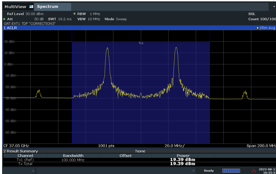
Plot 7-72. Conducted Power Plot – DFT-S – H-DL Polarization (50MHz-2CC – QPSK – Low Ch. – 1RB)
