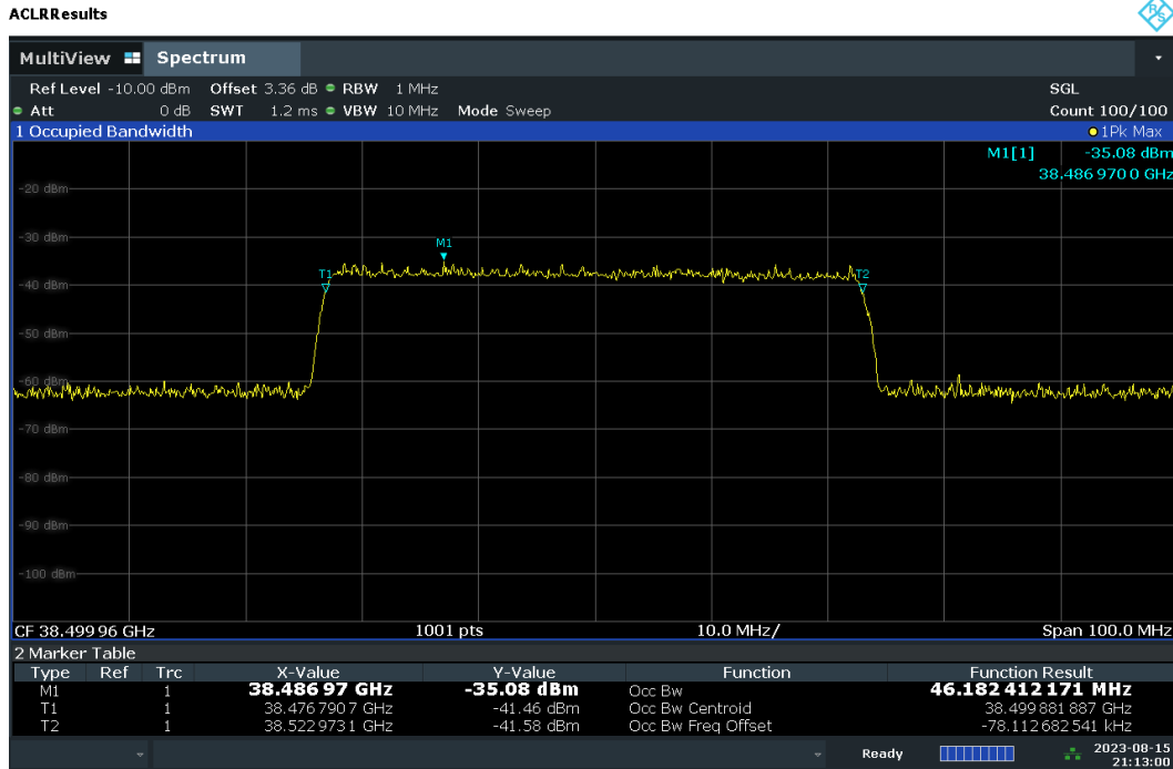
Plot 7-1. Occupied Bandwidth Input at 0.5dB below AGC Threshold – DFT-s – V-DL Polarization.
