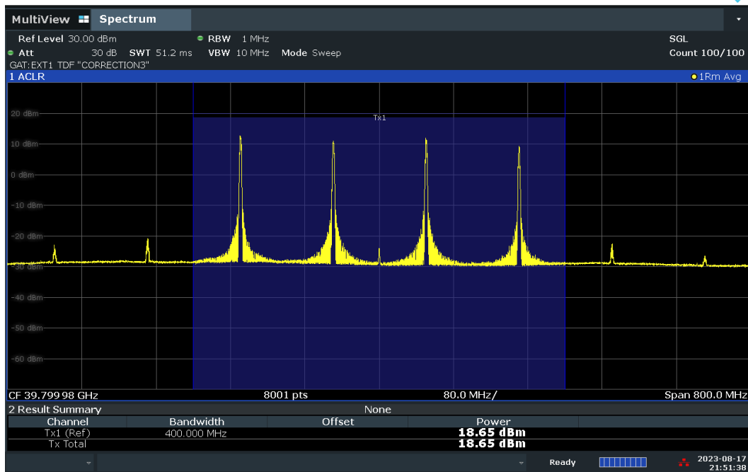
Plot 7-62. Conducted Power Plot – DFT-S – V-DL Polarization (100MHz-4CC – QPSK – High Ch. – 1 RB)
