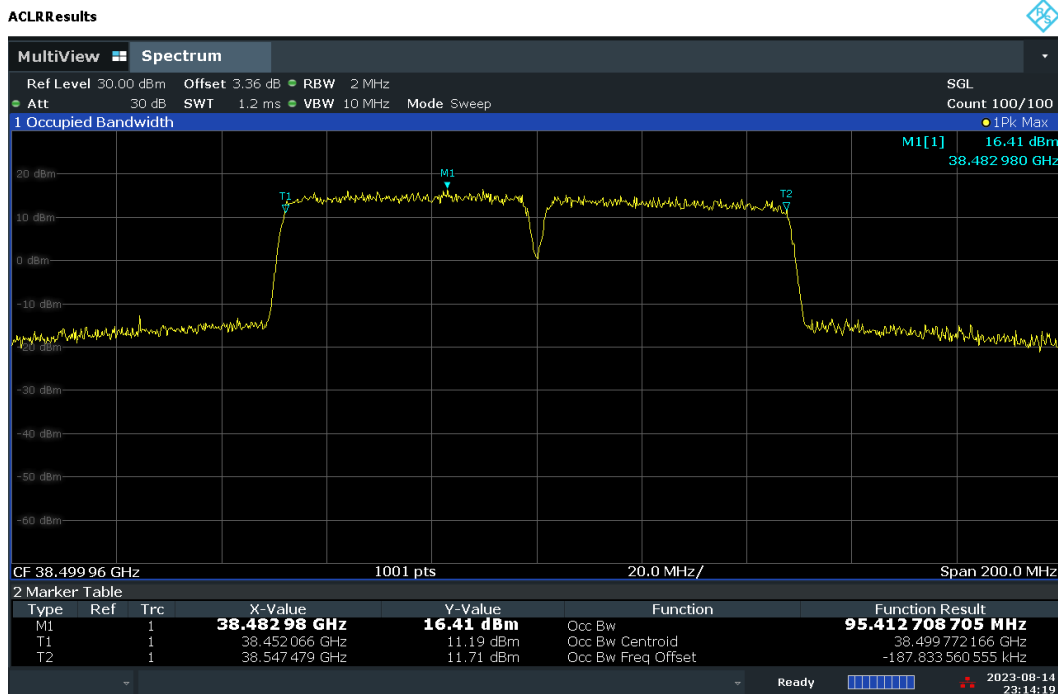
Plot 7-28. Occupied Bandwidth Plot – DFT-s – H-DL Polarization (50MHz-2CC – 16QAM – Mid Channel)
