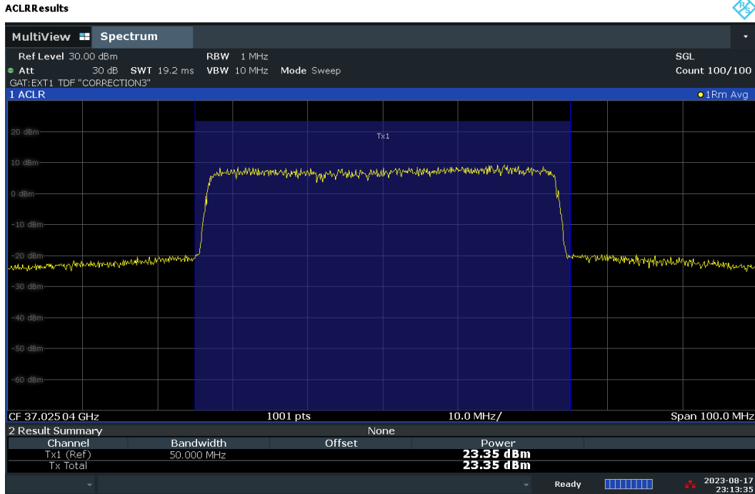
Plot 7-43. Conducted Power Plot – DFT-S – V-DL Polarization (50MHz-1CC – QPSK – Low Ch. – Full RB)
