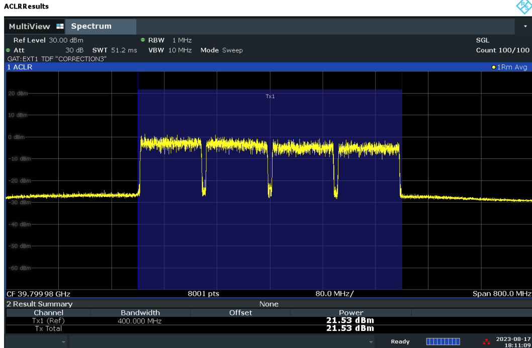
Plot 7-84. Conducted Power Plot – DFT-S – H-DL Polarization (100MHz-4CC – 16QAM – High Ch. – Full RB)
