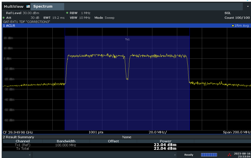
Plot 7-77. Conducted Power Plot – DFT-S – H-DL Polarization (50MHz-2CC – 16QAM – High Ch. – Full RB)
