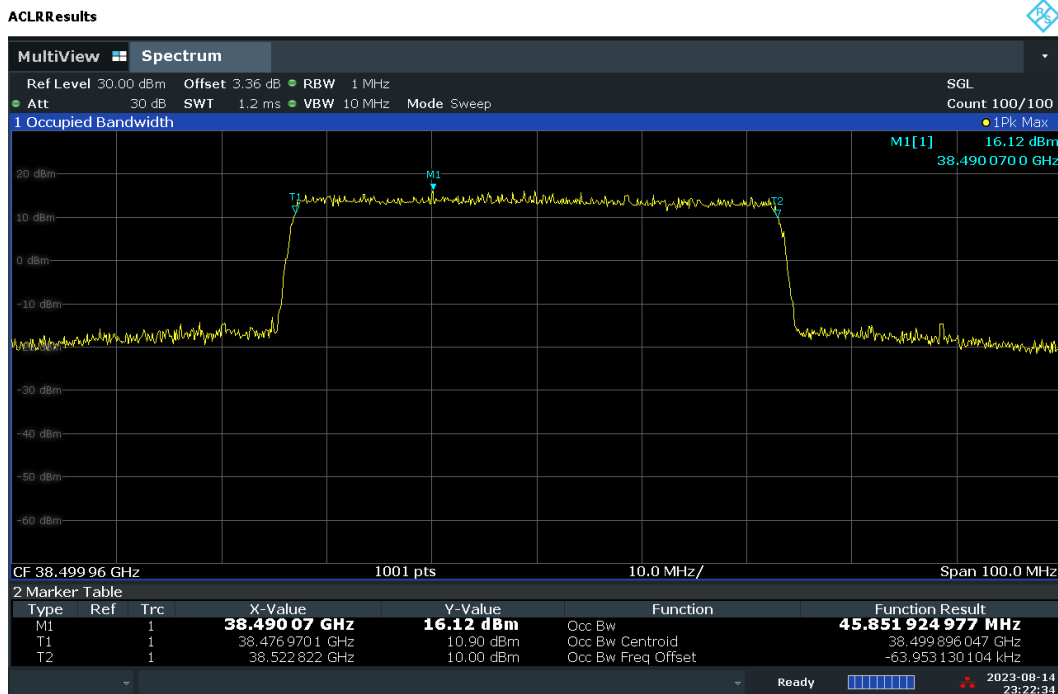
Plot 7-26. Occupied Bandwidth Plot – DFT-s – H-DL Polarization (50MHz-1CC – 16QAM – Mid Channel)
