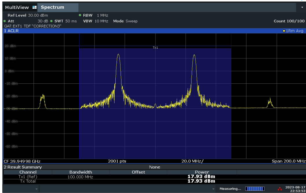
Plot 7-97. Conducted Power Plot – CP – V-DL Polarization (50MHz-2CC – QPSK – High Ch. – 1 RB)
