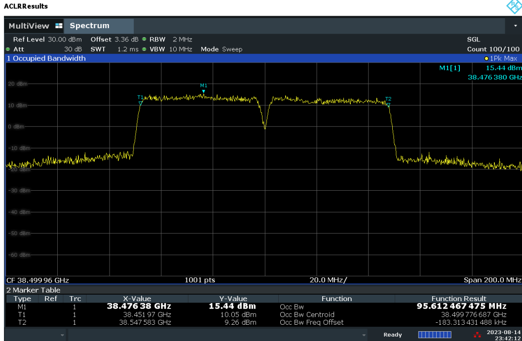
Plot 7-33. Occupied Bandwidth Plot – CP – V-DL Polarization (50MHz-2CC – QPSK – Mid Channel)
