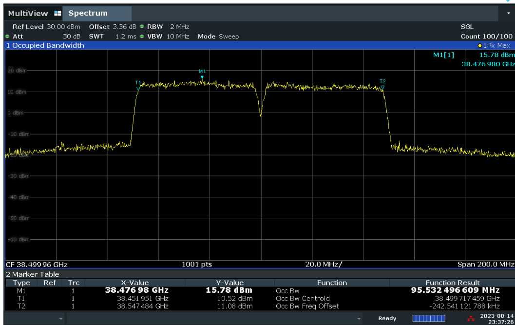
Plot 7-22. Occupied Bandwidth Plot – DFT-s – V-DL Polarization (50MHz-2CC – 16QAM – Mid Channel)
