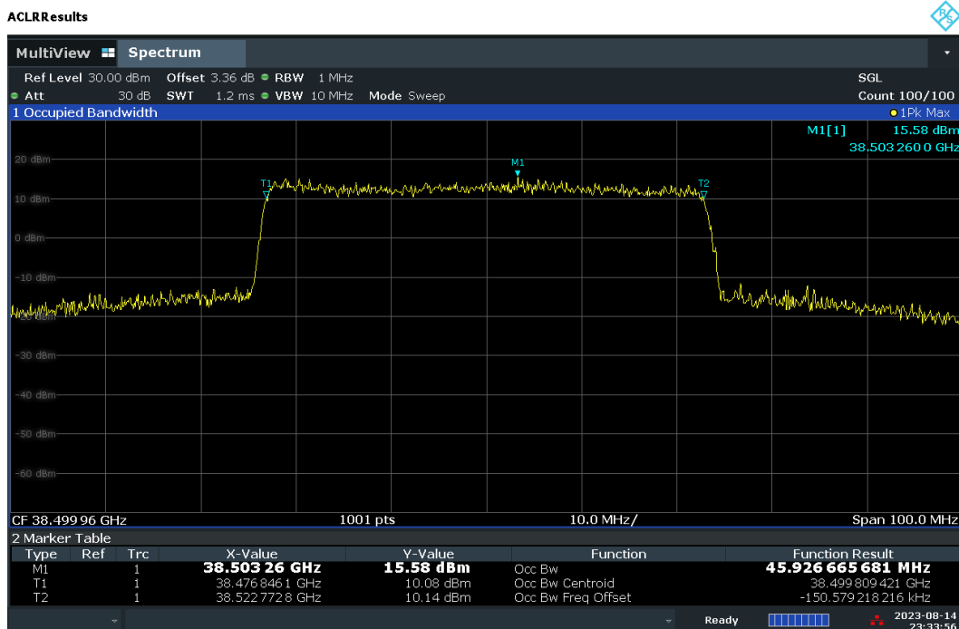
Plot 7-32. Occupied Bandwidth Plot – CP – V-DL Polarization (50MHz-1CC – 16QAM – Mid Channel)
