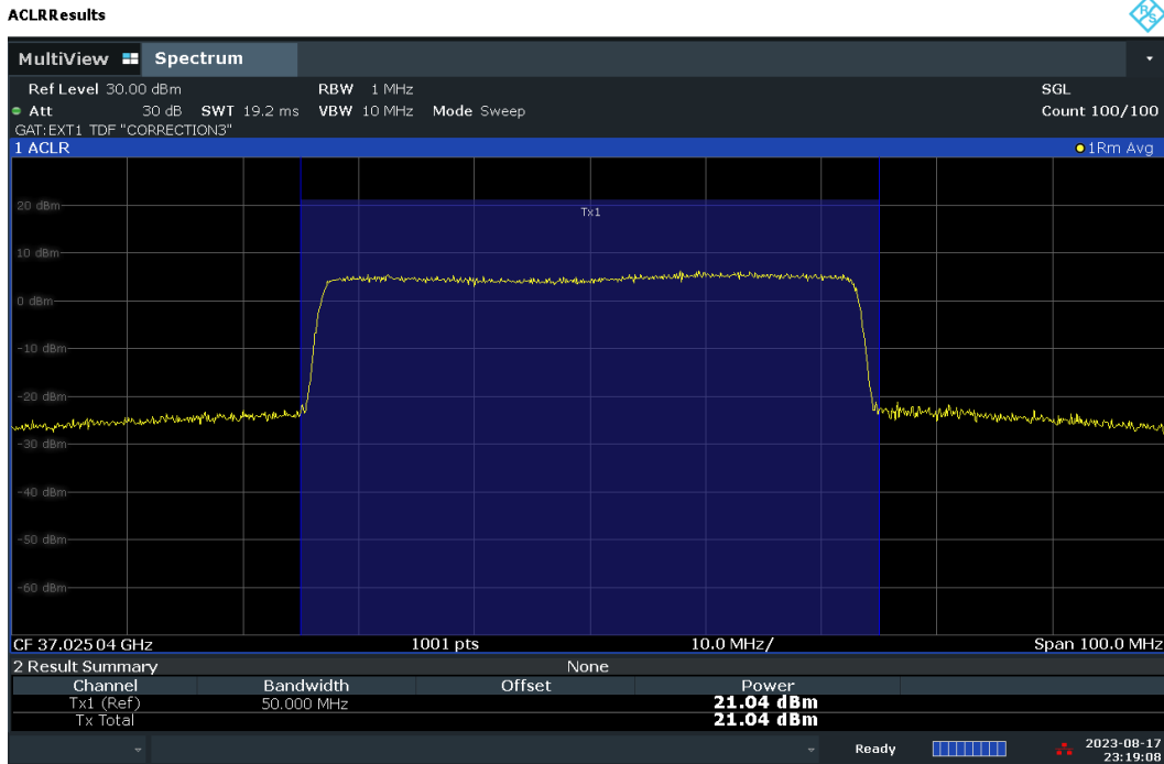
Plot 7-85. Conducted Power Plot – CP – V-DL Polarization (50MHz-1CC – QPSK – Low Ch. – Full RB)
