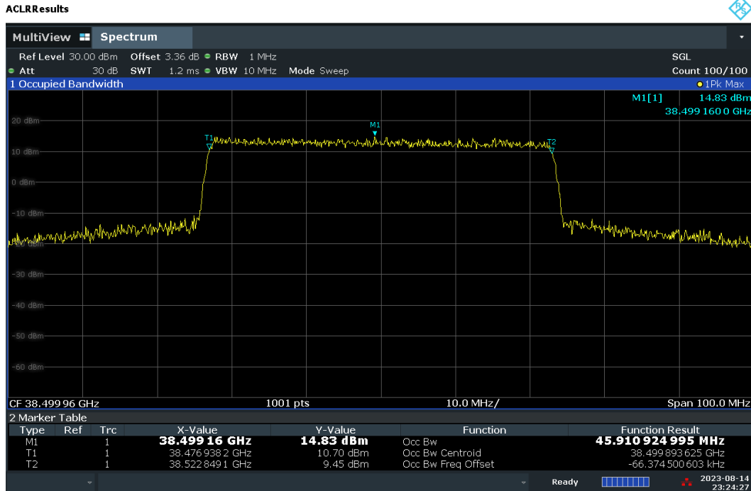
Plot 7-37. Occupied Bandwidth Plot – CP – H-DL Polarization (50MHz-1CC – QPSK – Mid Channel)
