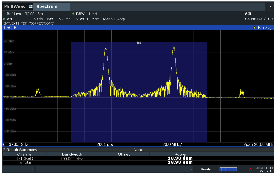
Plot 7-51. Conducted Power Plot – DFT-S – V-DL Polarization (50MHz-2CC – QPSK – Low Ch. – 1RB)
