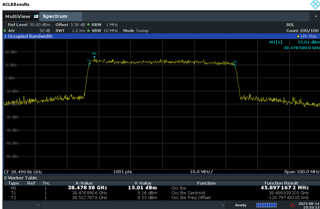
Plot 7-31. Occupied Bandwidth Plot – CP – V-DL Polarization (50MHz-1CC – QPSK – Mid Channel)
