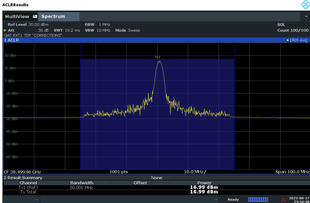
Plot 7-88. Conducted Power Plot – CP – V-DL Polarization (50MHz-1CC – QPSK – Mid Ch. – 1 RB)
