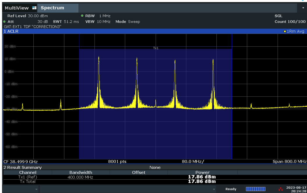
Plot 7-102. Conducted Power Plot – CP – V-DL Polarization (100MHz-4CC – QPSK – Mid Ch. – 1 RB)
