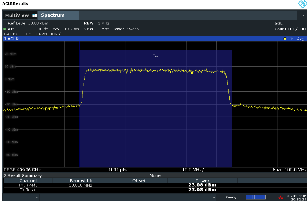
Plot 7-66. Conducted Power Plot – DFT-S – H-DL Polarization (50MHz-1CC – QPSK – Mid Ch. – Full RB)
