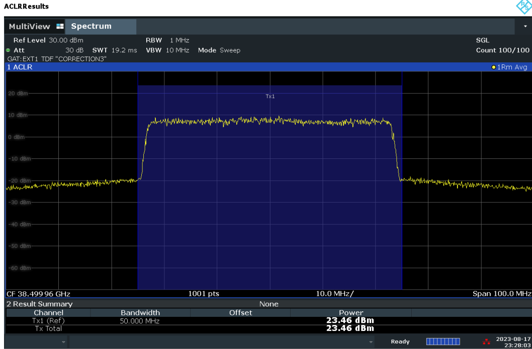
Plot 7-45. Conducted Power Plot – DFT-S – V-DL Polarization (50MHz-1CC – QPSK – Mid Ch. – Full RB)
