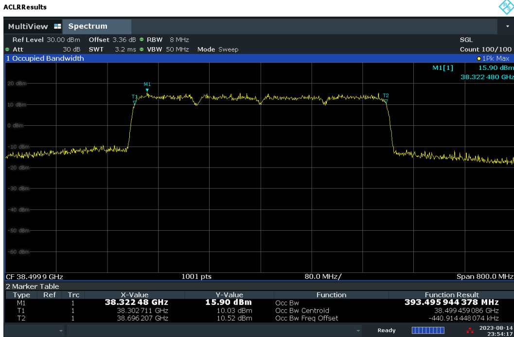
Plot 7-36. Occupied Bandwidth Plot – CP – V-DL Polarization (100MHz-4CC – 16QAM – Mid Channel)
