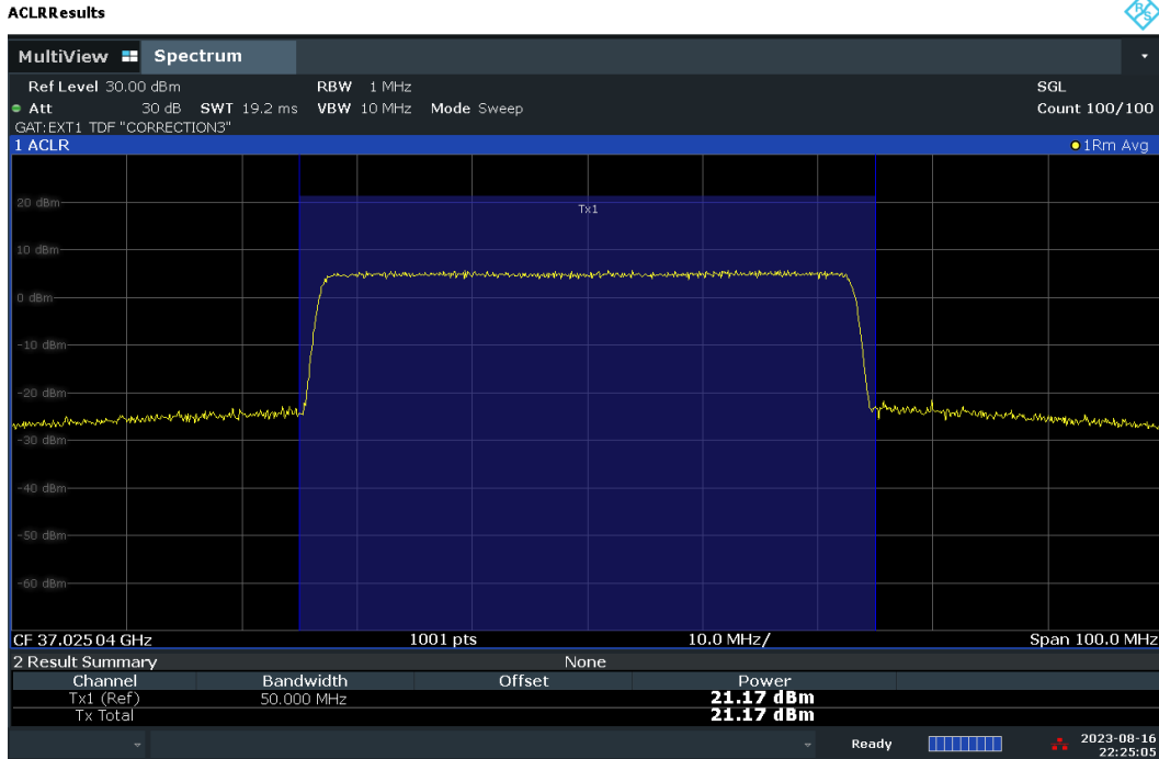
Plot 7-106. Conducted Power Plot – CP – H-DL Polarization (50MHz-1CC – QPSK – Low Ch. – Full RB)
