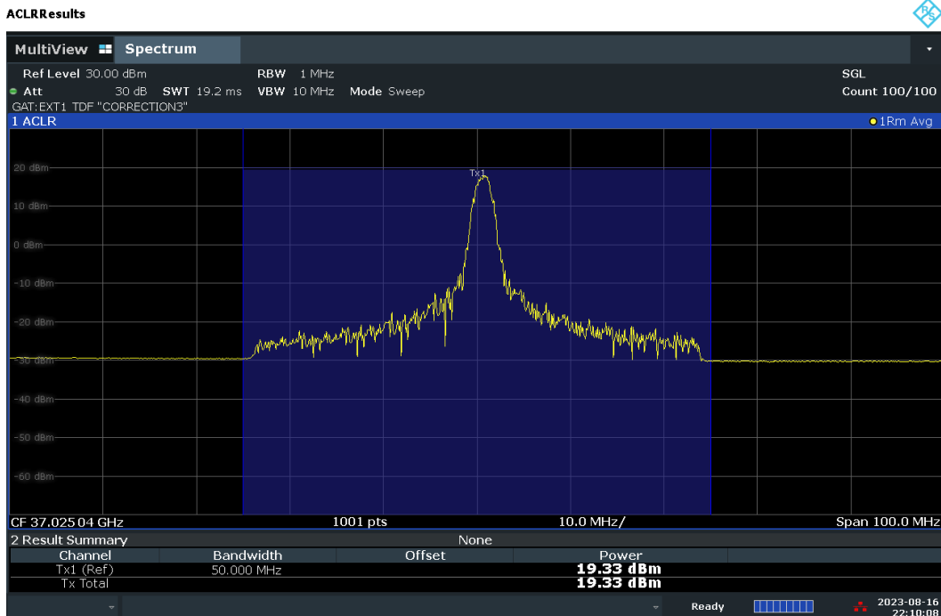
Plot 7-65. Conducted Power Plot – DFT-S – H-DL Polarization (50MHz-1CC – QPSK – Low Ch. – 1RB)
