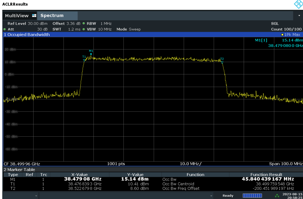
Plot 7-11. Occupied Bandwidth Input at 3dB above AGC Threshold – CP – V-DL Polarization.
