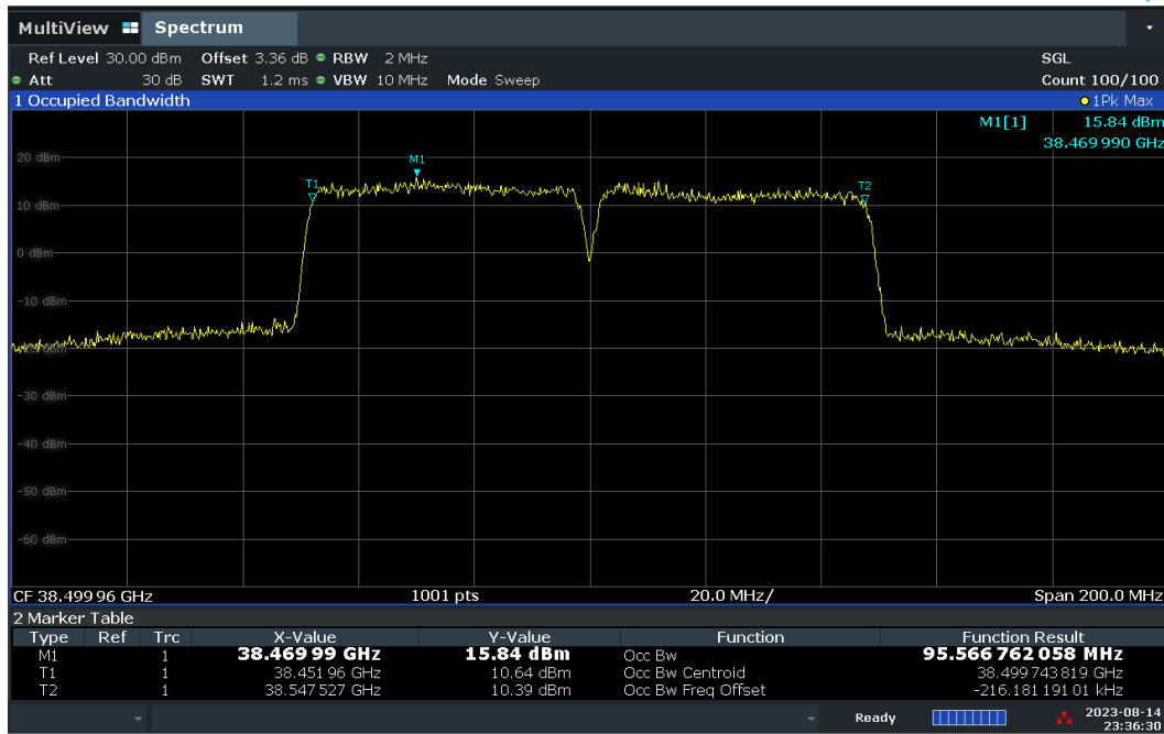
Plot 7-21. Occupied Bandwidth Plot – DFT-s – V-DL Polarization (50MHz-2CC – QPSK – Mid Channel)
