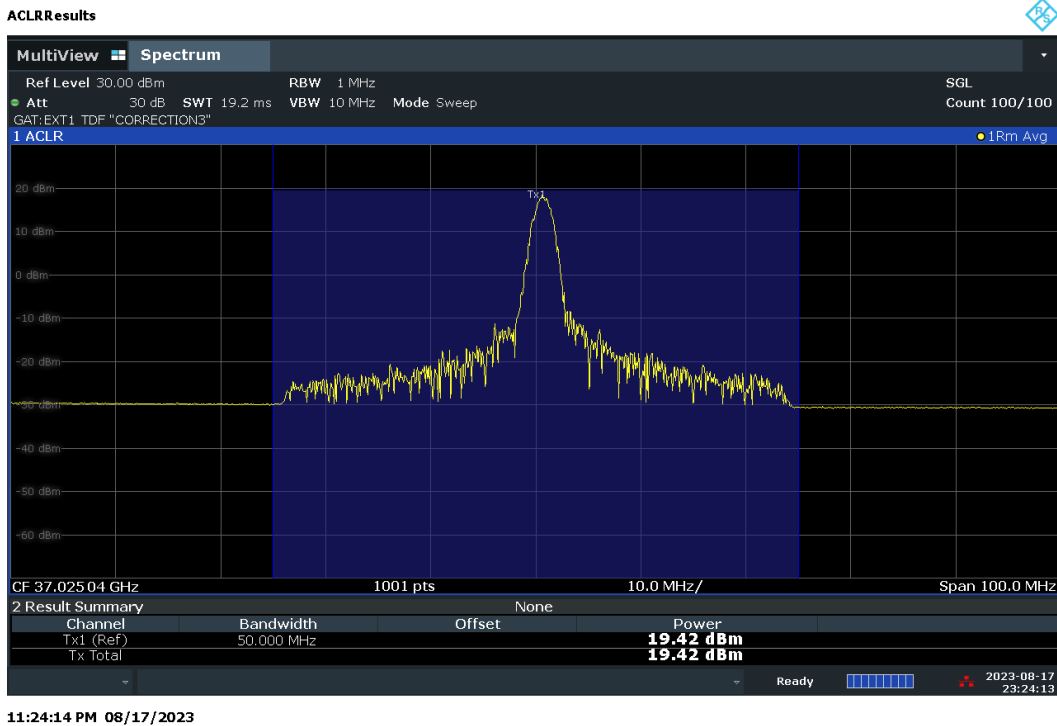
Plot 7-44. Conducted Power Plot – DFT-S – V-DL Polarization (50MHz-1CC – QPSK – Low Ch. – 1RB)
