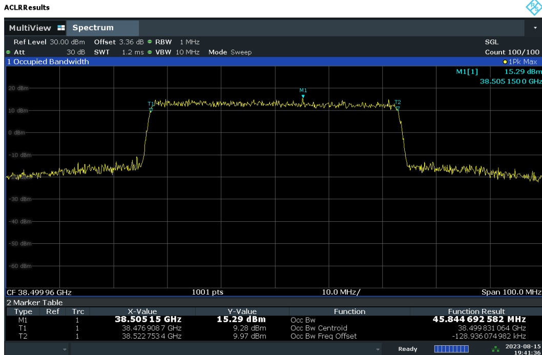
Plot 7-15. Occupied Bandwidth Input at 3dB above AGC Threshold – CP – H-DL Polarization.
