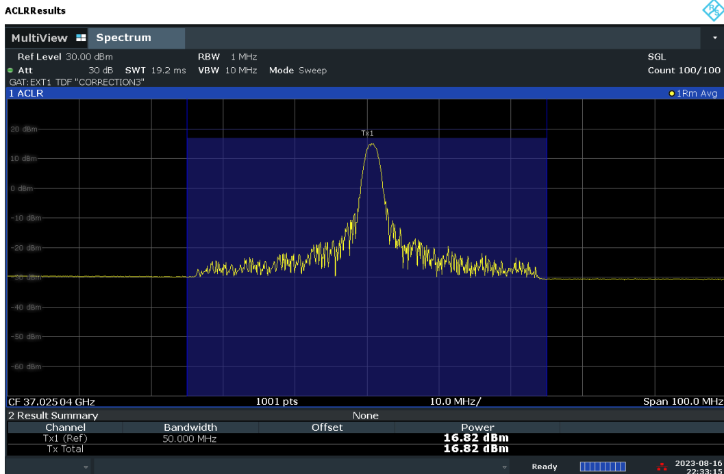
Plot 7-107. Conducted Power Plot – CP – H-DL Polarization (50MHz-1CC – QPSK – Low Ch. – 1RB)
