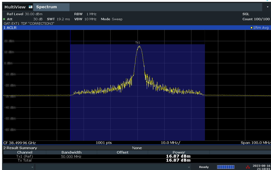
Plot 7-109. Conducted Power Plot – CP – H-DL Polarization (50MHz-1CC – QPSK – Mid Ch. – 1 RB)
