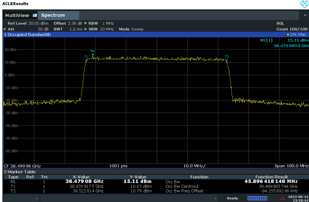
Plot 7-25. Occupied Bandwidth Plot – DFT-s – H-DL Polarization (50MHz-1CC – QPSK – Mid Channel)
