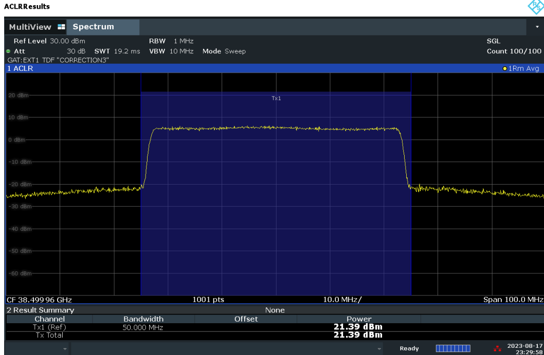
Plot 7-87. Conducted Power Plot – CP – V-DL Polarization (50MHz-1CC – QPSK – Mid Ch. – Full RB)
