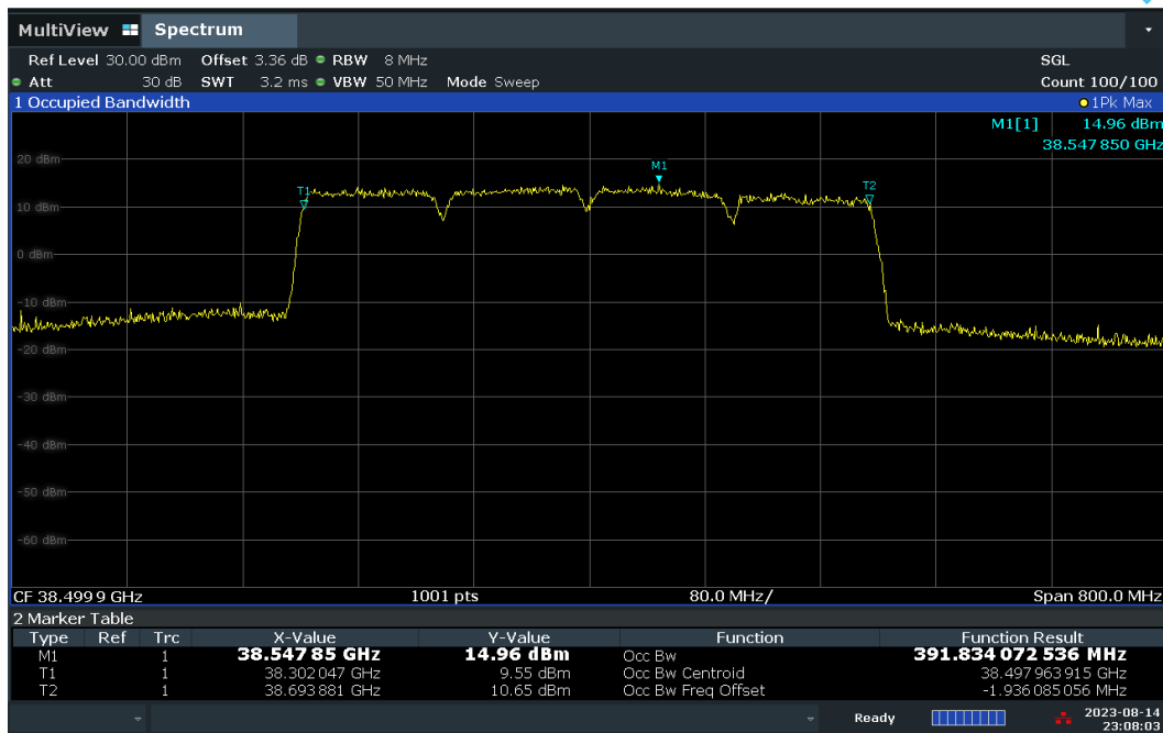
Plot 7-30. Occupied Bandwidth Plot – DFT-s – H-DL Polarization (100MHz-4CC – 16QAM – Mid Channel)
