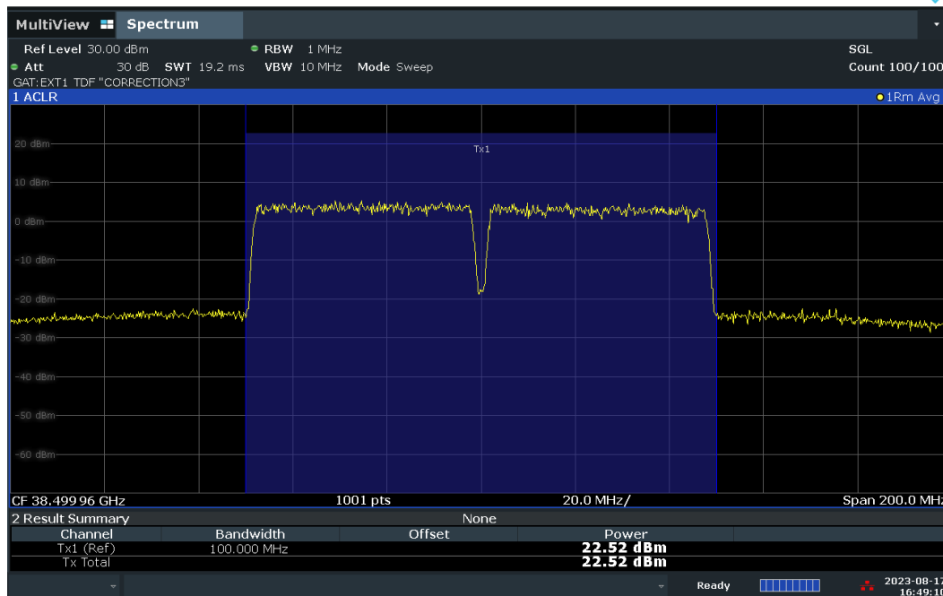
Plot 7-73. Conducted Power Plot – DFT-S – H-DL Polarization (50MHz-2CC – QPSK – Mid Ch. – Full RB)
