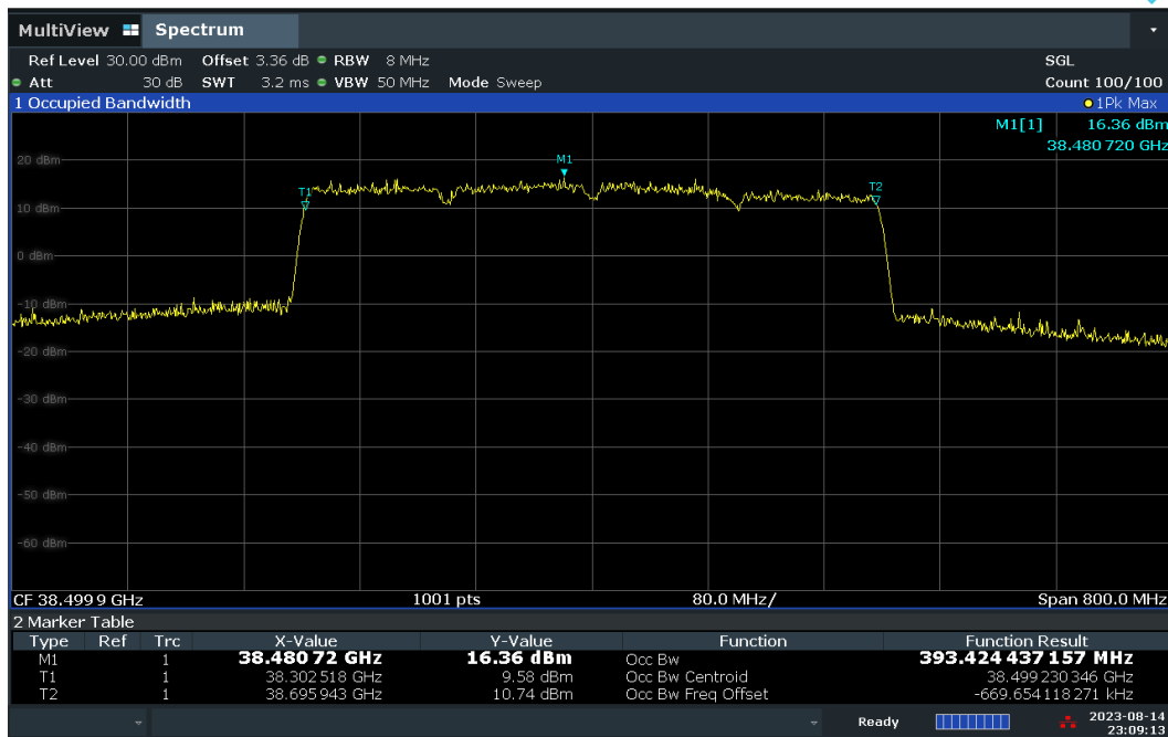
Plot 7-42. Occupied Bandwidth Plot – CP – H-DL Polarization (100MHz-4CC – 16QAM – Mid Channel)
