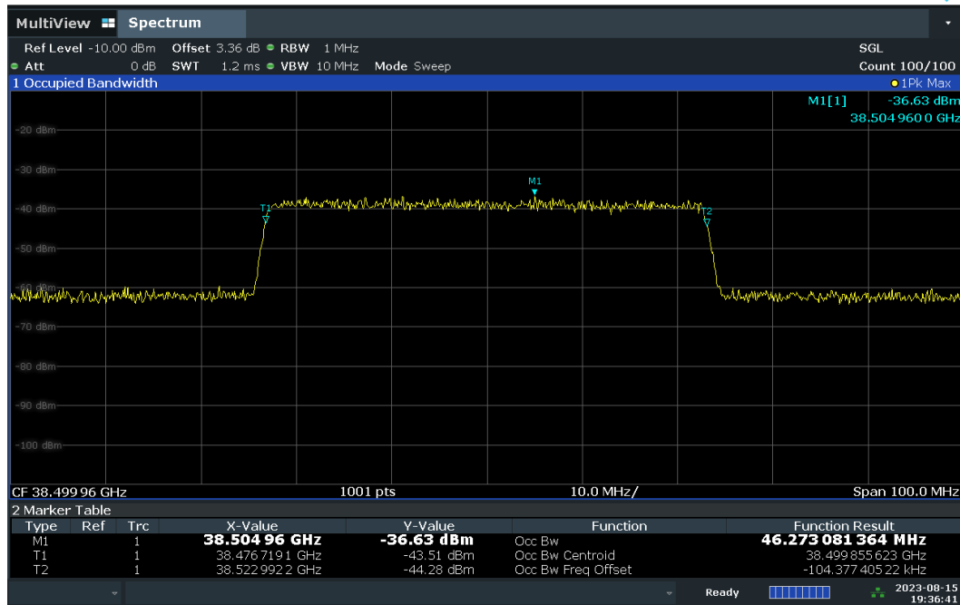
Plot 7-13. Occupied Bandwidth Input at 0.5dB below AGC Threshold – CP – H-DL Polarization.
