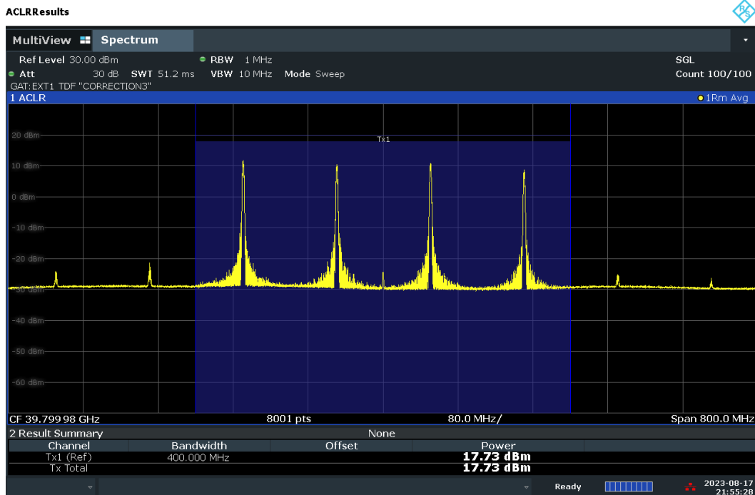
Plot 7-104. Conducted Power Plot – CP – V-DL Polarization (100MHz-4CC – QPSK – High Ch. – 1 RB)
