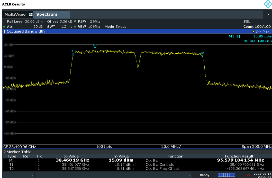
Plot 7-34. Occupied Bandwidth Plot – CP – V-DL Polarization (50MHz-2CC – 16QAM – Mid Channel)
