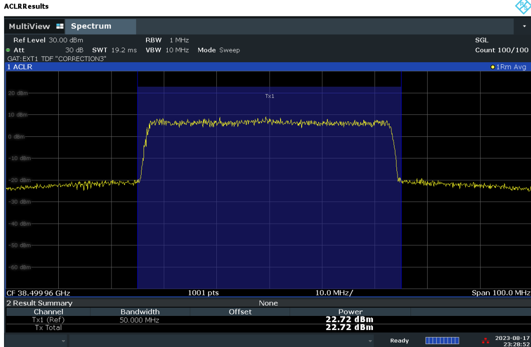
Plot 7-49. Conducted Power Plot – DFT-S – V-DL Polarization (50MHz-1CC – 16QAM – Mid Ch. – Full RB)
