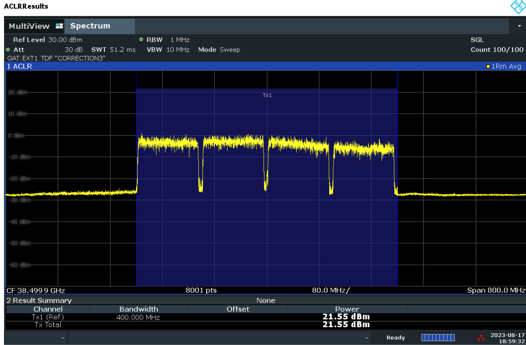
Plot 7-80. Conducted Power Plot – DFT-S – H-DL Polarization (100MHz-4CC – QPSK – Mid Ch. – Full RB)
