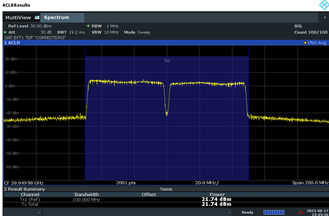
Plot 7-96. Conducted Power Plot – CP – V-DL Polarization (50MHz-2CC – QPSK – High Ch. – Full RB)
