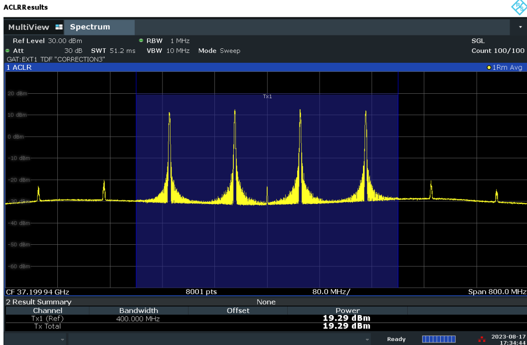
Plot 7-79. Conducted Power Plot – DFT-S – H-DL Polarization (100MHz-4CC – QPSK – Low Ch. – 1RB)
