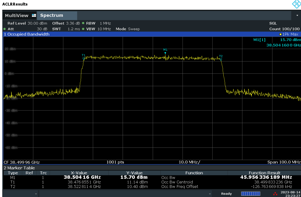
Plot 7-38. Occupied Bandwidth Plot – CP – H-DL Polarization (50MHz-1CC – 16QAM – Mid Channel)
