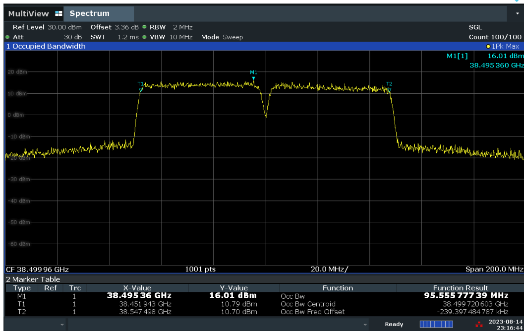
Plot 7-40. Occupied Bandwidth Plot – CP – H-DL Polarization (50MHz-2CC – 16QAM – Mid Channel)
