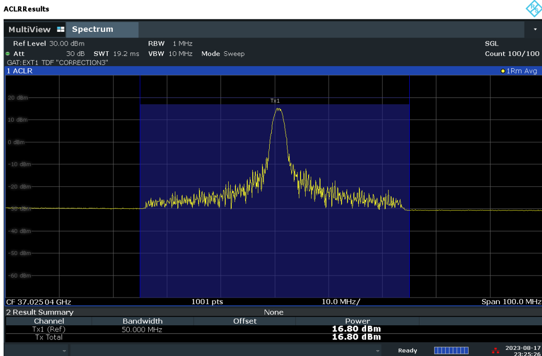
Plot 7-86. Conducted Power Plot – CP – V-DL Polarization (50MHz-1CC – QPSK – Low Ch. – 1RB)
