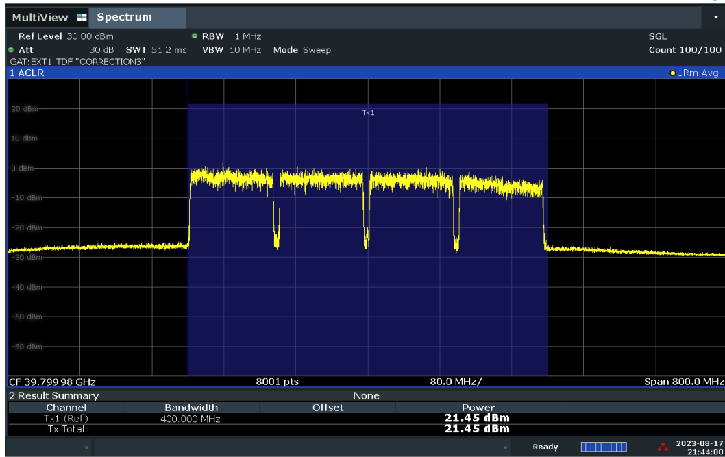
Plot 7-63. Conducted Power Plot – DFT-S – V-DL Polarization (100MHz-4CC – 16QAM – High Ch. – Full RB)
