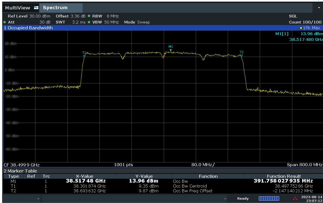
Plot 7-29. Occupied Bandwidth Plot – DFT-s – H-DL Polarization (100MHz-4CC – QPSK – Mid Channel)
