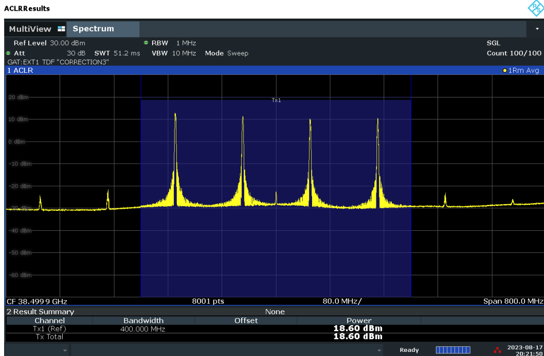
Plot 7-60. Conducted Power Plot – DFT-S – V-DL Polarization (100MHz-4CC – QPSK – Mid Ch. – 1 RB)
