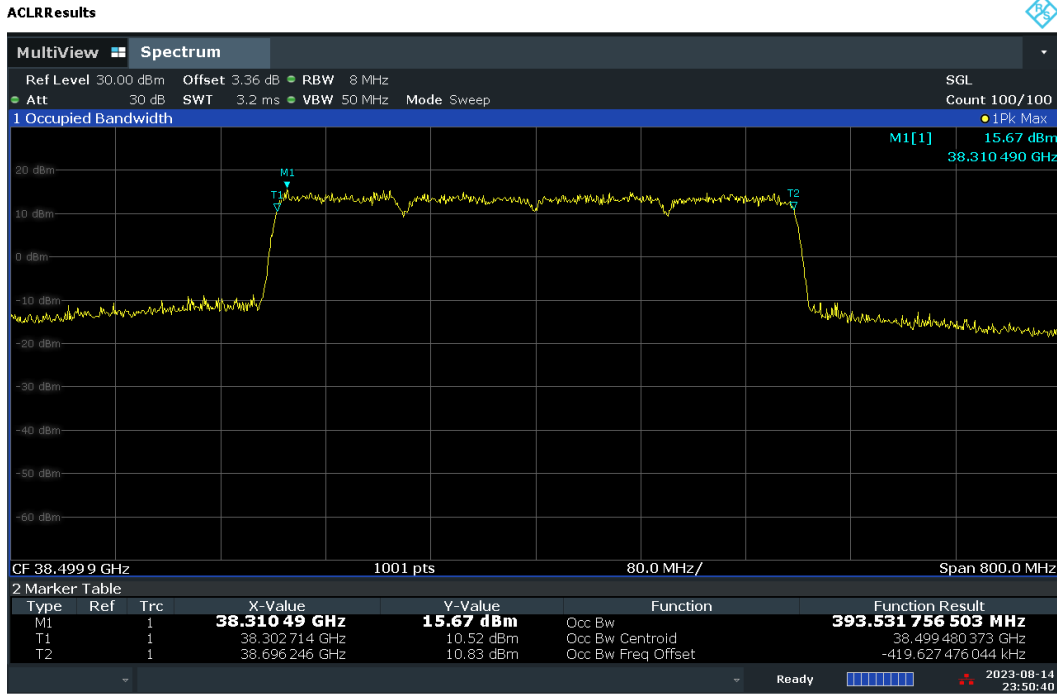
Plot 7-35. Occupied Bandwidth Plot – CP – V-DL Polarization (100MHz-4CC – QPSK – Mid Channel)
