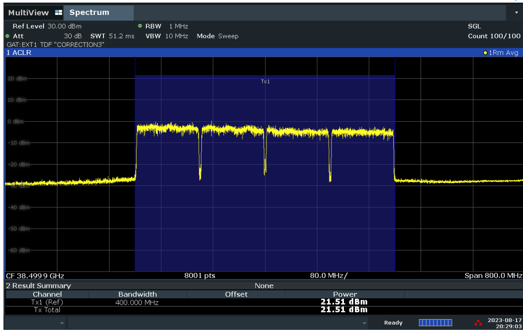
Plot 7-101. Conducted Power Plot – CP – V-DL Polarization (100MHz-4CC – QPSK – Mid Ch. – Full RB)
