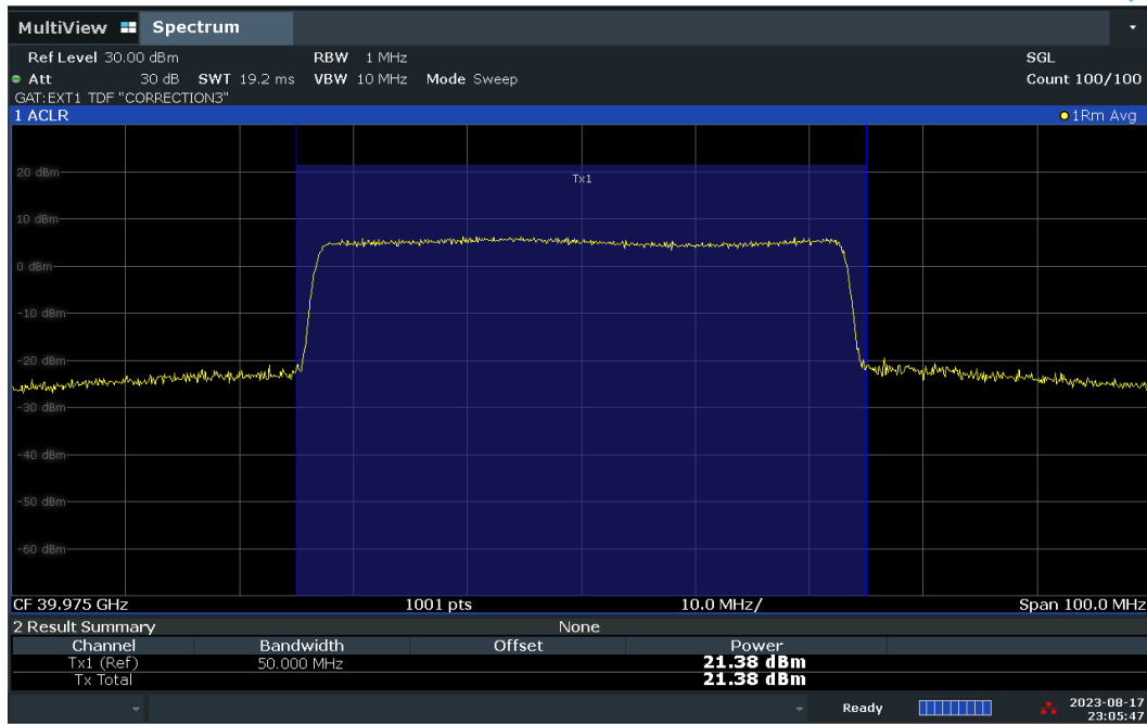
Plot 7-89. Conducted Power Plot – CP – V-DL Polarization (50MHz-1CC – QPSK – High Ch. – Full RB)
