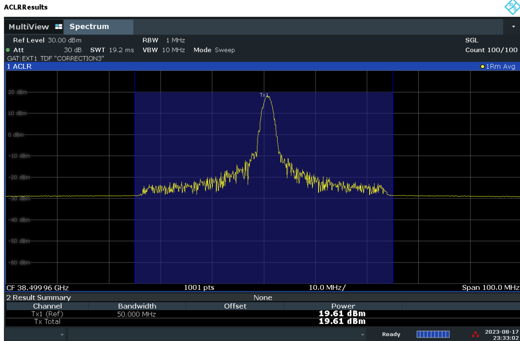
Plot 7-46. Conducted Power Plot – DFT-S – V-DL Polarization (50MHz-1CC – QPSK – Mid Ch. – 1 RB)
