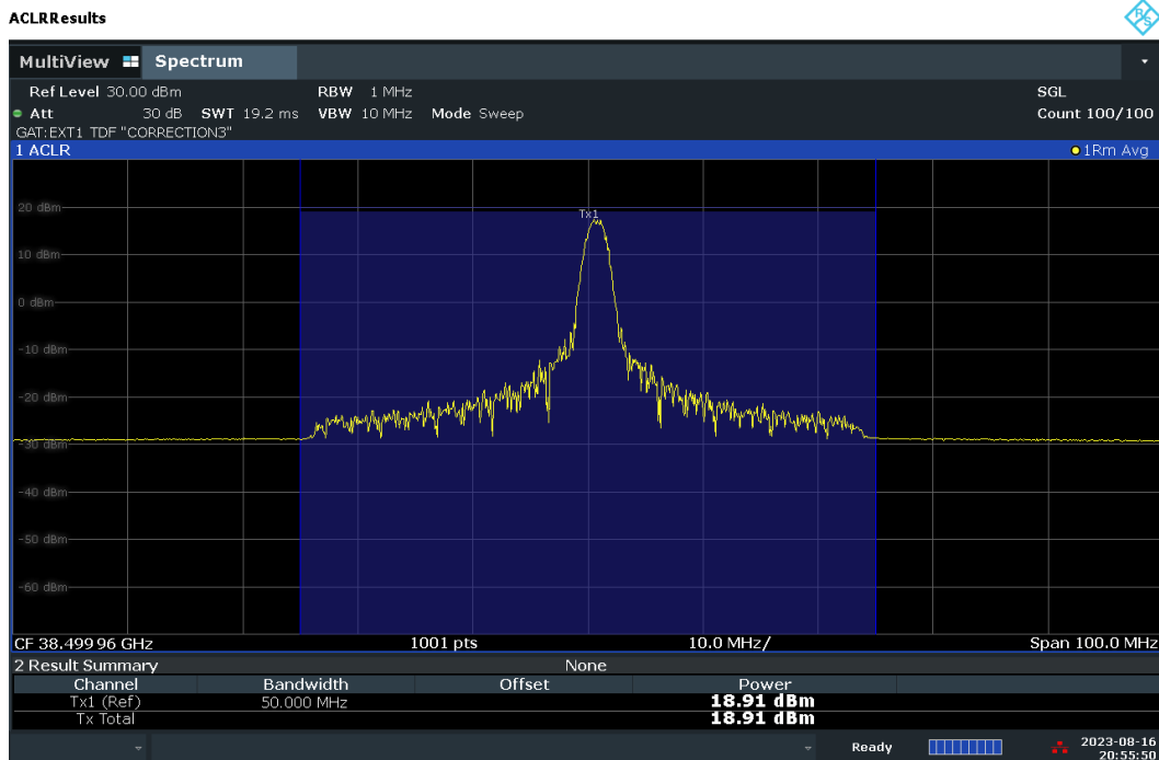
Plot 7-67. Conducted Power Plot – DFT-S – H-DL Polarization (50MHz-1CC – QPSK – Mid Ch. – 1 RB)
