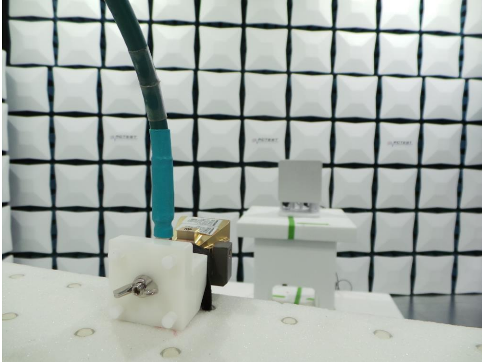
Setup 5. Test Setup 18-40GHz - SU
