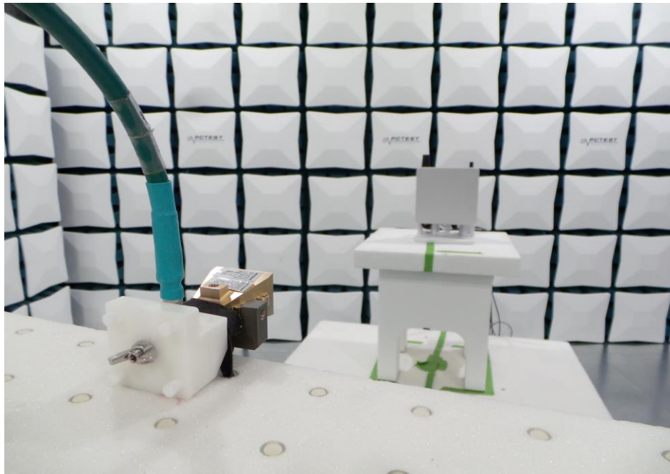
Setup 5. Test Setup 18-40GHz - DU
