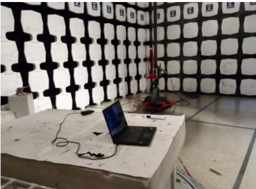
Radiated Emission:
