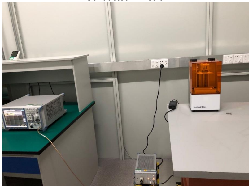
Conducted Emission
