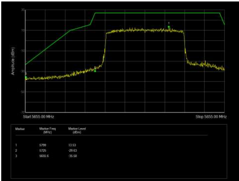
Band Edge NVNT 802.11n(HT20) 5745MHz Low Ant 0
