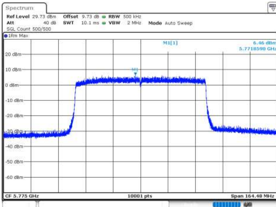
PSD NVNT 802.11ax80 5775MHz Ant 3
