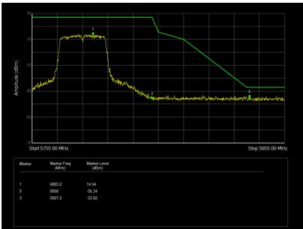
Band Edge NVNT 802.11ac80 5775MHz High Ant 0
