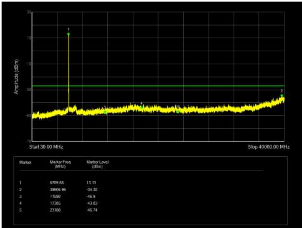
Tx. Spurious NVNT 802.11n(HT40) 5755MHz Ant 3 Emission
