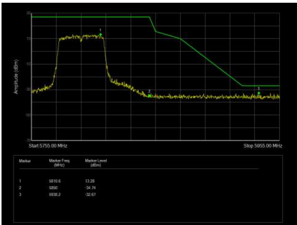
Band Edge NVNT 802.11ac40 5755MHz Low Ant 3
