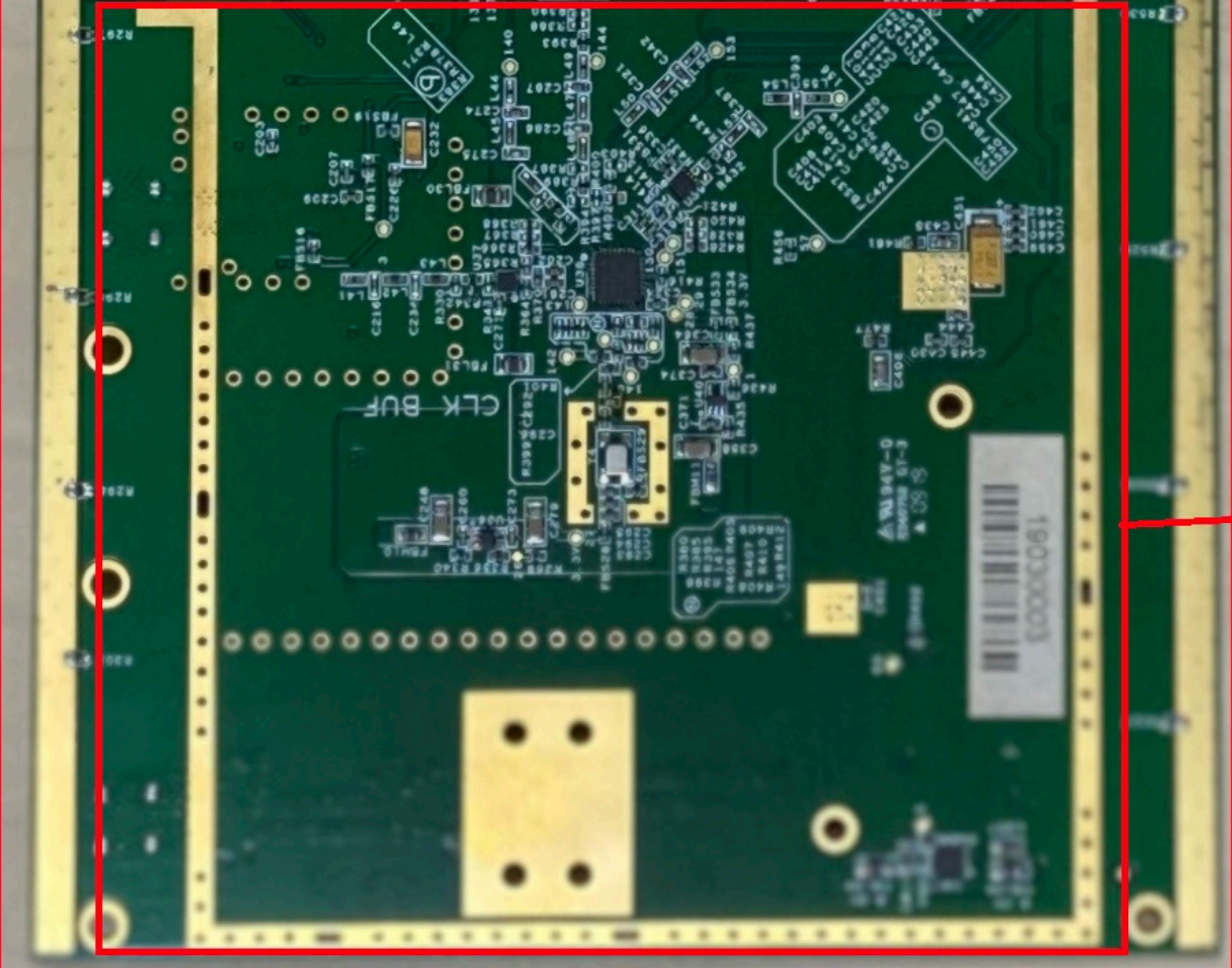
small signal RF section (back)
