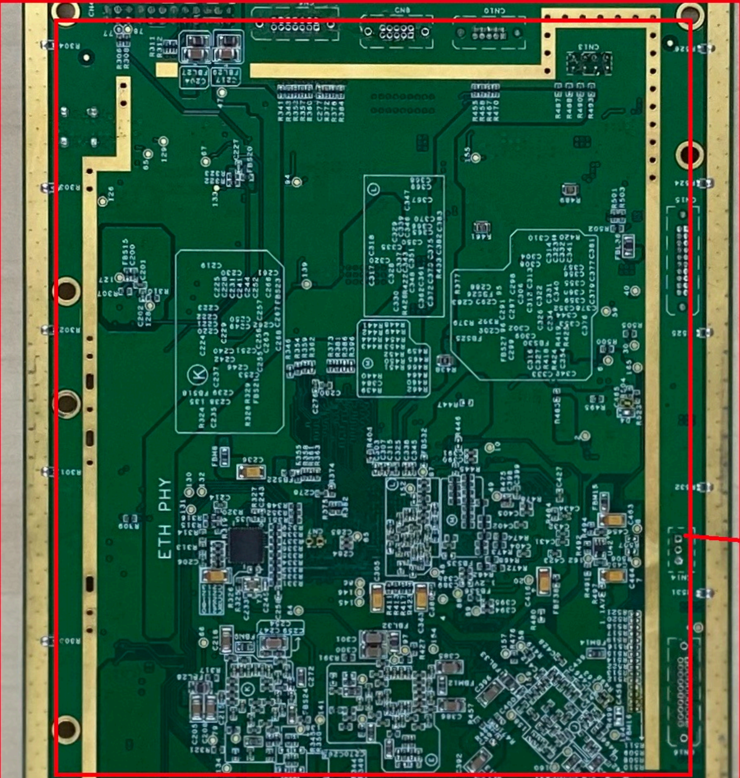
Digital + small signal board (back)
