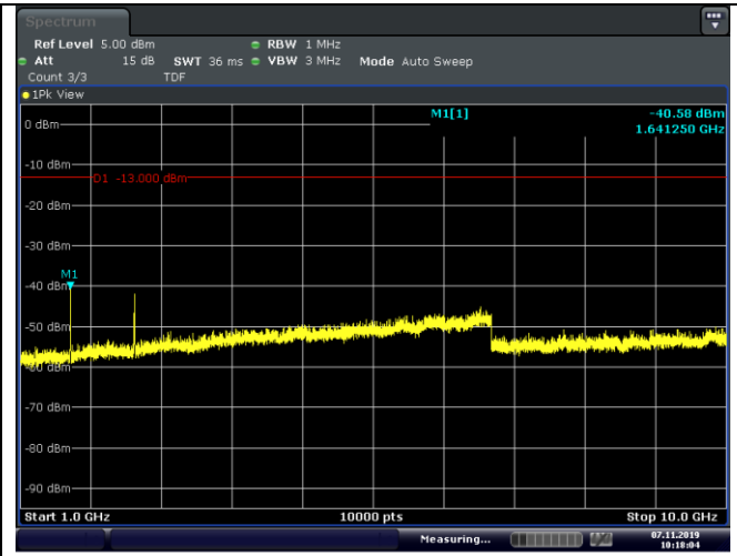
1GHz~10GHz
