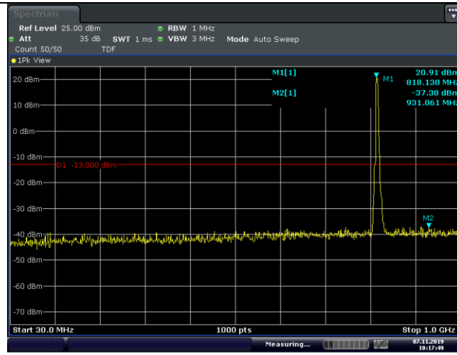
30MHz~1GHz
