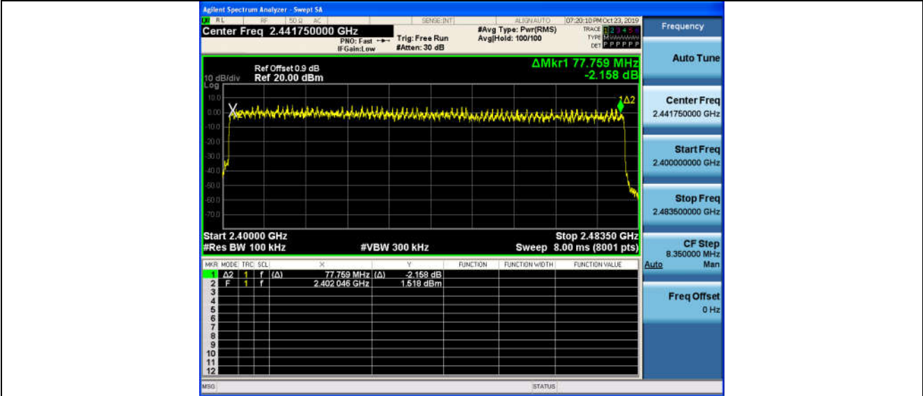
π/4DQPSK Modulation
