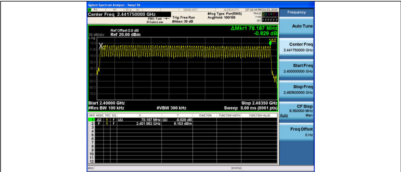
GFSK Modulation
