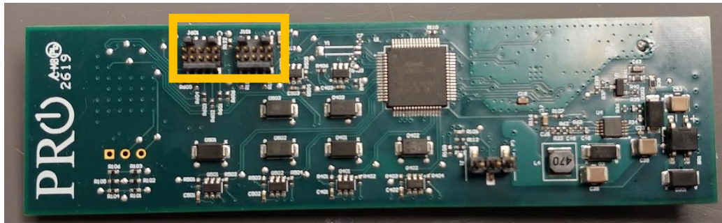
Pbase Top and Bottom PCBA (Note, Outlined parts to be DNI for chamber testing and production)
