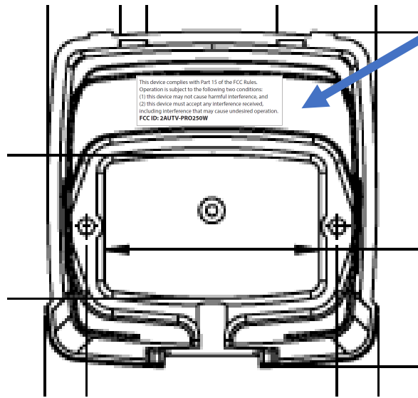
Interior view of rear product housing
