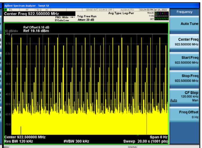
922.5 MHz - Number of pulses in 20 s
