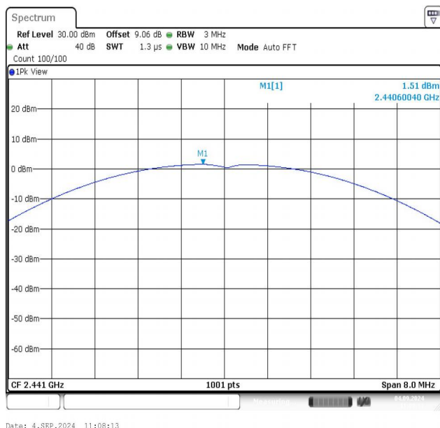
2DH5-Ant1-2441-PASS
