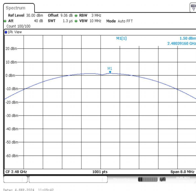
2DH5-Ant1-2480-PASS
