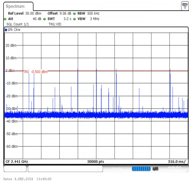
2DH3-Ant1-Hop-PASS
