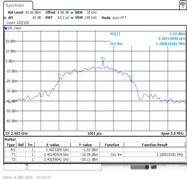
2DH5-Ant1-2402
