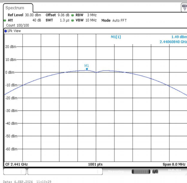
3DH5-Ant1-2441-PASS
