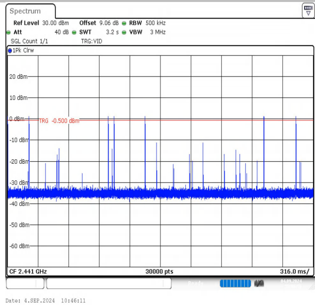
2DH5-Ant1-Hop-PASS
