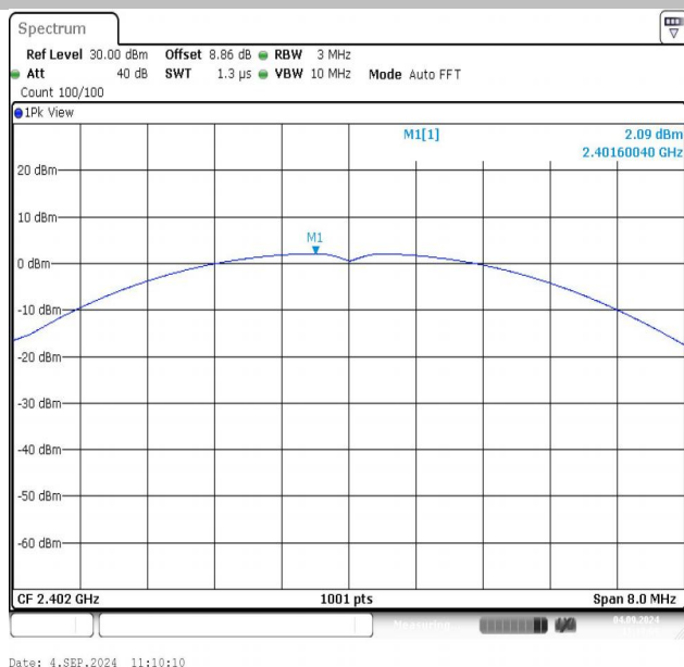
3DH5-Ant1-2402-PASS
