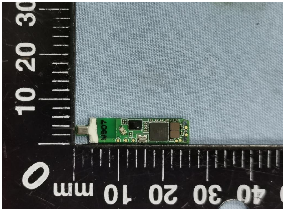
Solder Board-Component View 10
