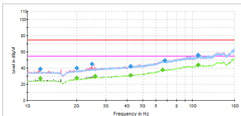
Radiated Emission from 1GHz to 18GHz
