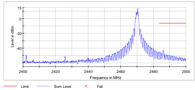
Figure 7.5.1.2-5: Upper Band-edge – Channel 24
