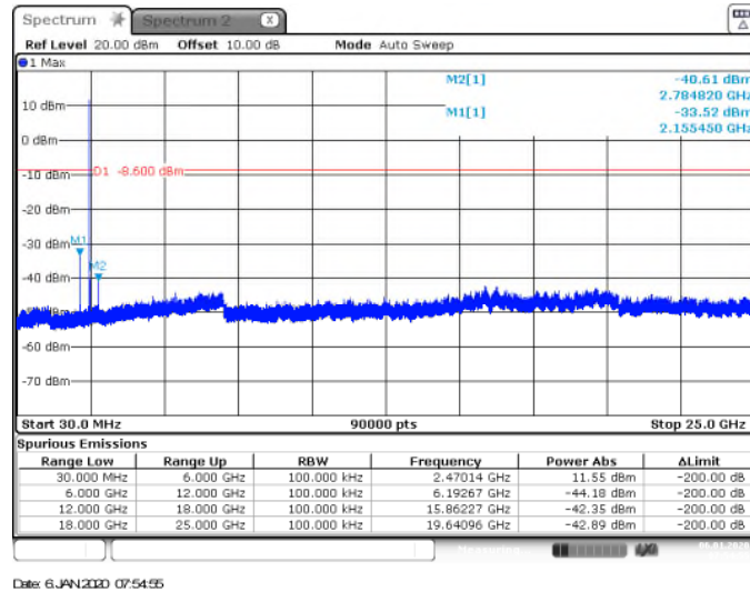
Figure 7.5.1.2-3: HCH – 30MHz–25GHz
