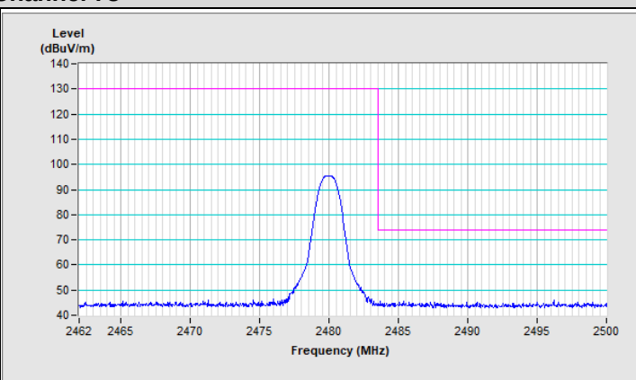
BT GFSK Channel 78
