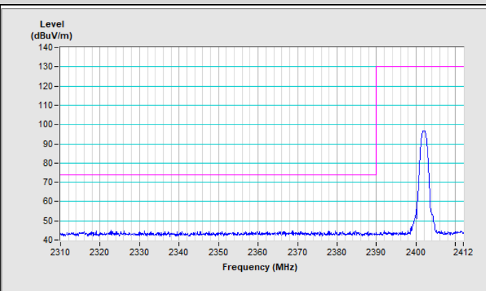
BT GFSK Channel 0
