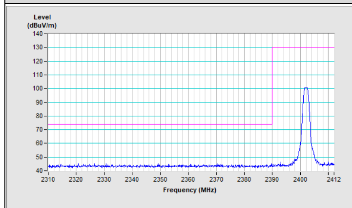
Horizontal (Peak)
