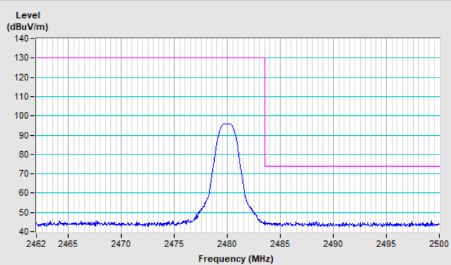
Vertical (Peak)
