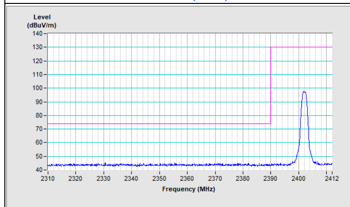
Vertical (Peak)
