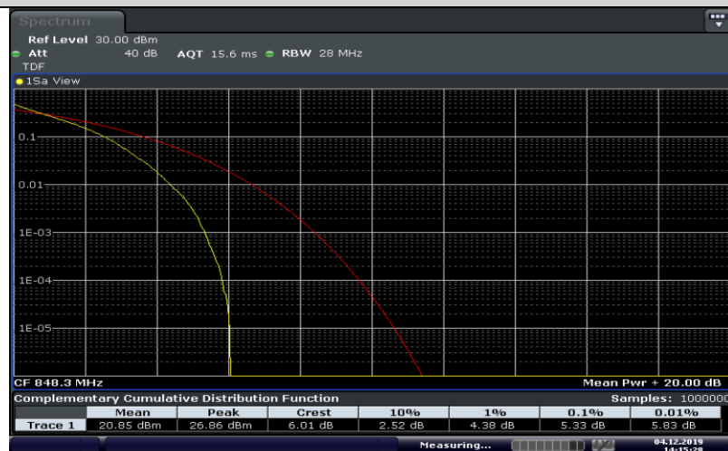
Band5-1.4MHz-QPSK-20643-6RB#0
