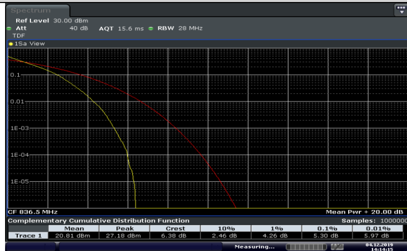
Band5-1.4MHz-QPSK-20525-6RB#0
