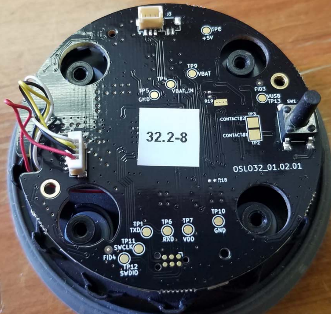
Top View of the PCB for the EUT - View #2
