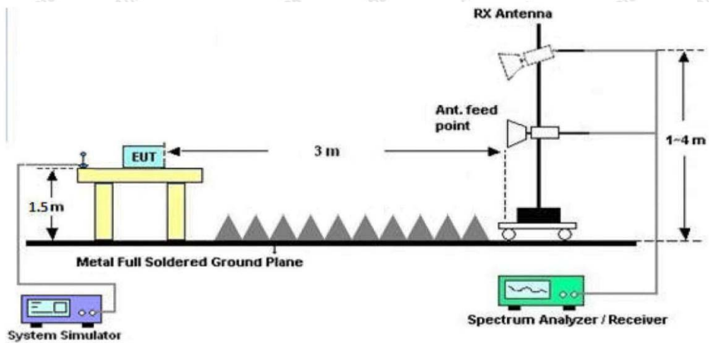
Figure 3. Above 1 GHz
